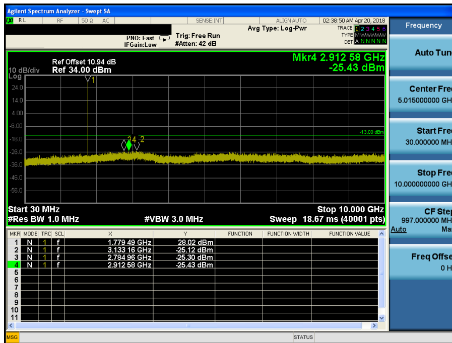
LTE Band 66 / 1.4MHz / 16QAM - RB Size/Offset (1/2) – High Channel
