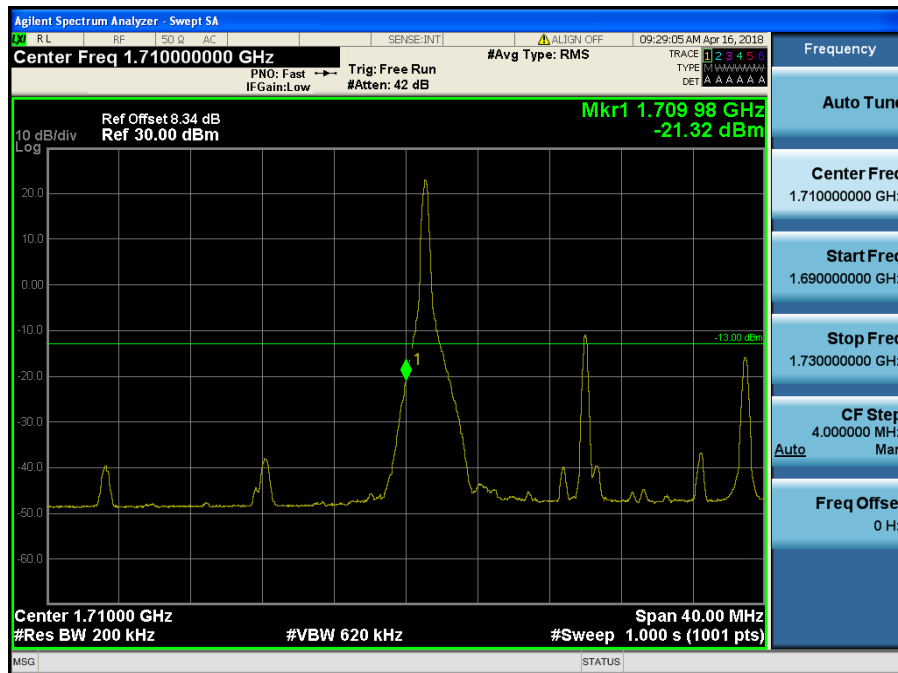
LTE Band 66 / 20MHz / QPSK - RB Size/Offset (1/0)
