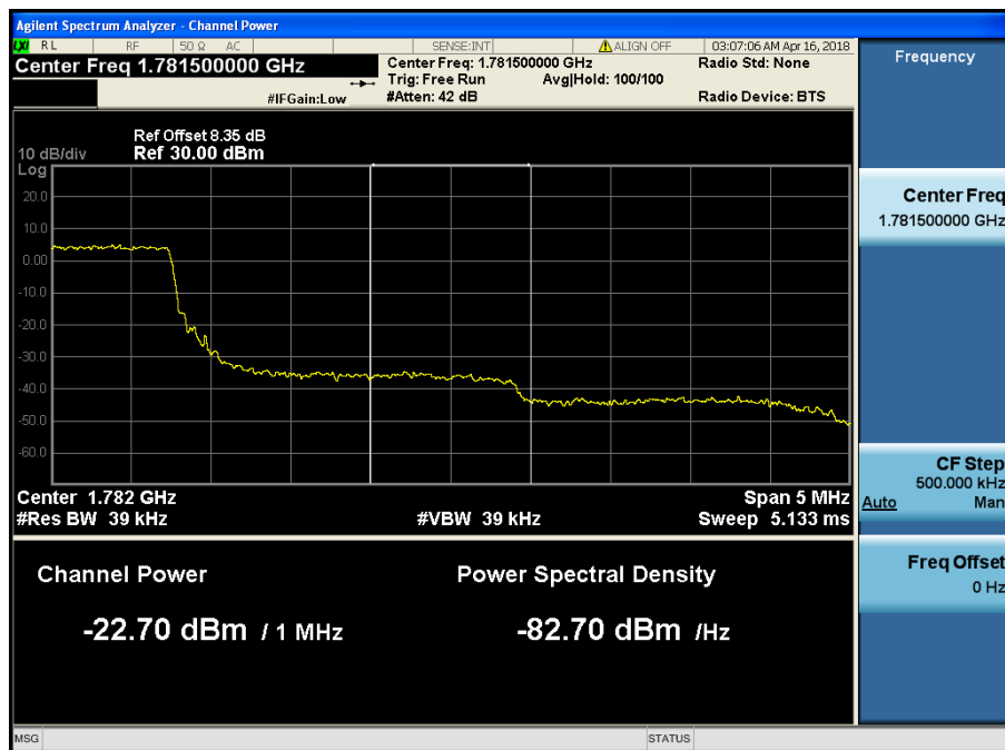
LTE Band 66 / 5MHz / QPSK - RB Size/Offset (12/13)
