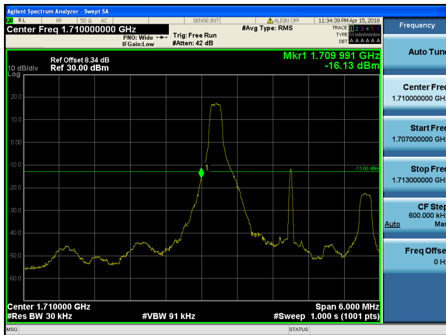
LTE Band 66 / 3MHz / QPSK - RB Size/Offset (1/0)
