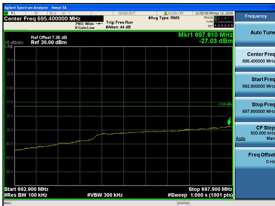
LTE Band 12 / 5MHz / QPSK Offset/Size (25/0)
