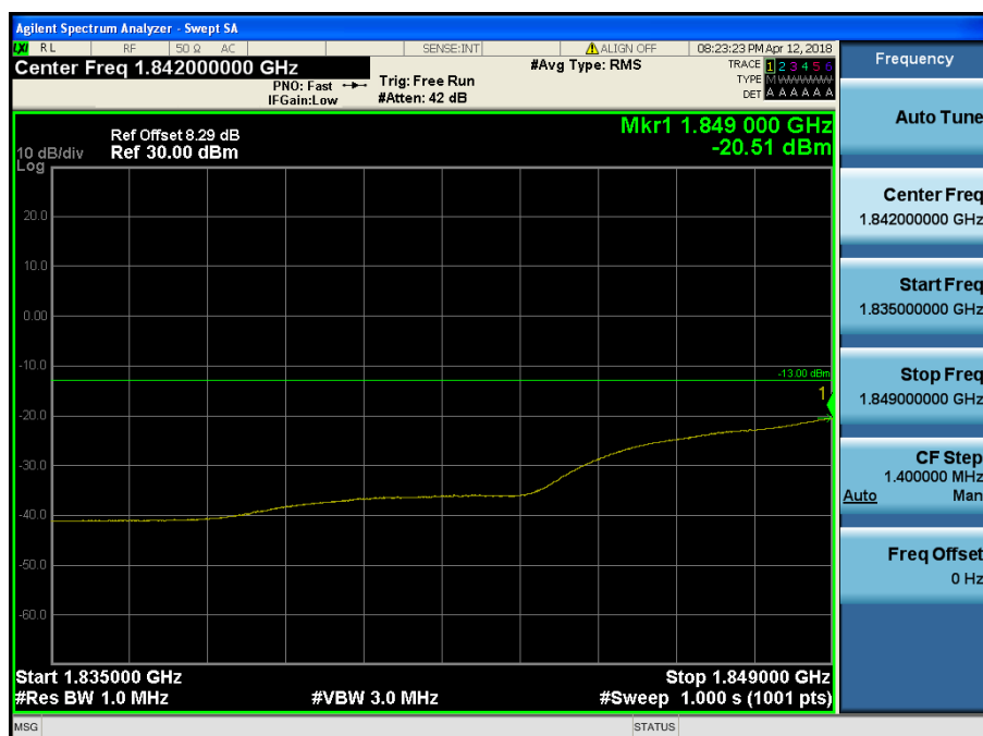
LTE Band 2 / 15MHz / QPSK - RB Size/Offset (36/0)
