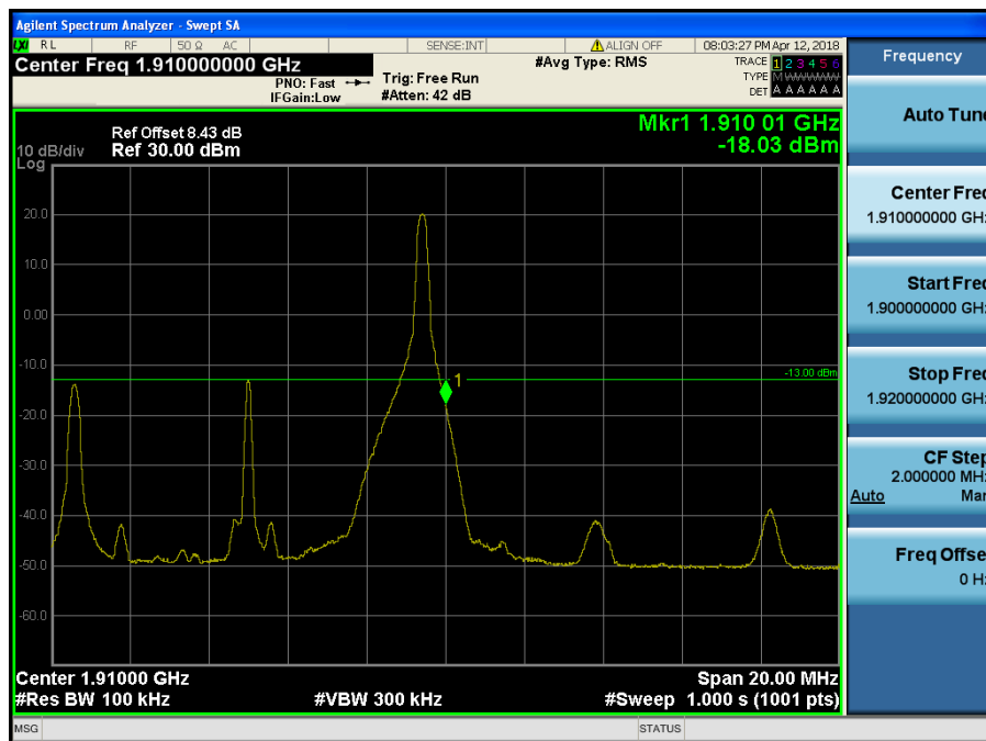
LTE Band 2 / 10MHz / QPSK - RB Size/Offset (1/49)
