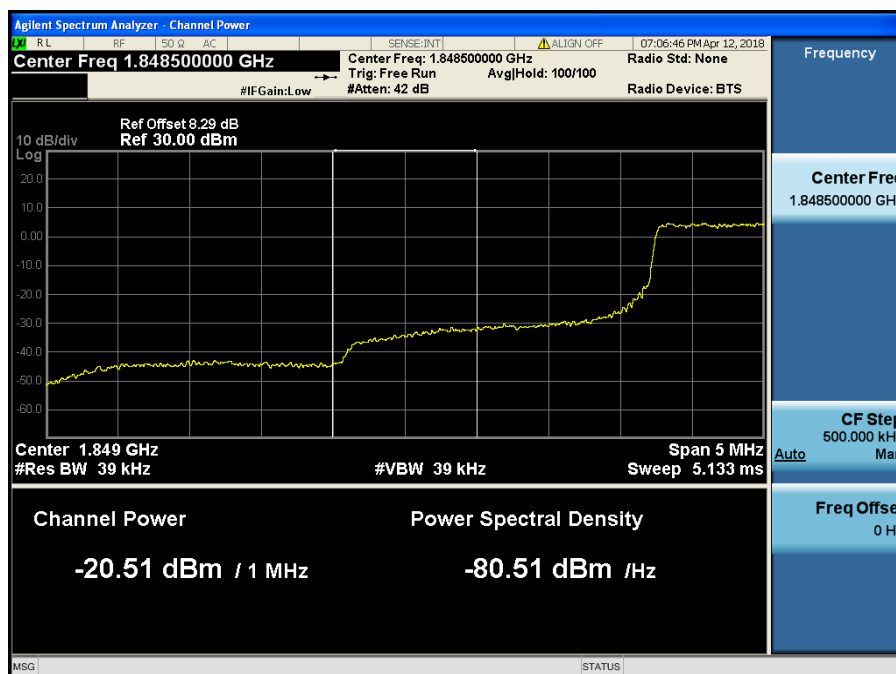
LTE Band 2 / 5MHz / QPSK Offset/Size (12/0)
