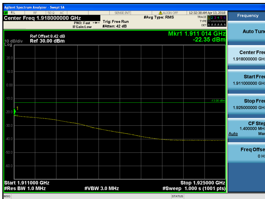
LTE Band 2 / 15MHz / 16QAM - RB Size/Offset (36/39)
