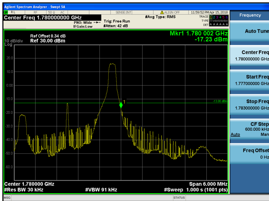
LTE Band 66 / 3MHz / QPSK - RB Size/Offset (1/14)
