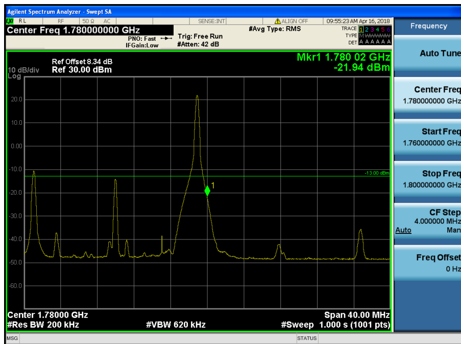
LTE Band 66 / 20MHz / QPSK - RB Size/Offset (1/99)
