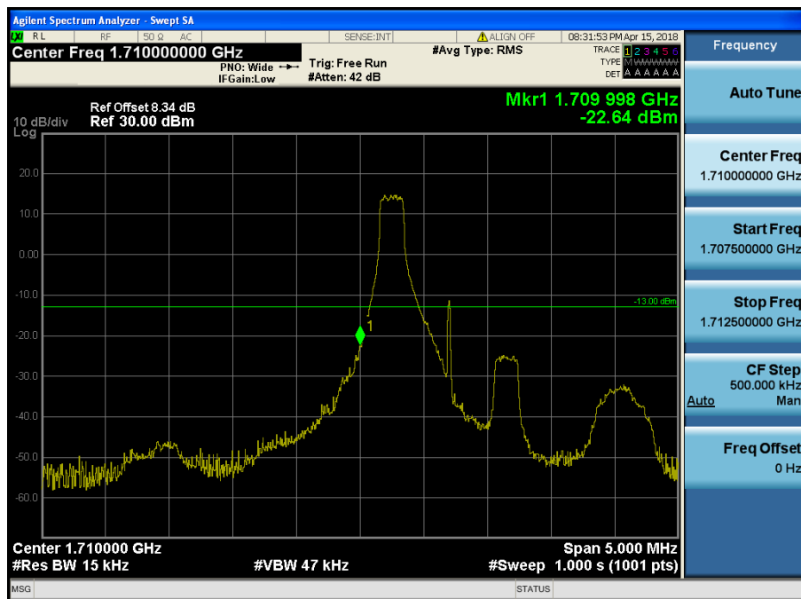
LTE Band 66 / 1.4MHz / QPSK - RB Size/Offset (1/0)
