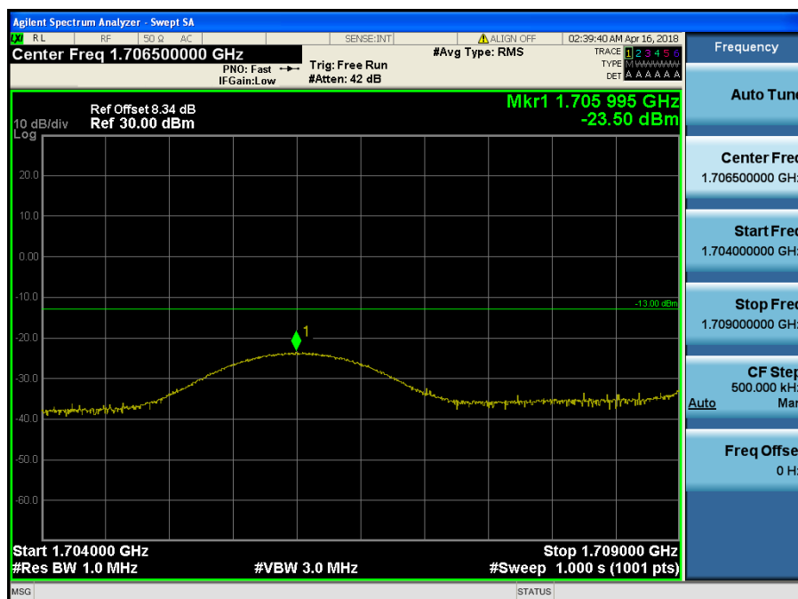
LTE Band 66 / 5MHz / QPSK Offset/Size (1/24)
