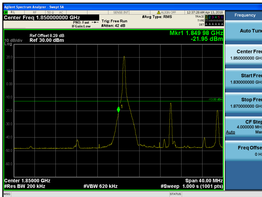
LTE Band 2 / 20MHz / 16QAM - RB Size/Offset (1/0)
