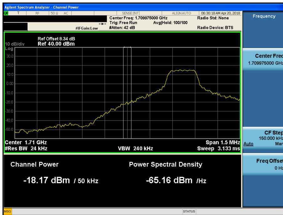
LTE Band 66 / 5MHz / QPSK Offset/Size (1/0)
