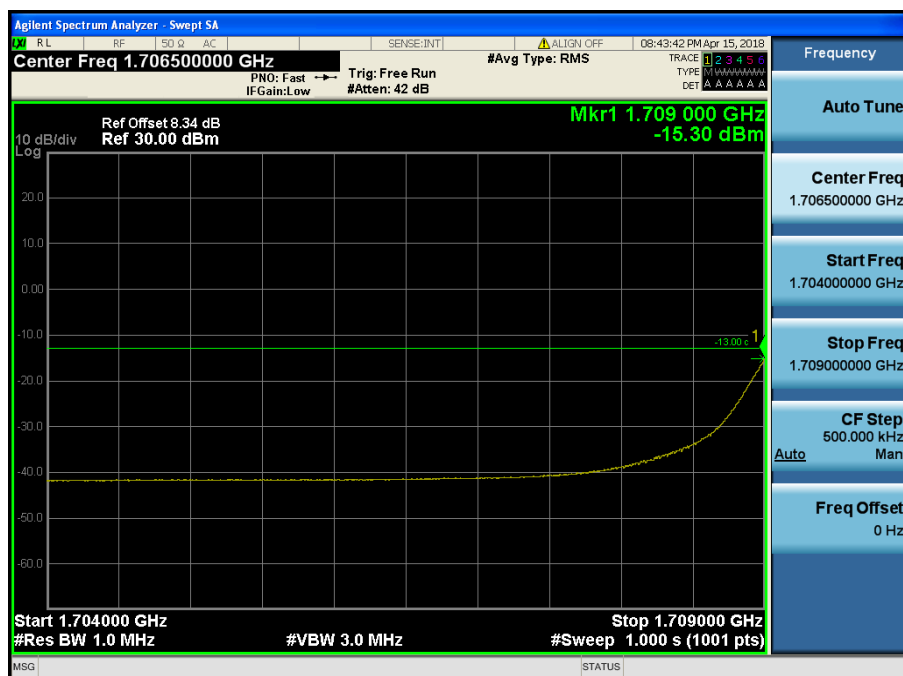
LTE Band 66 / 1.4MHz / QPSK - RB Size/Offset (3/2)
