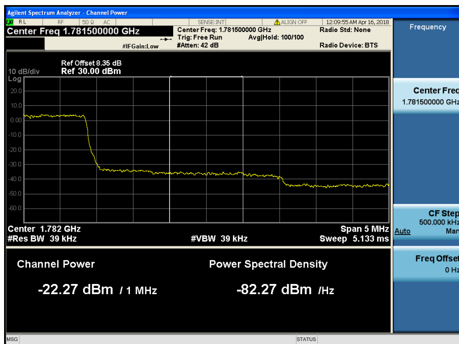
LTE Band 66 / 3MHz / QPSK - RB Size/Offset (15/0)
