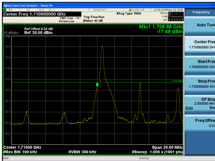
LTE Band 66 / 10MHz / 16QAM - RB Size/Offset (1/0)
