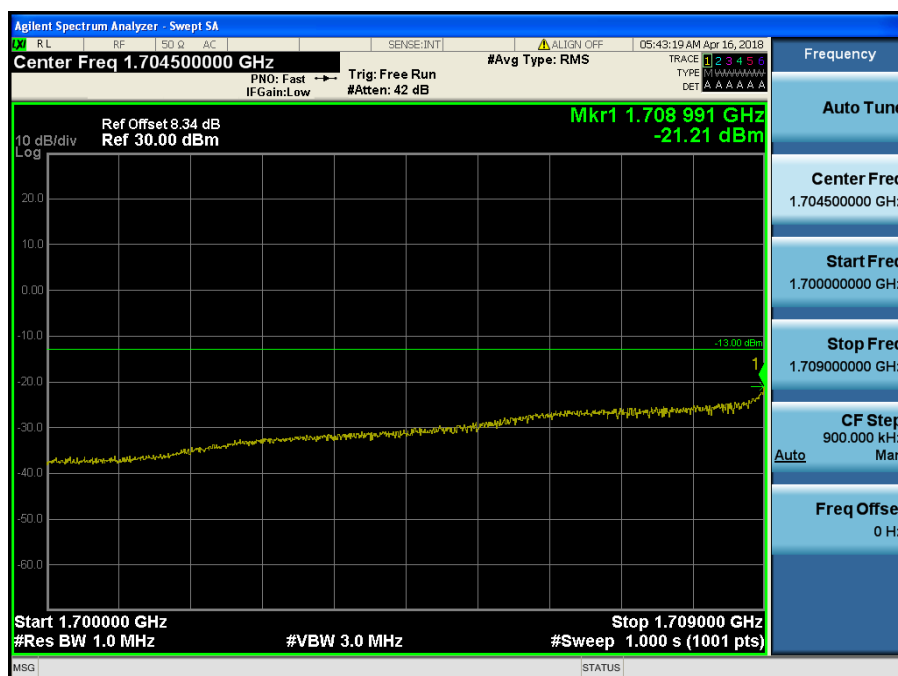
LTE Band 66 / 10MHz / QPSK - RB Size/Offset (25/0)
