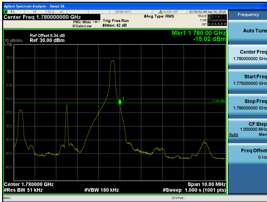
LTE Band 66 / 5MHz / QPSK - RB Size/Offset (1/24)
