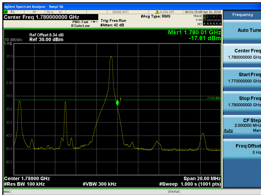
LTE Band 66 / 10MHz / QPSK - RB Size/Offset (1/49)
