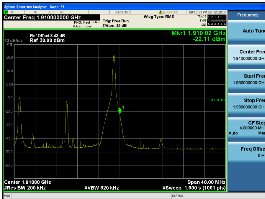
LTE Band 2 / 20MHz / QPSK - RB Size/Offset (1/99)
