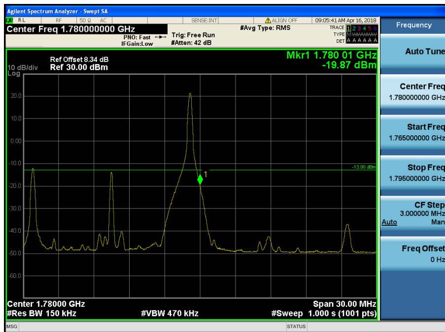
LTE Band 66 / 15MHz / QPSK - RB Size/Offset (1/74)
