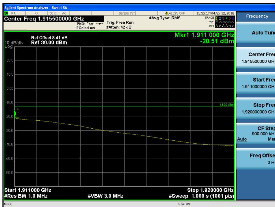
LTE Band 2 / 10MHz / 16QAM - RB Size/Offset (25/25)
