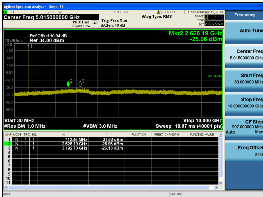
LTE Band 17 / 5MHz / QPSK - RB Size/Offset (1/24)–Mid Channel
