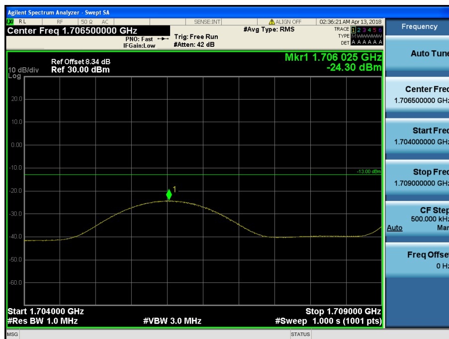
LTE Band 4 / 5MHz / QPSK Offset/Size (1/24)
