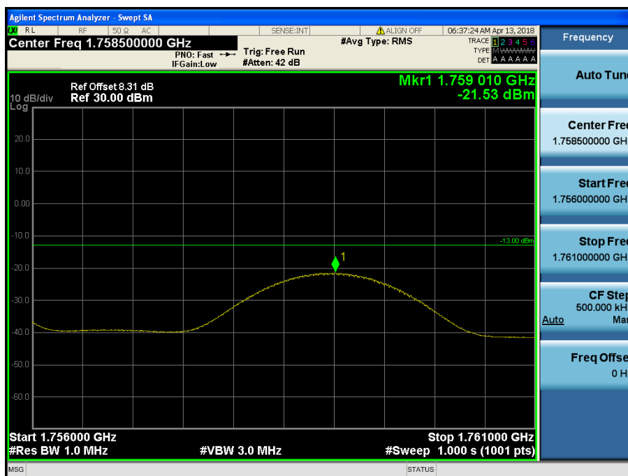
LTE Band 4 / 5MHz / 16QAM - RB Size/Offset (1/0)
