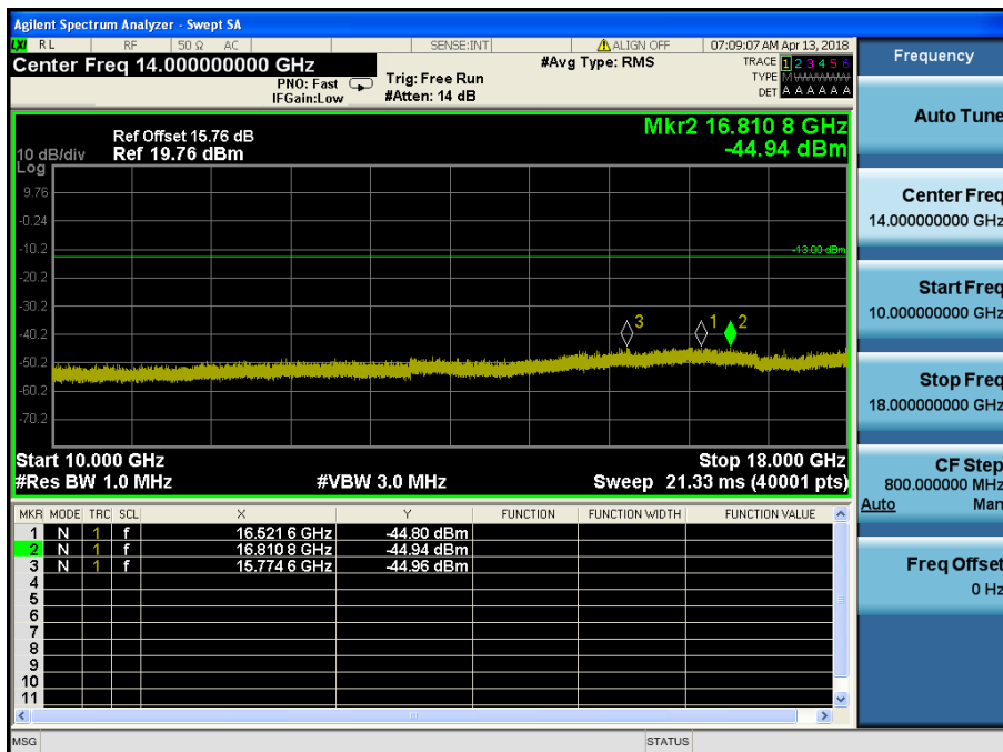
LTE Band 4 / 10MHz / 16QAM - RB Size/Offset (1/25) – Mid Channel
