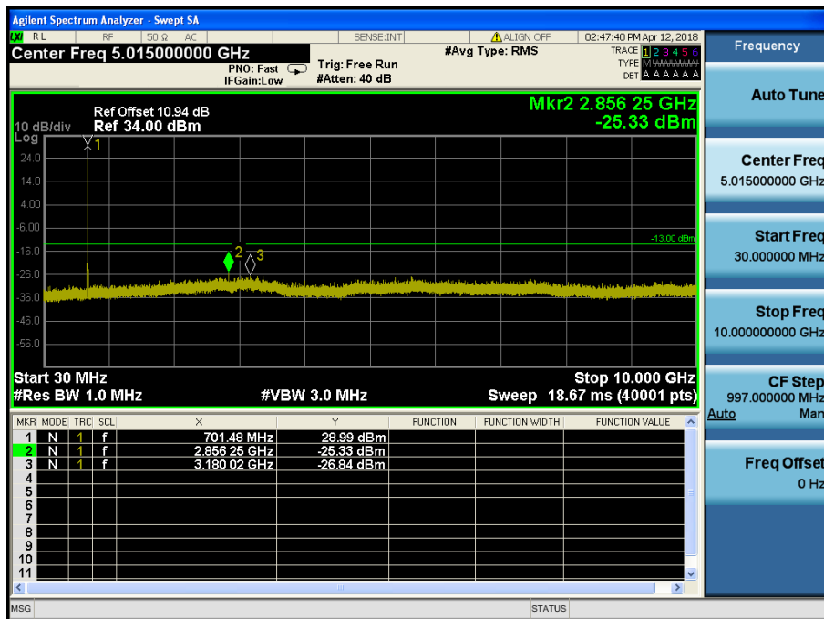
LTE Band 12 / 5MHz / 16QAM - RB Size/Offset (12/6) – Low Channel
