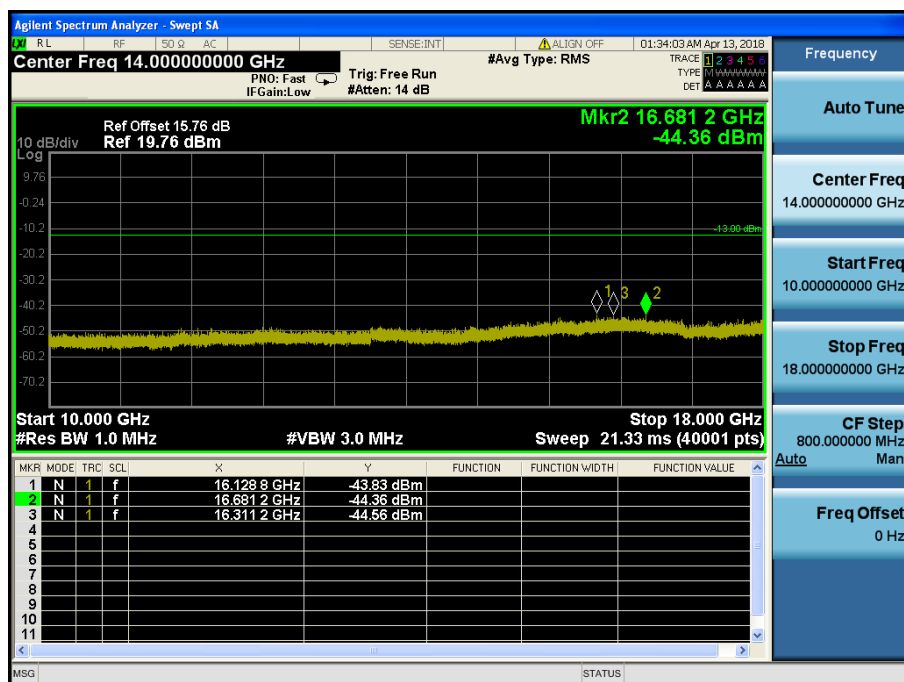
LTE Band 4 / 1.4MHz / QPSK - RB Size/Offset (3/2) – Mid Channel
