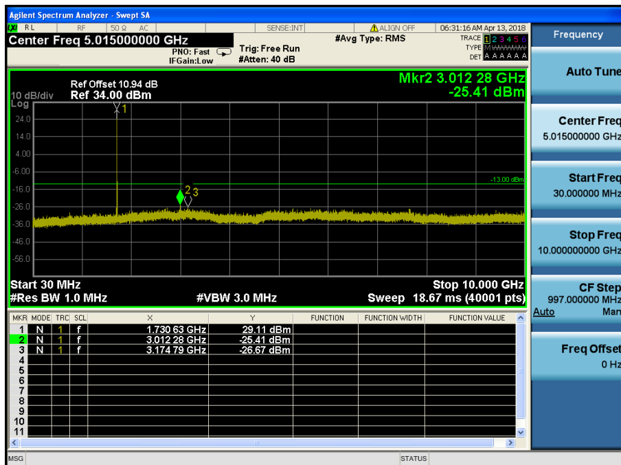
LTE Band 4 / 5MHz / 16QAM - RB Size/Offset (1/0) – Mid Channel
