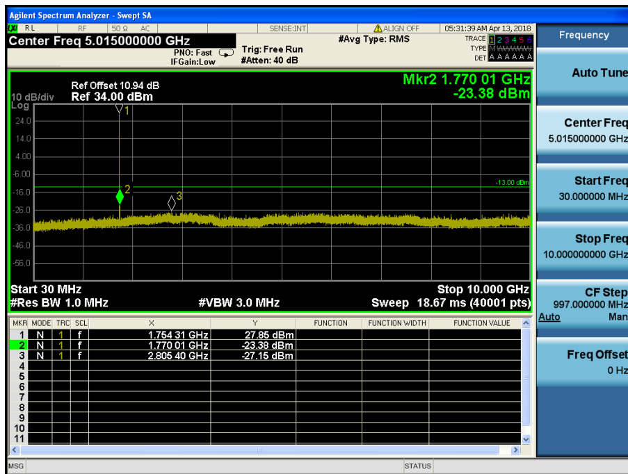
LTE Band 4 / 1.4MHz / 16QAM - RB Size/Offset (3/2) – High Channel
