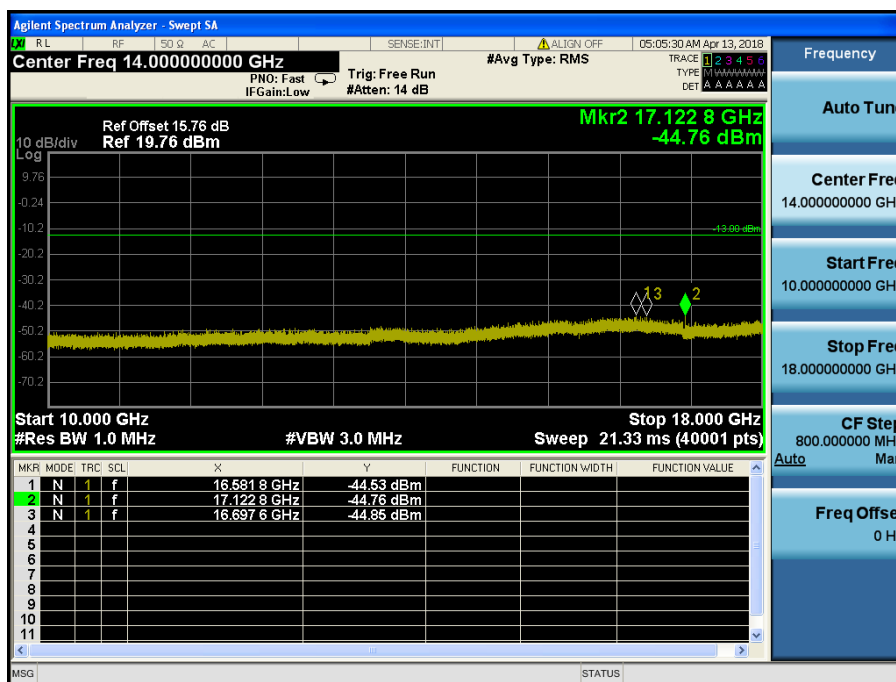
LTE Band 4 / 1.4MHz / 16QAM - RB Size/Offset (1/5) – Low Channel
