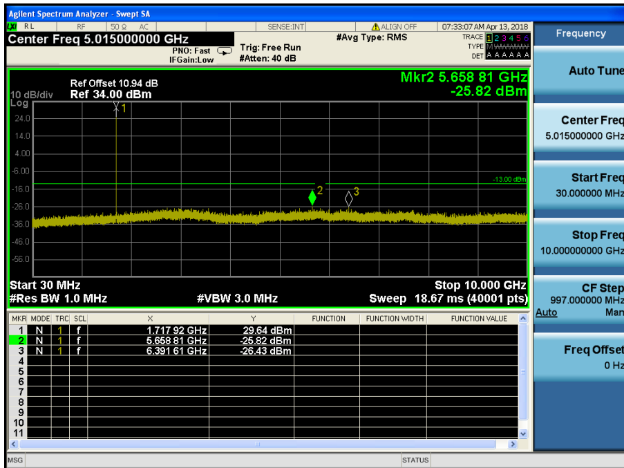
LTE Band 4 / 15MHz / 16QAM - RB Size/Offset (1/36)–Low Channel
