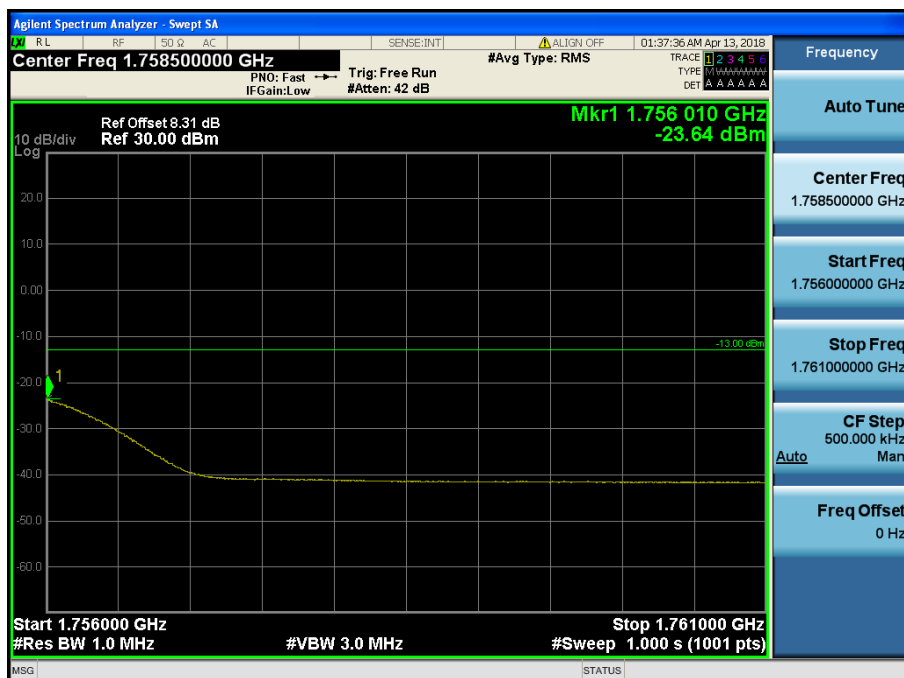
LTE Band 4 / 1.4MHz / QPSK - RB Size/Offset (1/0)
