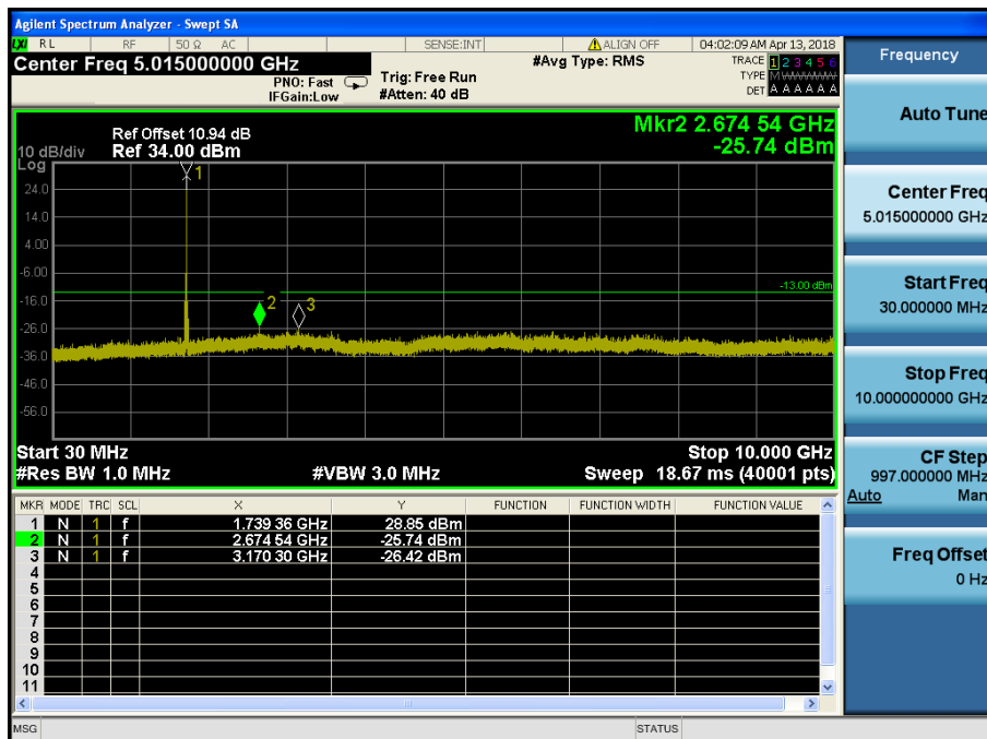
LTE Band 4 / 15MHz / QPSK - RB Size/Offset (1/74) – Mid Channel
