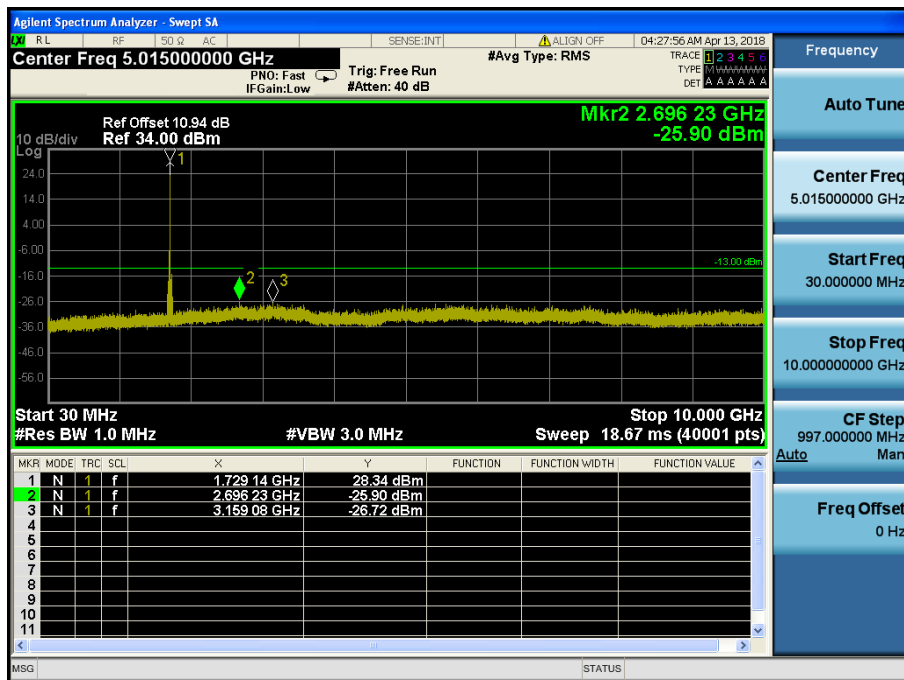
LTE Band 4 / 20MHz / QPSK - RB Size/Offset (1/99) –Low Channel
