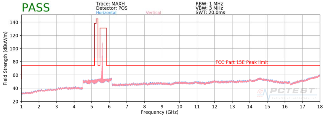
Plot 7-79. Radiated Spurious Plot above 1GHz (802.11a – U2C Ch. 120, Ant. Pol. H)
