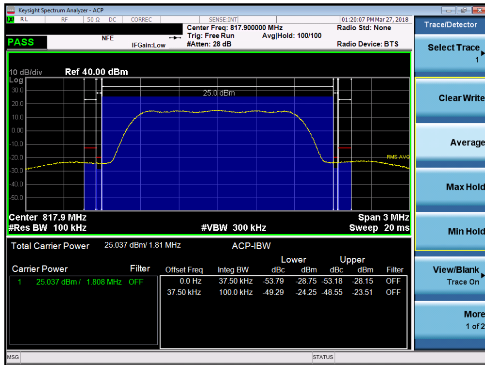
Plot 7-25. Channel Edge Plot (CDMA - Ch. 476)
