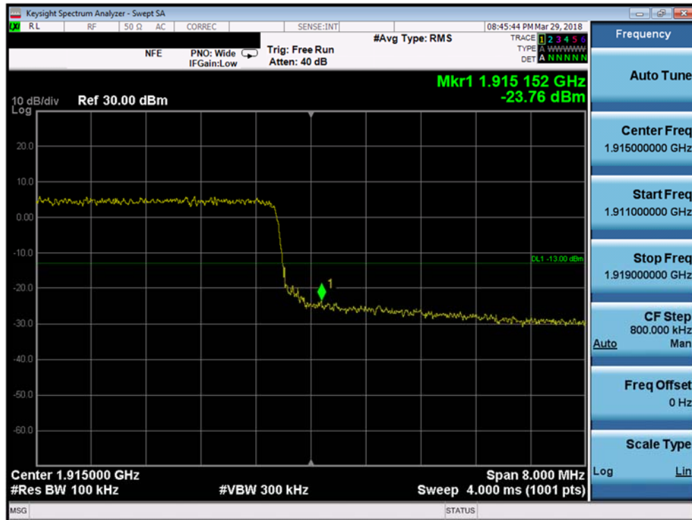
Plot 7-195. Upper Band Edge Plot (Band 25 - 10.0MHz QPSK - Full RB Configuration)
