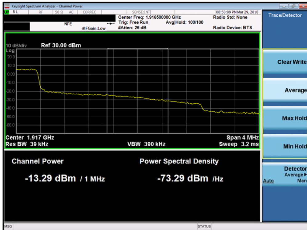
Plot 7-184. Upper Extended Band Edge Plot (Band 25 - 3.0MHz QPSK - Full RB Configuration)
