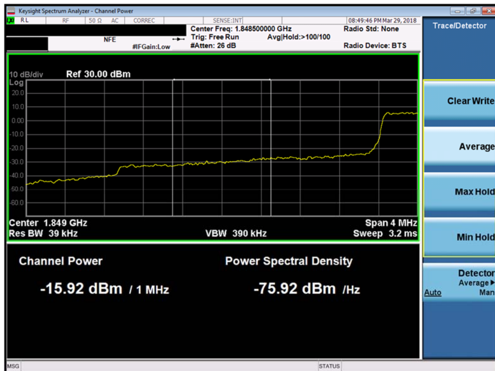
Plot 7-180. Lower Extended Band Edge Plot (Band 25/2 - 3.0MHz QPSK - Full RB Configuration)
