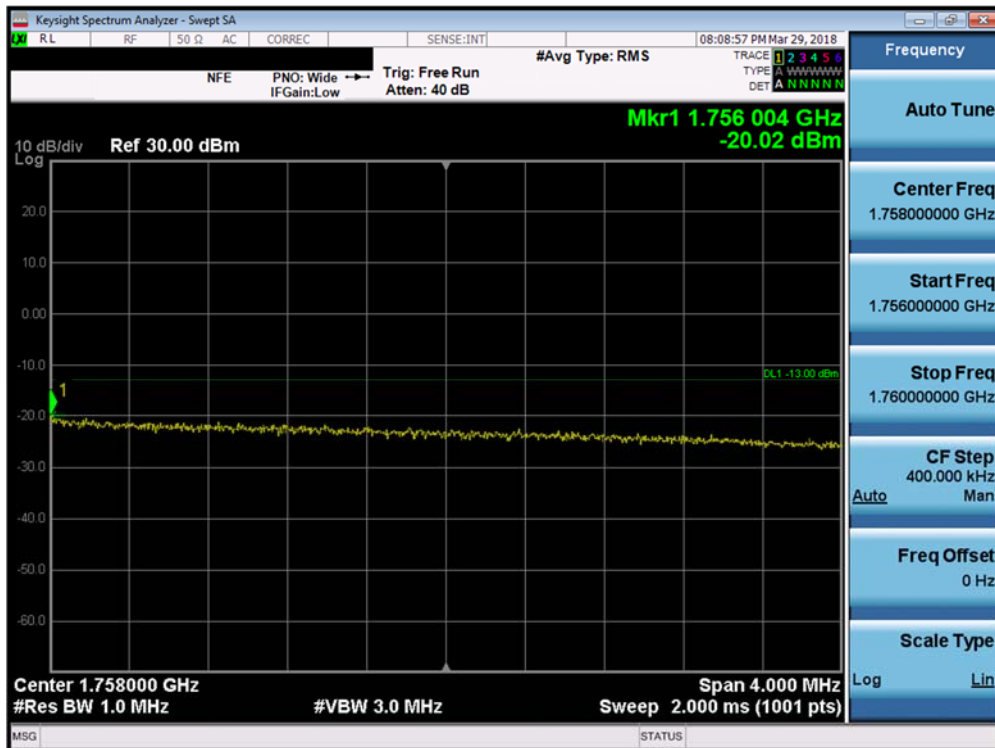
Plot 7-164. Upper Extended Band Edge Plot (Band 4 - 10.0MHz QPSK - Full RB Configuration)
