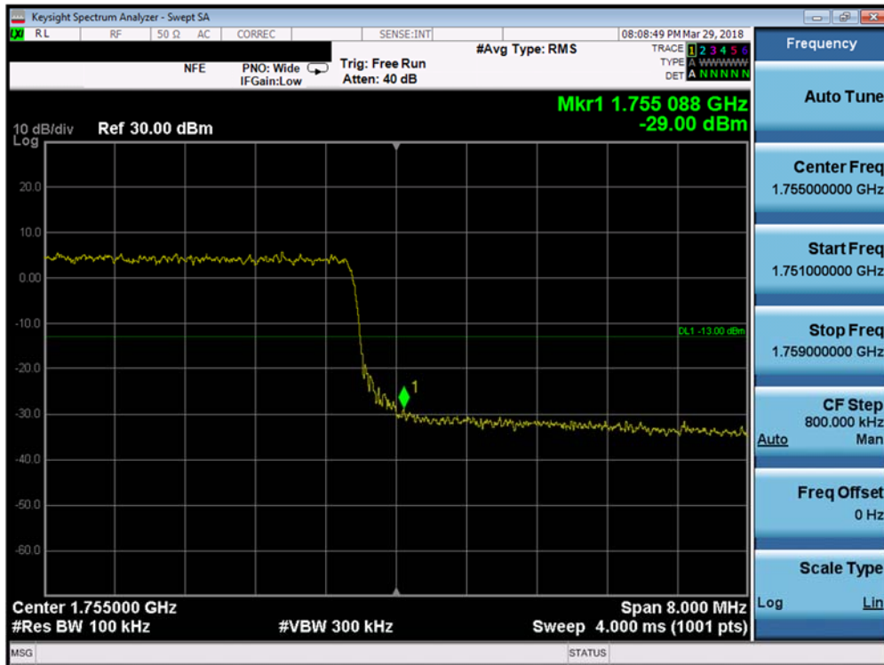
Plot 7-163. Upper Band Edge Plot (Band 4 - 10.0MHz QPSK - Full RB Configuration)
