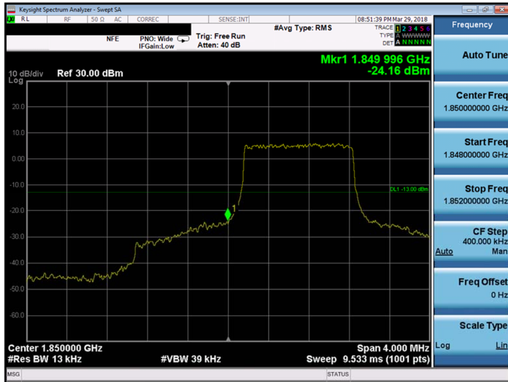
Plot 7-173. Lower Band Edge Plot (Band 25/2 - 1.4MHz QPSK - Full RB Configuration)
