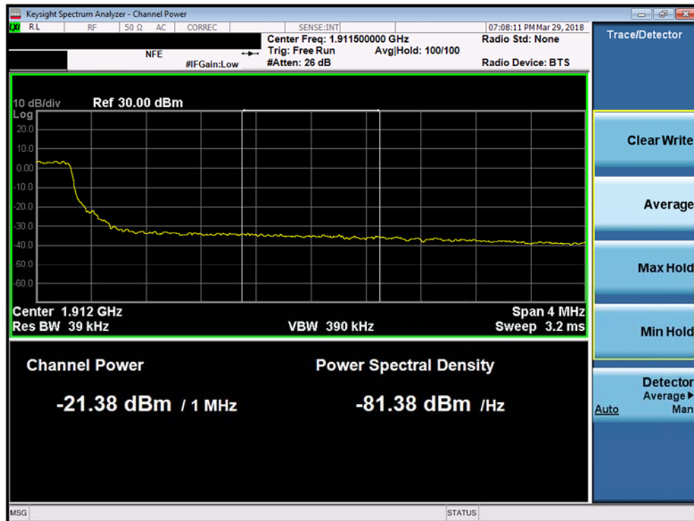
Plot 7-188. Upper Extended Band Edge Plot (Band 2 - 5.0MHz QPSK - Full RB Configuration)
