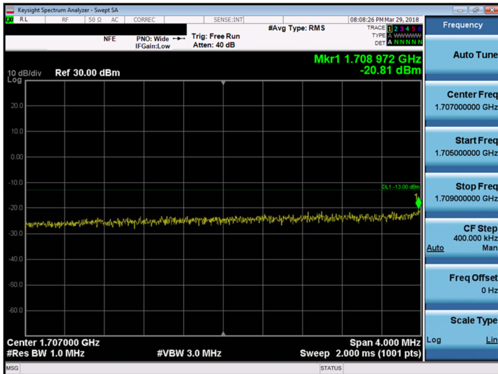
Plot 7-162. Lower Extended Band Edge Plot (Band 4 - 10.0MHz QPSK - Full RB Configuration)
