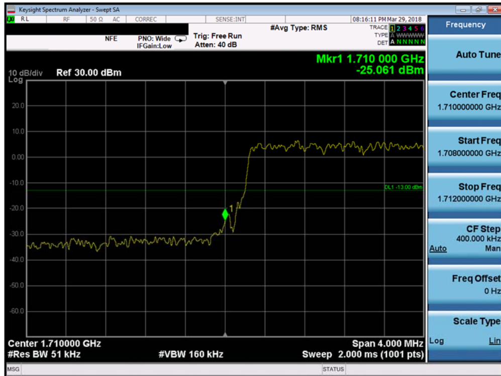
Plot 7-157. Lower Band Edge Plot (Band 4 - 5.0MHz QPSK - Full RB Configuration)
