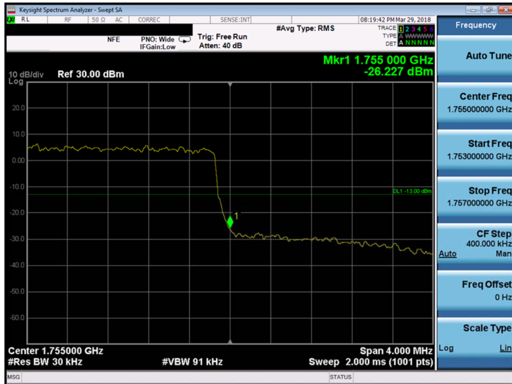
Plot 7-155. Upper Band Edge Plot (Band 4 - 3.0MHz QPSK - Full RB Configuration)
