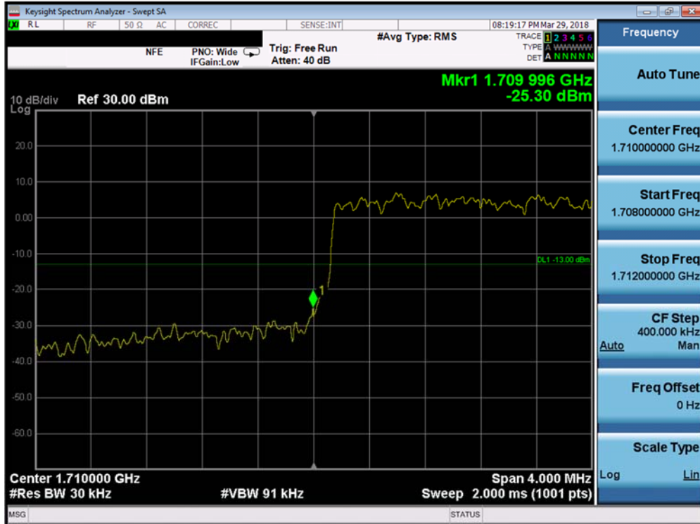
Plot 7-153. Lower Band Edge Plot (Band 4 - 3.0MHz QPSK - Full RB Configuration)
