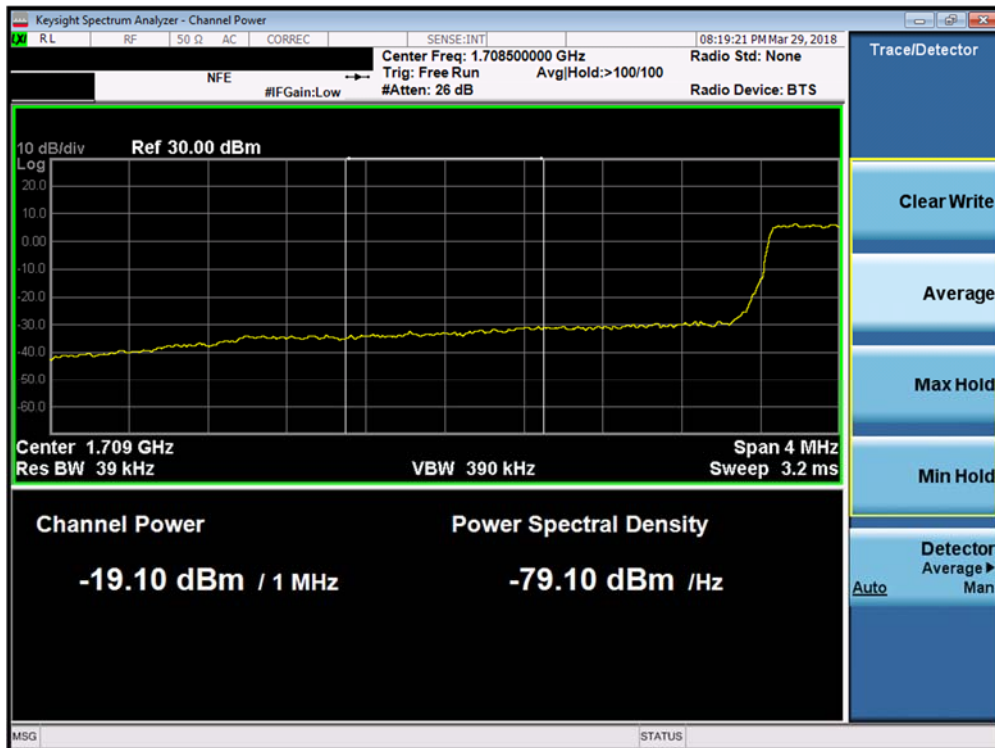
Plot 7-154. Lower Extended Band Edge Plot (Band 4 - 3.0MHz QPSK - Full RB Configuration)
