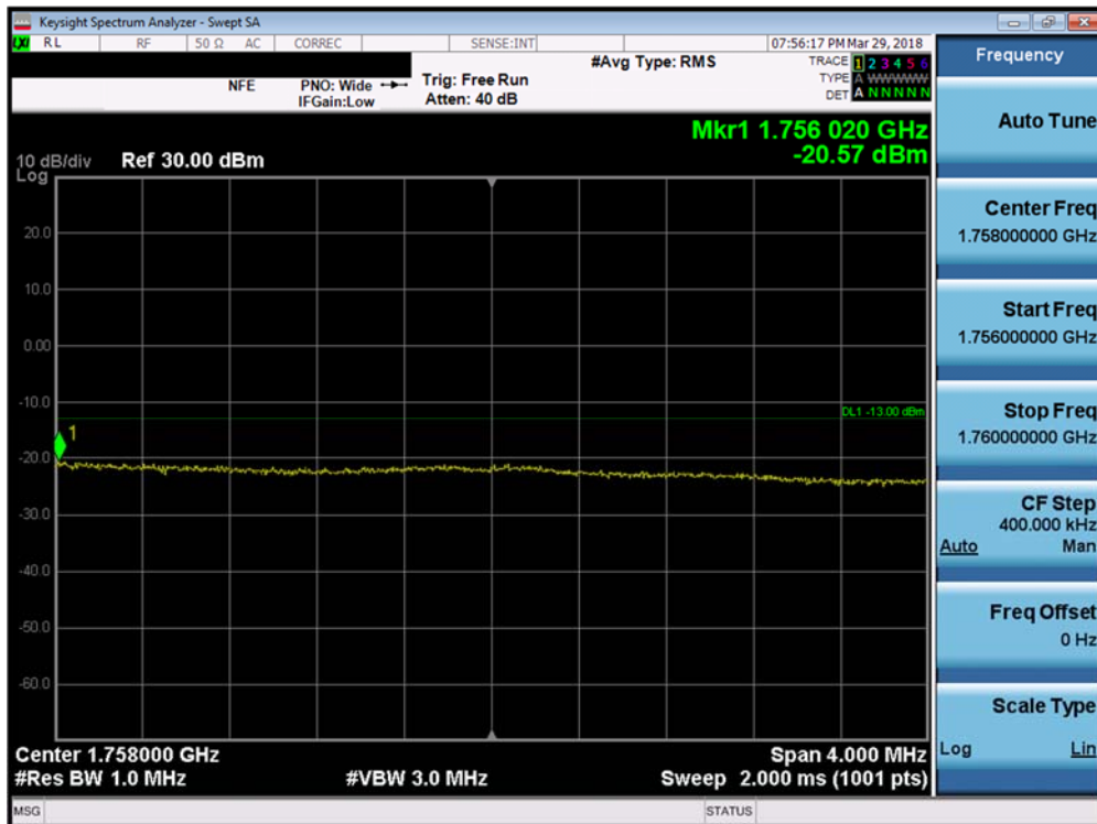
Plot 7-168. Upper Extended Band Edge Plot (Band 4 - 15.0MHz QPSK - Full RB Configuration)
