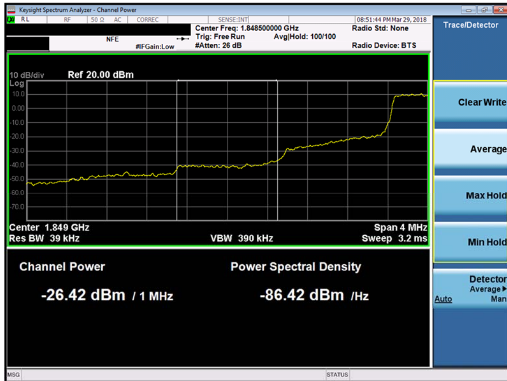
Plot 7-174. Lower Extended Band Edge Plot (Band 25/2 - 1.4MHz QPSK - Full RB Configuration)
