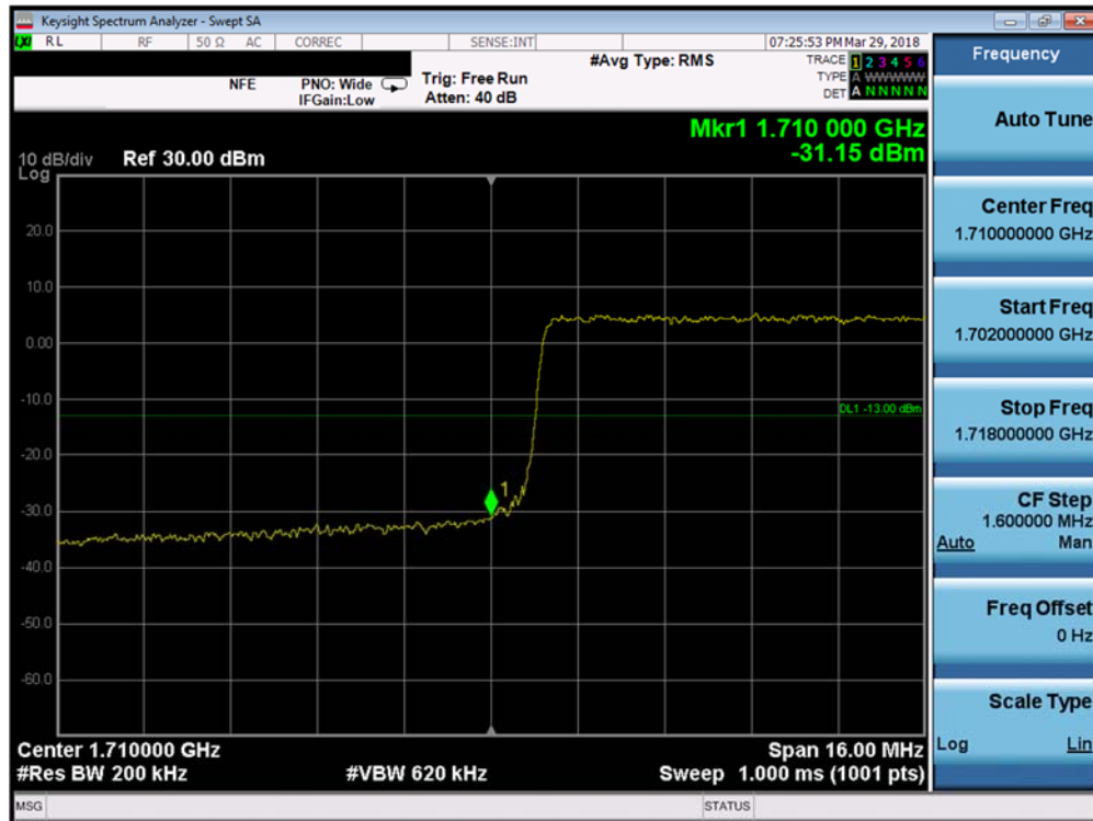
Plot 7-169. Lower Band Edge Plot (Band 4 - 20.0MHz QPSK - Full RB Configuration)
