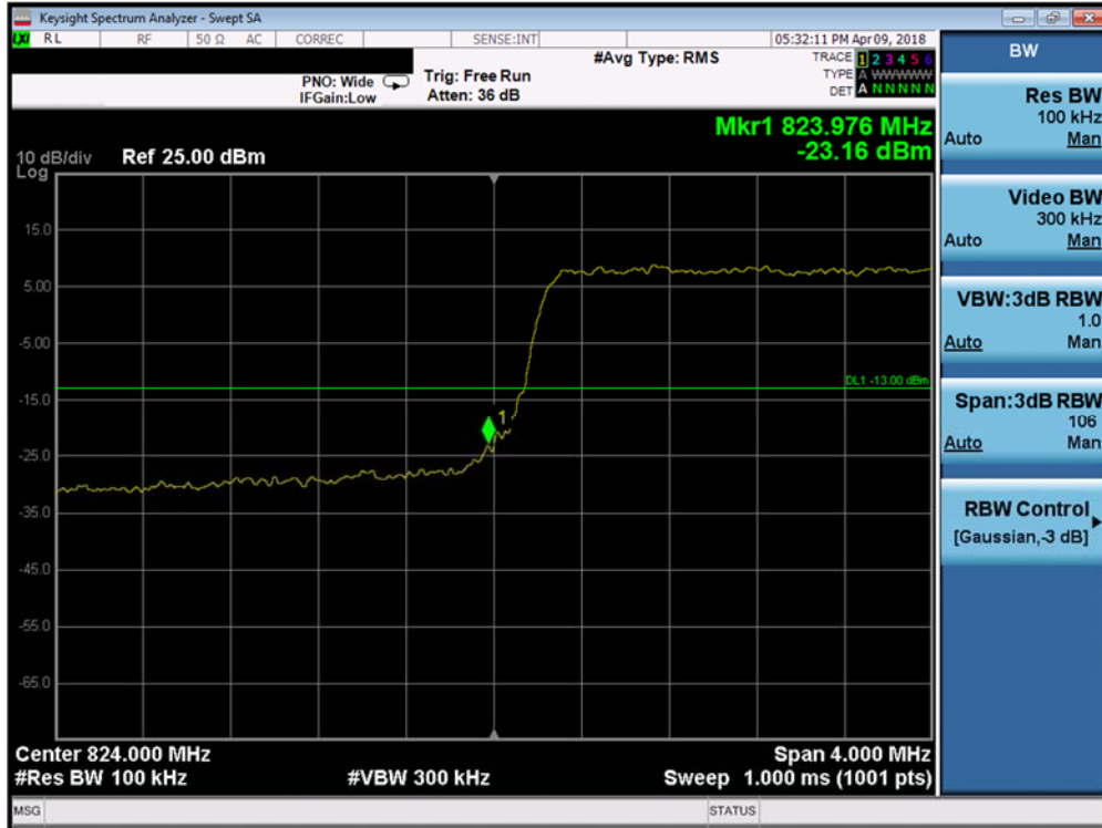
Plot 7-143. Lower Band Edge Plot (Band 26/5 - 5.0MHz QPSK - Full RB Configuration)
