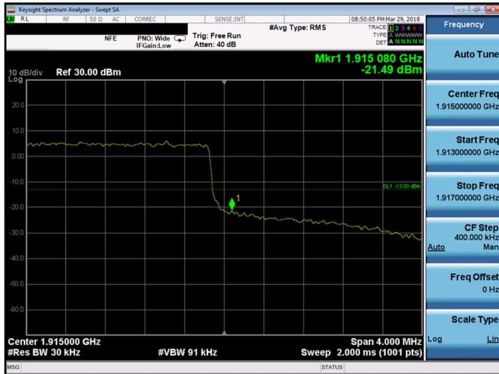
Plot 7-183. Upper Band Edge Plot (Band 25 - 3.0MHz QPSK - Full RB Configuration)
