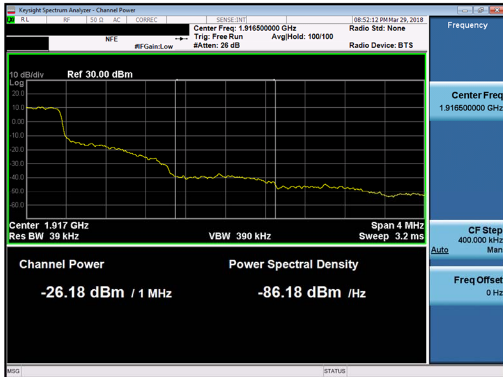
Plot 7-178. Upper Extended Band Edge Plot (Band 25 - 1.4MHz QPSK - Full RB Configuration)
