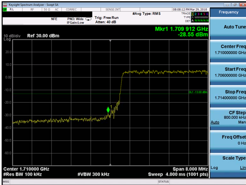
Plot 7-161. Lower Band Edge Plot (Band 4 - 10.0MHz QPSK - Full RB Configuration)
