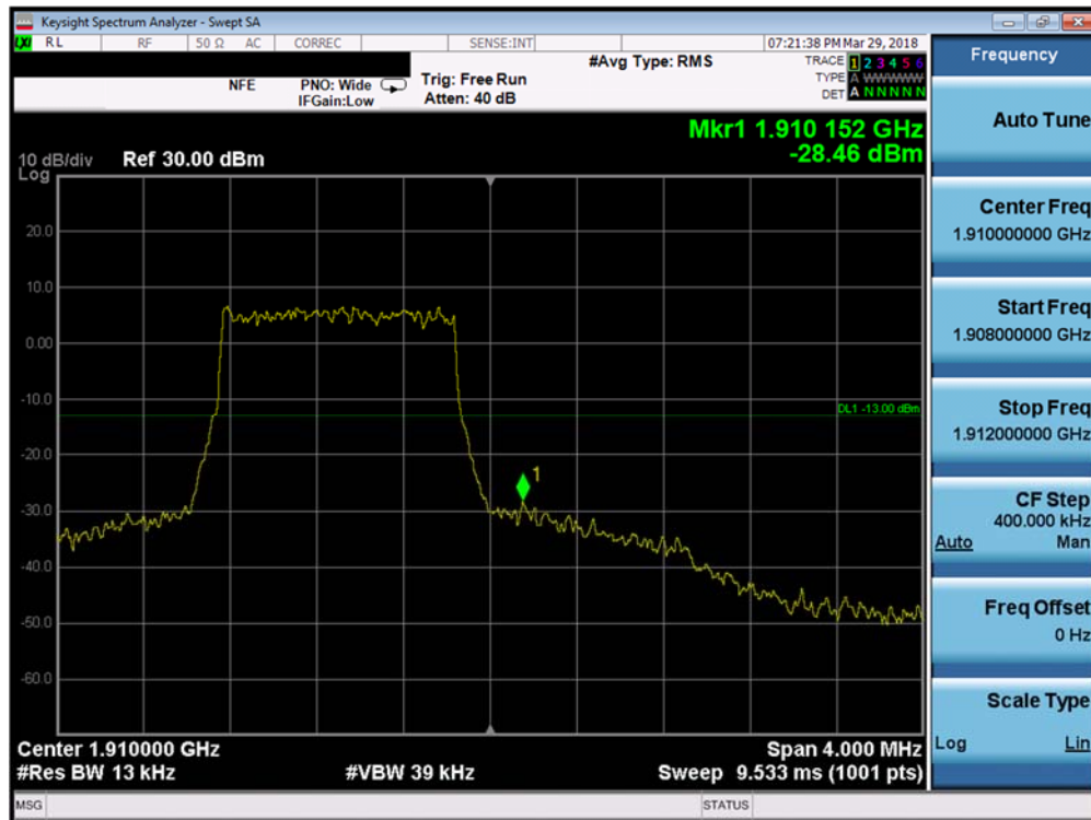
Plot 7-175. Upper Band Edge Plot (Band 2 - 1.4MHz QPSK - Full RB Configuration)
