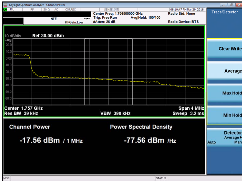
Plot 7-156. Upper Extended Band Edge Plot (Band 4 - 3.0MHz QPSK - Full RB Configuration)
