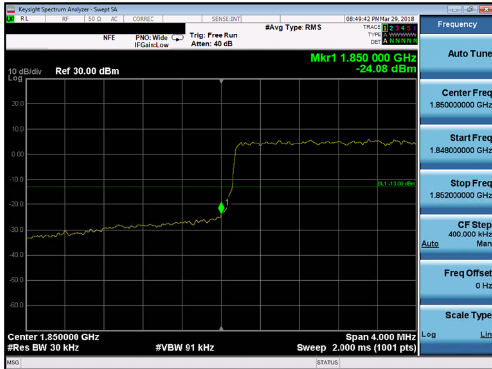
Plot 7-179. Lower Band Edge Plot (Band 25/2 - 3.0MHz QPSK - Full RB Configuration)
