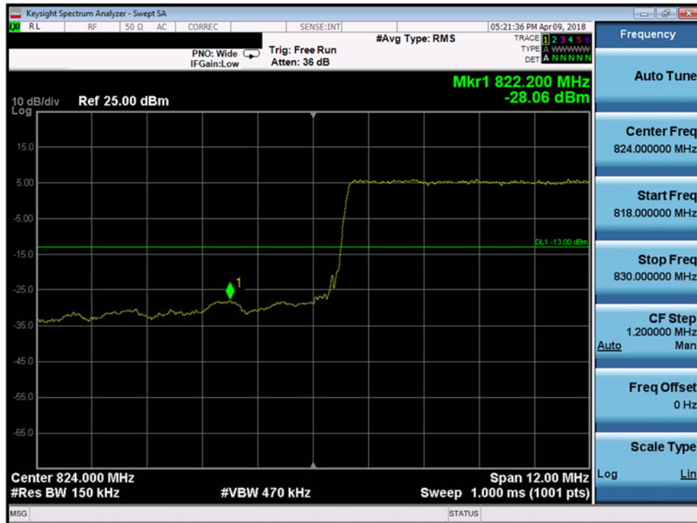
Plot 7-147. Lower Band Edge Plot (Band 26 - 15.0MHz QPSK - Full RB Configuration)
