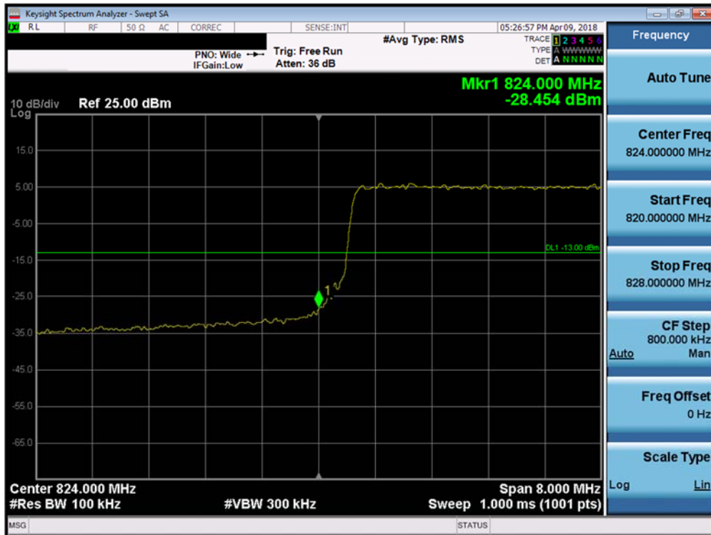
Plot 7-145. Lower Band Edge Plot (Band 26/5 - 10.0MHz QPSK - Full RB Configuration)
