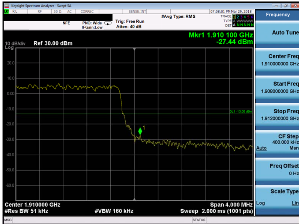
Plot 7-187. Upper Band Edge Plot (Band 2 - 5.0MHz QPSK - Full RB Configuration)
