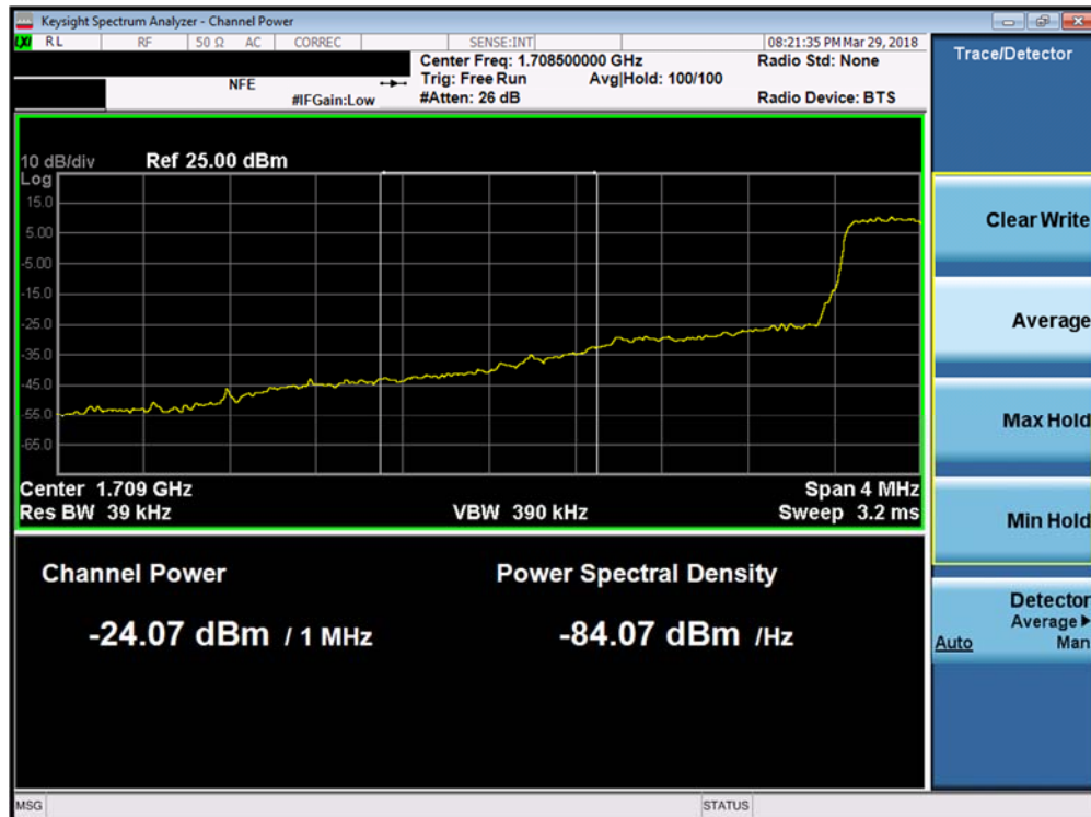
Plot 7-150. Lower Extended Band Edge Plot (Band 4 - 1.4MHz QPSK - Full RB Configuration)
