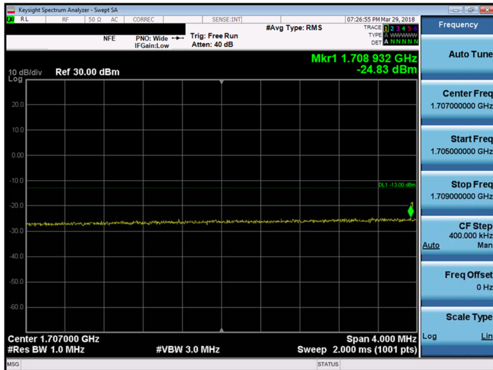
Plot 7-170. Lower Extended Band Edge Plot (Band 4 - 20.0MHz QPSK - Full RB Configuration)
