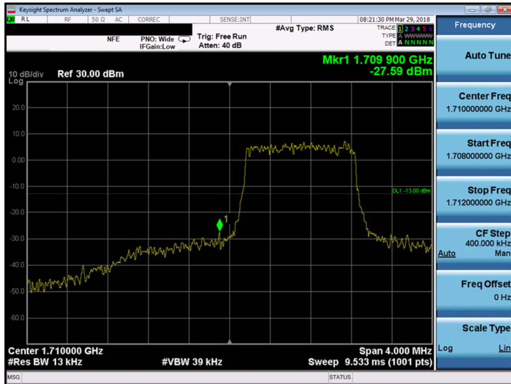
Plot 7-149. Lower Band Edge Plot (Band 4 - 1.4MHz QPSK - Full RB Configuration)
