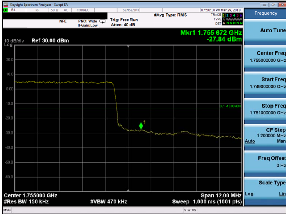
Plot 7-167. Upper Band Edge Plot (Band 4 - 15.0MHz QPSK - Full RB Configuration)
