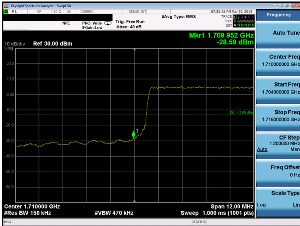
Plot 7-165. Lower Band Edge Plot (Band 4 - 15.0MHz QPSK - Full RB Configuration)
