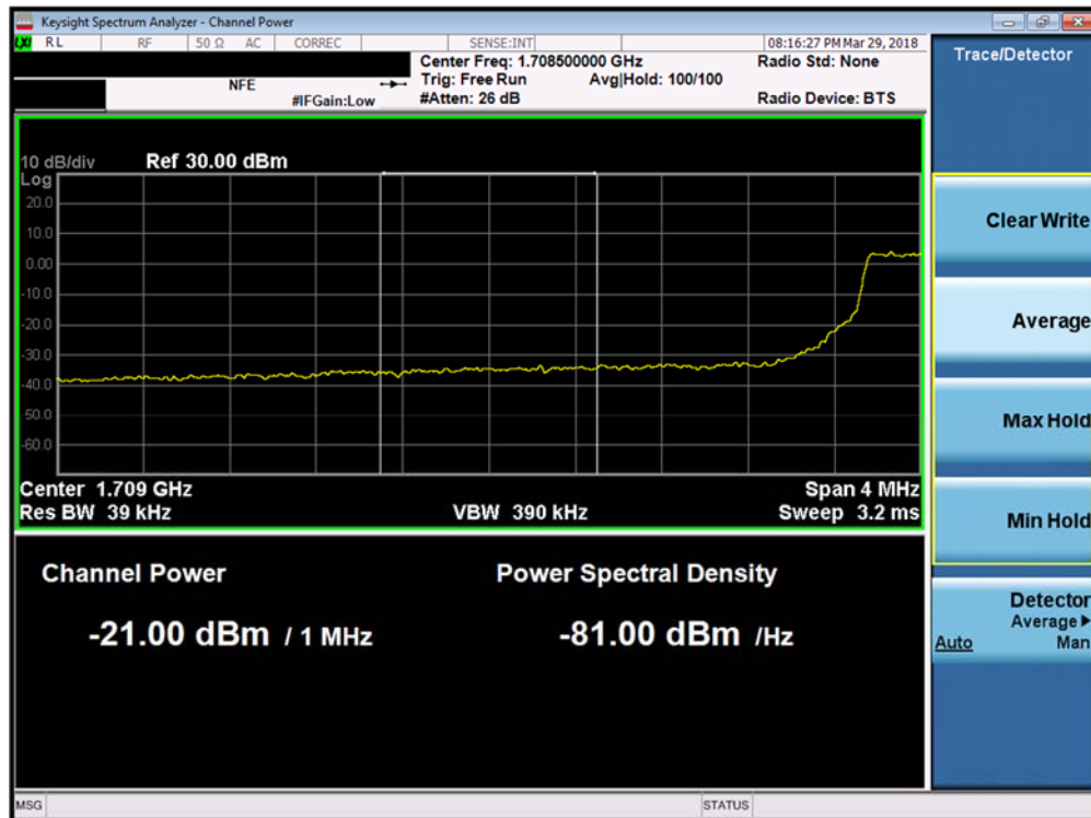
Plot 7-158. Lower Extended Band Edge Plot (Band 4 - 5.0MHz QPSK - Full RB Configuration)
