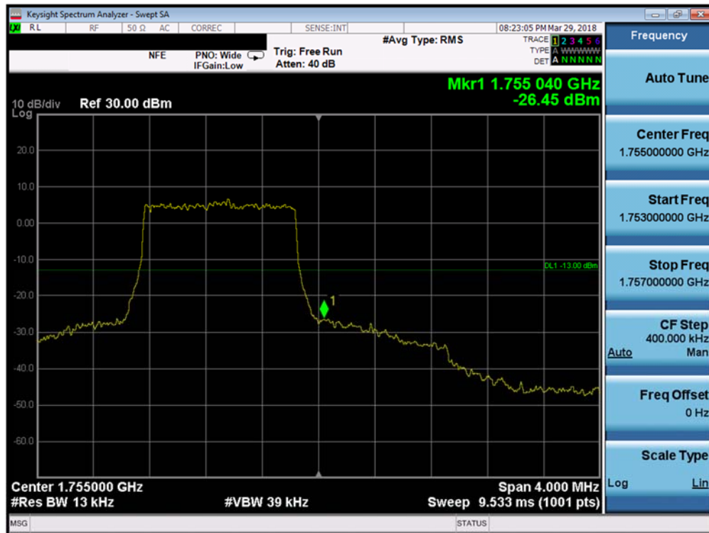
Plot 7-151. Upper Band Edge Plot (Band 4 - 1.4MHz QPSK - Full RB Configuration)
