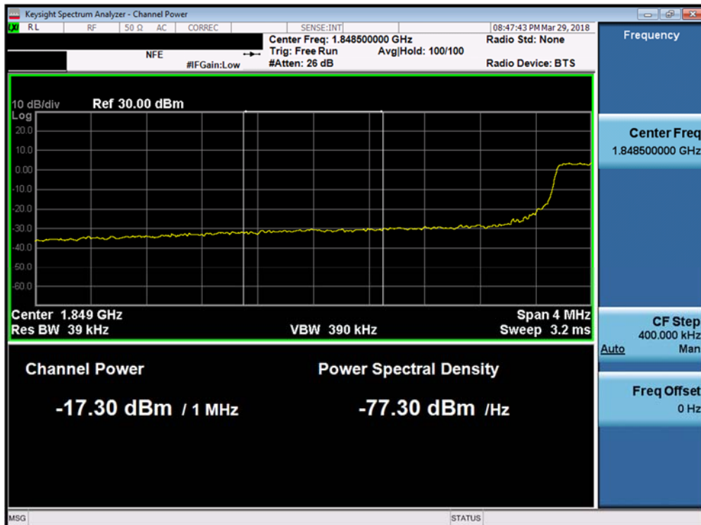
Plot 7-186. Lower Extended Band Edge Plot (Band 25/2 - 5.0MHz QPSK - Full RB Configuration)
