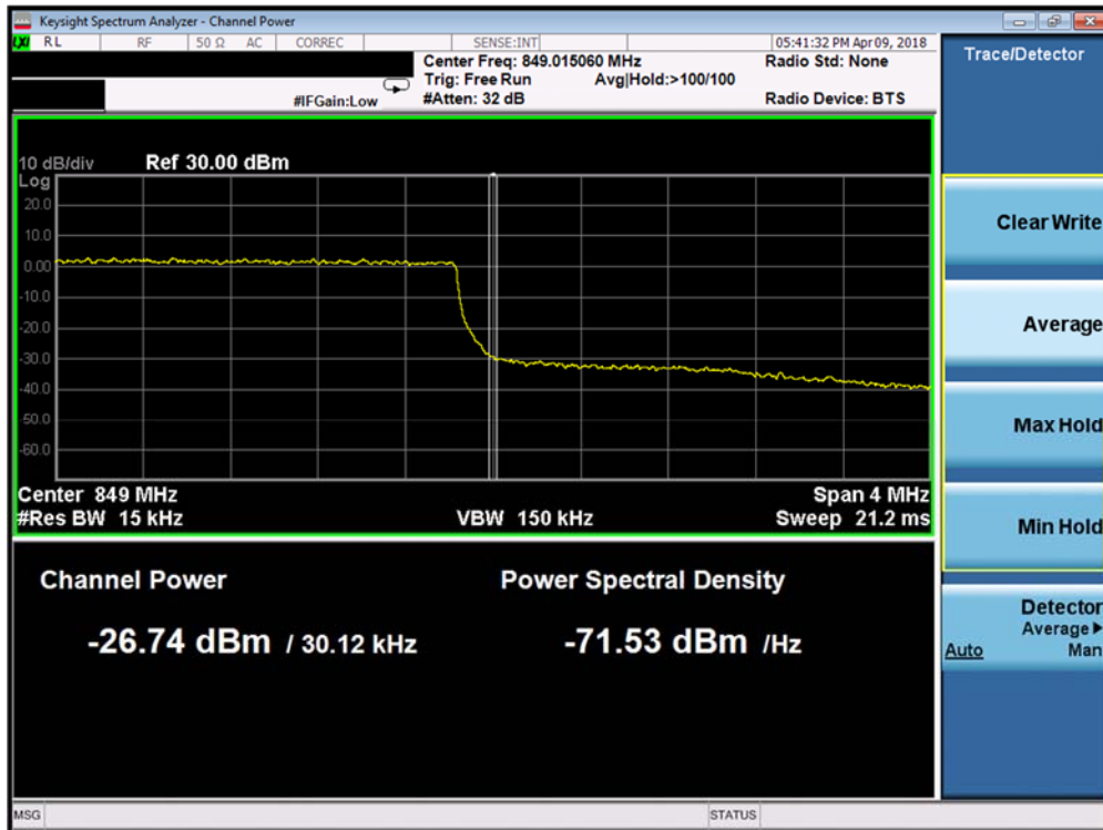
Plot 7-141. Upper Band Edge Plot (Band 26/5 - 3.0MHz QPSK - Full RB Configuration)
