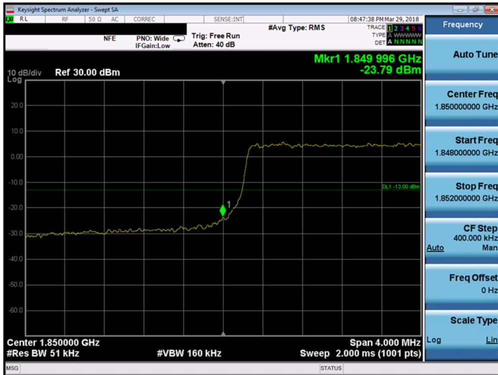
Plot 7-185. Lower Band Edge Plot (Band 25/2 - 5.0MHz QPSK - Full RB Configuration)
