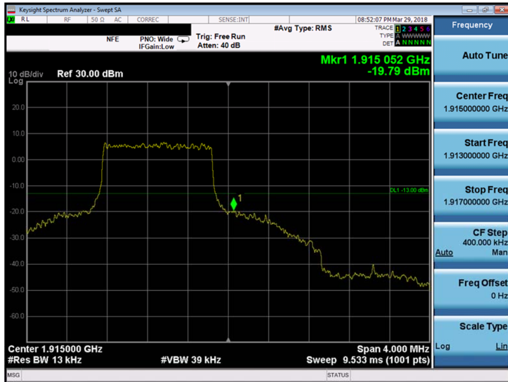
Plot 7-177. Upper Band Edge Plot (Band 25 - 1.4MHz QPSK - Full RB Configuration)
