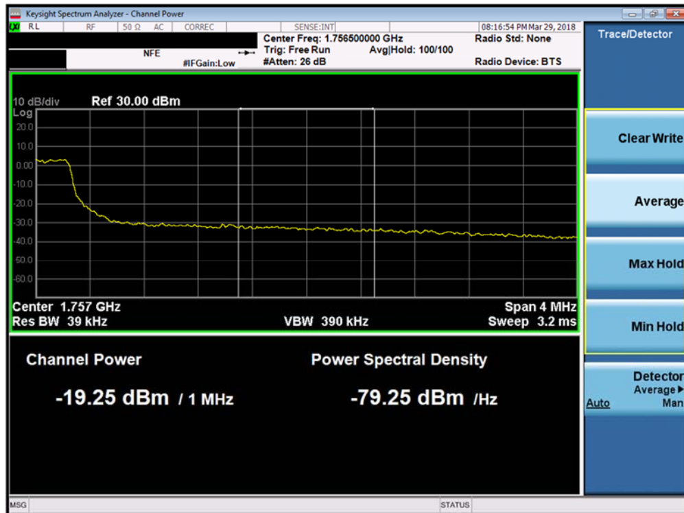
Plot 7-160. Upper Extended Band Edge Plot (Band 4 - 5.0MHz QPSK - Full RB Configuration)
