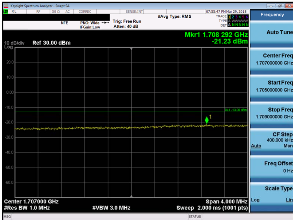
Plot 7-166. Lower Extended Band Edge Plot (Band 4 - 15.0MHz QPSK - Full RB Configuration)
