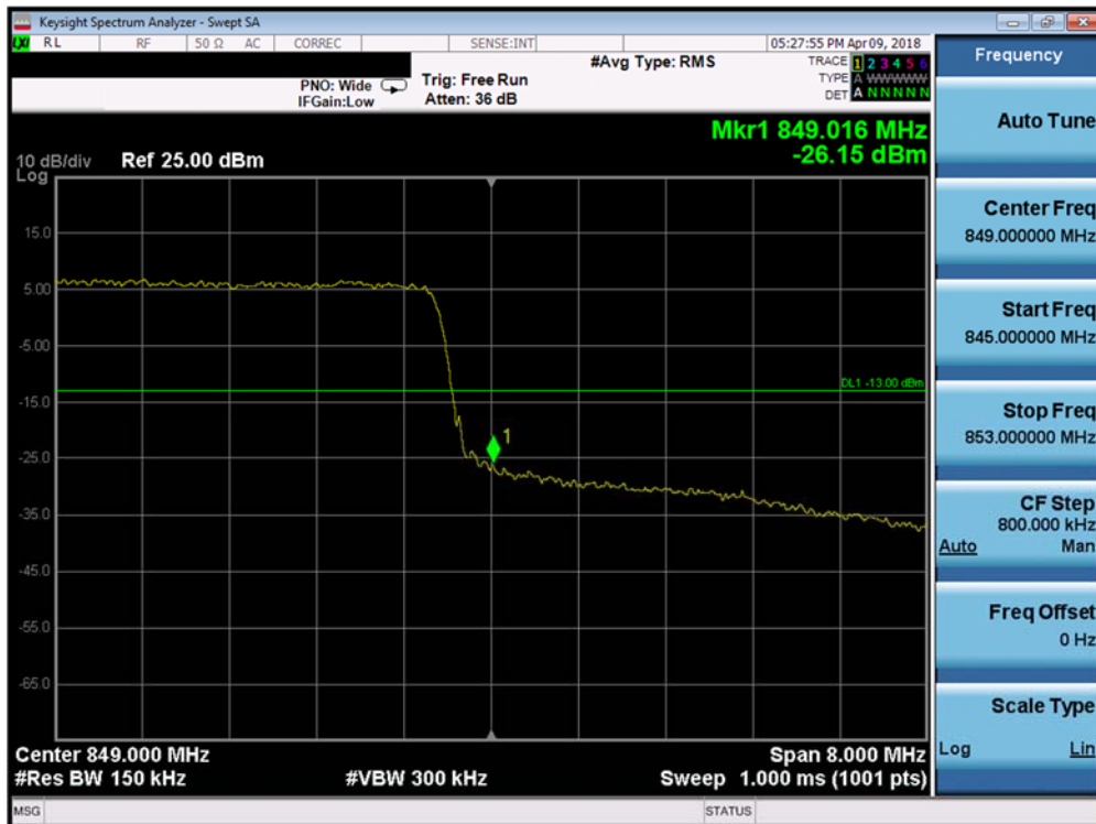
Plot 7-146. Upper Band Edge Plot (Band 26/5 - 10.0MHz QPSK - Full RB Configuration)
