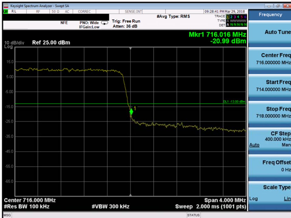
Plot 7-120. Upper Band Edge Plot (Band 12 - 3.0MHz QPSK - Full RB Configuration)
