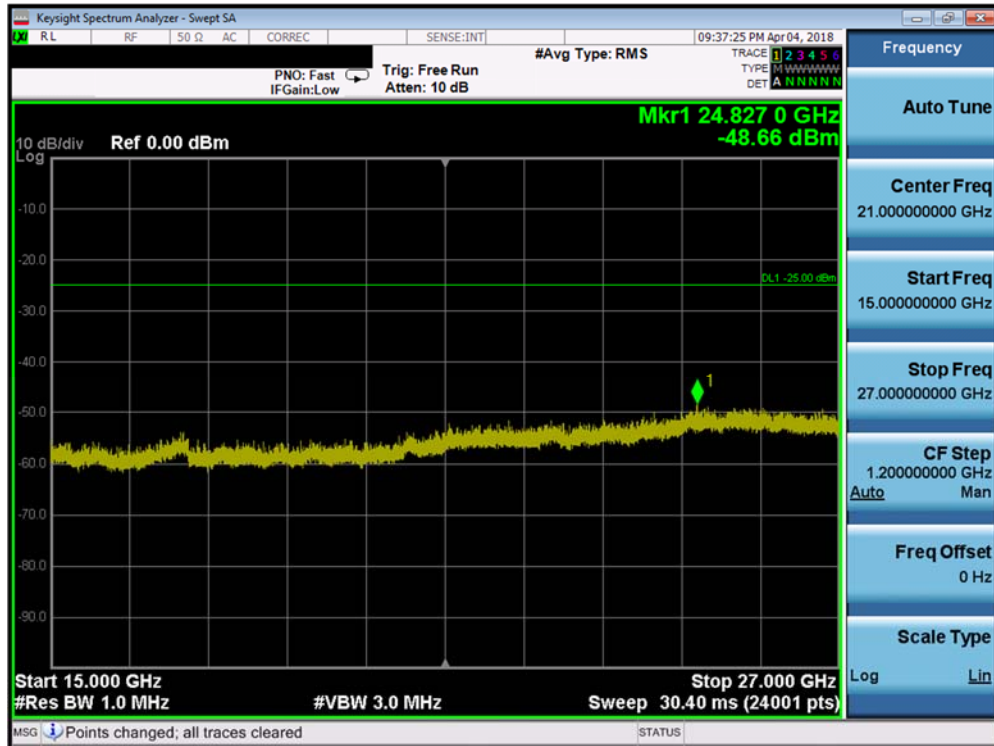
Plot 7-113. Conducted Spurious Plot (Band 41 PC2 - 20.0MHz QPSK - RB Size 1, RB Offset 0 - Mid Channel)
