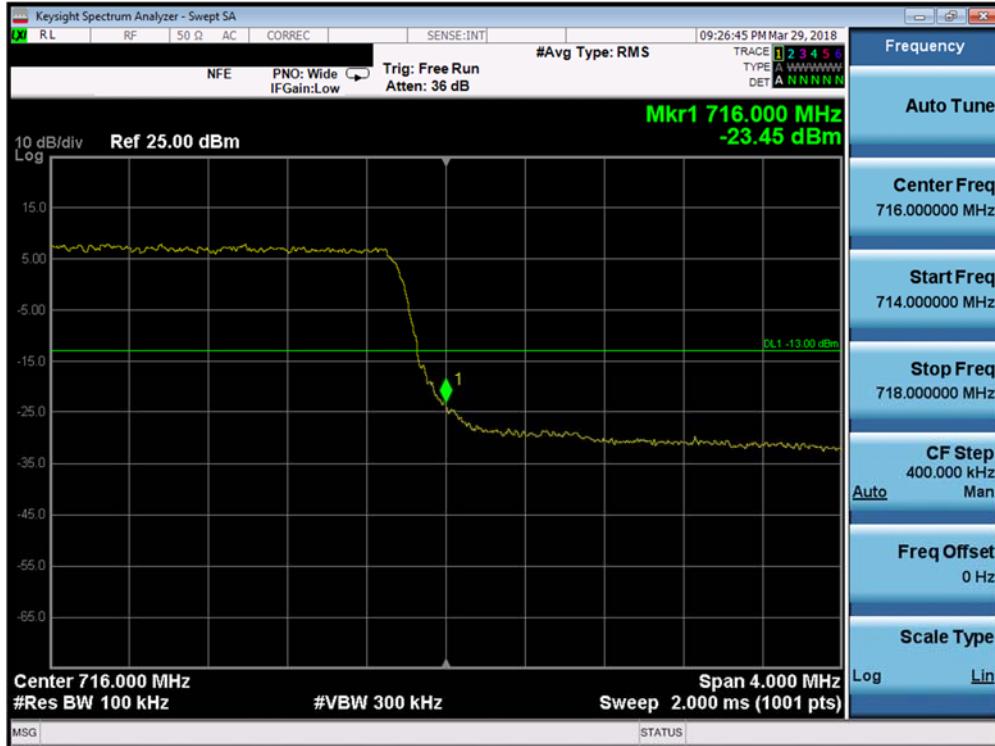
Plot 7-123. Upper Band Edge Plot (Band 12/17 - 5.0MHz QPSK - Full RB Configuration)
