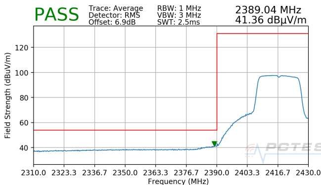
Plot 7-41. Radiated Restricted Lower Band Edge Measurement (Average)
