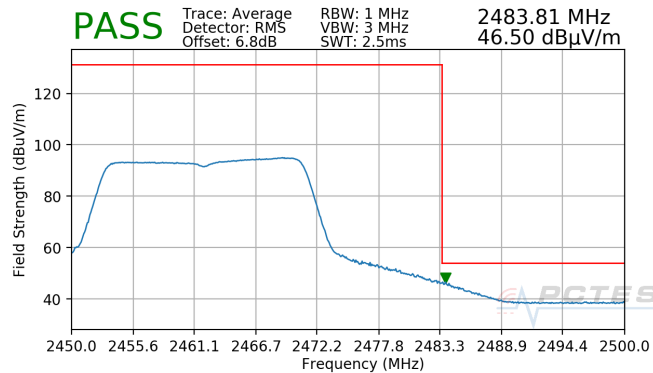
Plot 7-45. Radiated Restricted Upper Band Edge Measurement (Average)
