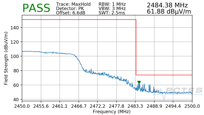
Plot 7-44. Radiated Restricted Upper Band Edge Measurement (Peak)
