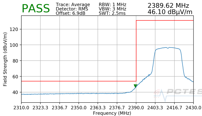
Plot 7-39. Radiated Restricted Lower Band Edge Measurement (Average)
