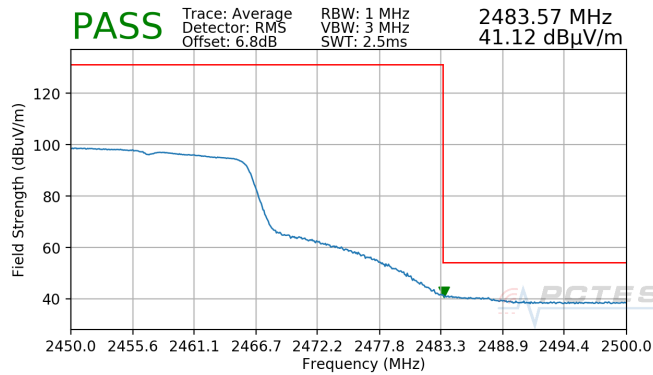
Plot 7-43. Radiated Restricted Upper Band Edge Measurement (Average)
