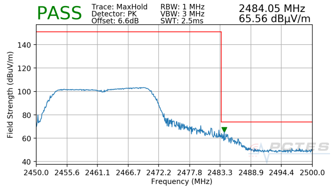
Plot 7-46. Radiated Restricted Upper Band Edge Measurement (Peak)
