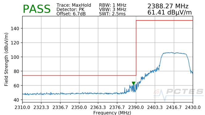
Plot 7-42. Radiated Restricted Lower Band Edge Measurement (Peak)
