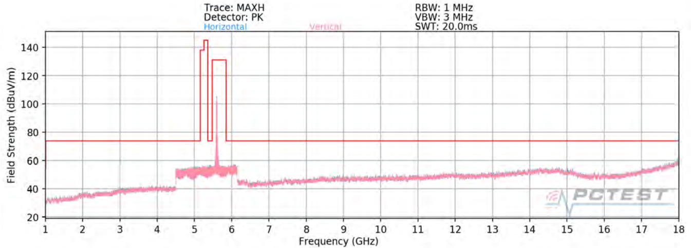
Plot 7-81. Radiated Spurious Plot above 1GHz (802.11a – U2C Ch. 120)
