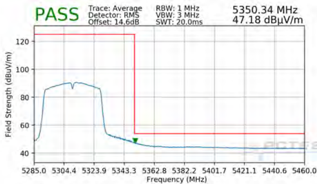
Plot 7-94. Radiated Upper Band Edge Plot (Average – UNII Band 2A)
