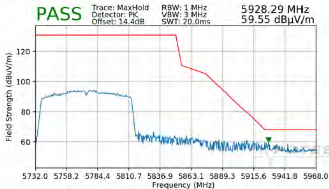
Plot 7-105. Radiated Upper Band Edge Plot (Peak – UNII Band 3)
