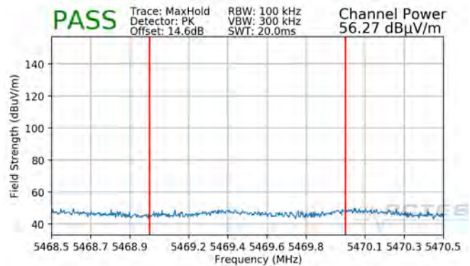
Plot 7-97. Radiated Lower Band Edge Plot (Peak – UNII Band 2C)
