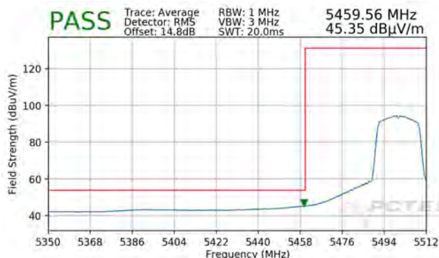
Plot 7-89. Radiated Lower Band Edge Plot (Average – UNII Band 2C)
