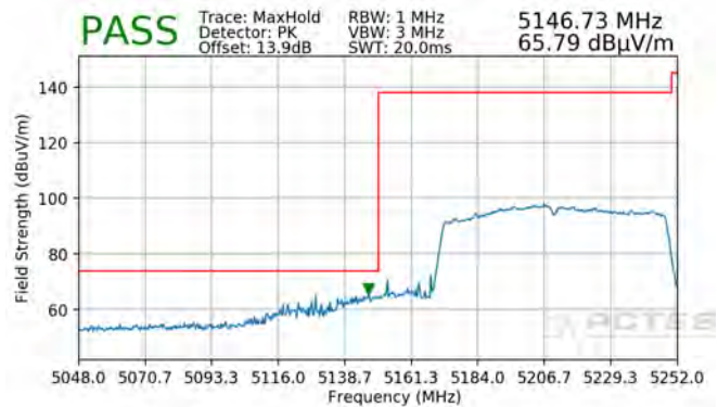
Plot 7-100. Radiated Lower Band Edge Plot (Peak – UNII Band 1)
