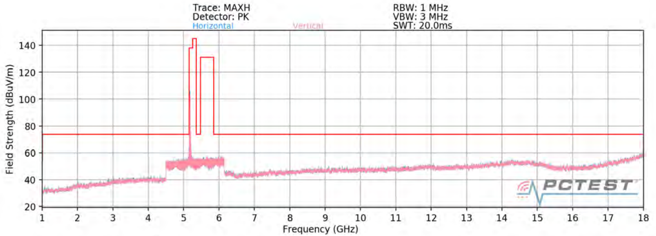
Plot 7-79. Radiated Spurious Plot above 1GHz (802.11a – U1 Ch. 40)
