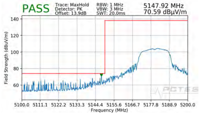
Plot 7-86. Radiated Lower Band Edge Plot (Peak – UNII Band 1)
