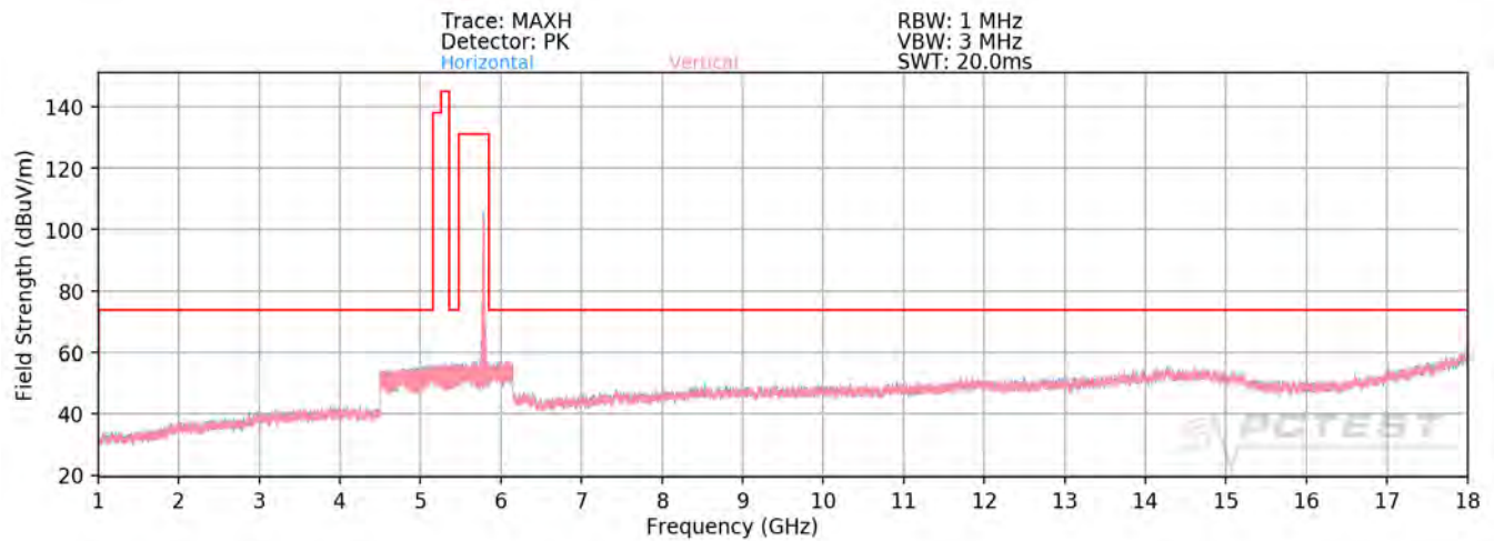
Plot 7-82. Radiated Spurious Plot above 1GHz (802.11a – U3 Ch. 157)
