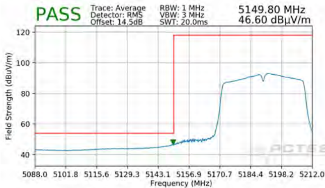
Plot 7-92. Radiated Lower Band Edge Plot (Average – UNII Band 1)
