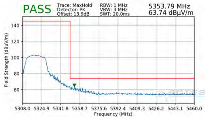
Plot 7-88. Radiated Upper Band Edge Plot (Peak – UNII Band 2A)
