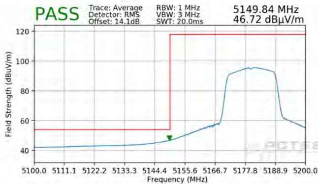
Plot 7-85. Radiated Lower Band Edge Plot (Average – UNII Band 1)
