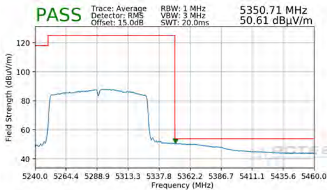
Plot 7-101. Radiated Upper Band Edge Plot (Average – UNII Band 2A)
