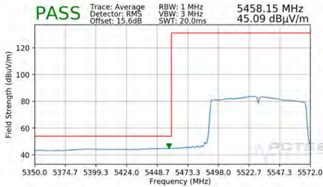
Plot 7-103. Radiated Lower Band Edge Plot (Average – UNII Band 2C)
