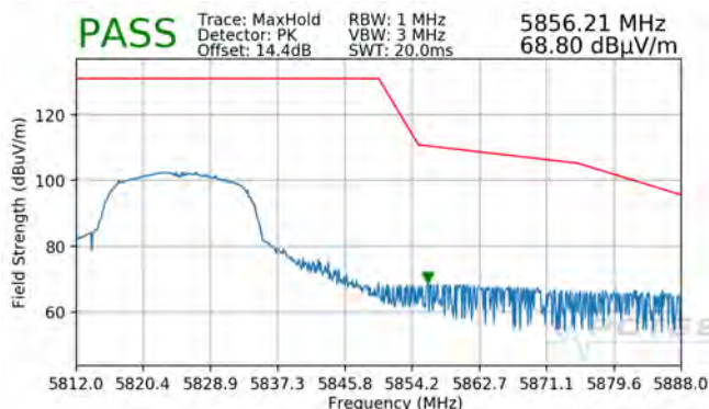
Plot 7-91. Radiated Upper Band Edge Plot (Peak – UNII Band 3)
