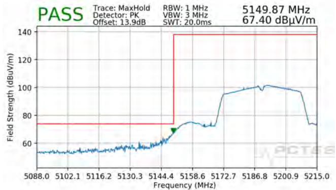
Plot 7-93. Radiated Lower Band Edge Plot (Peak – UNII Band 1)
