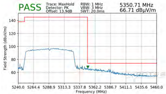
Plot 7-102. Radiated Upper Band Edge Plot (Peak – UNII Band 2A)
