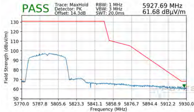
Plot 7-98. Radiated Upper Band Edge Plot (Peak – UNII Band 3)
