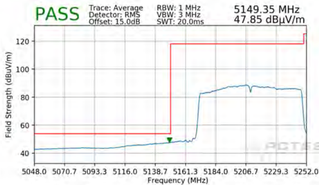
Plot 7-99. Radiated Lower Band Edge Plot (Average – UNII Band 1)
