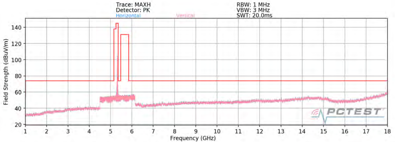
Plot 7-80. Radiated Spurious Plot above 1GHz (802.11a – U2A Ch. 56)
