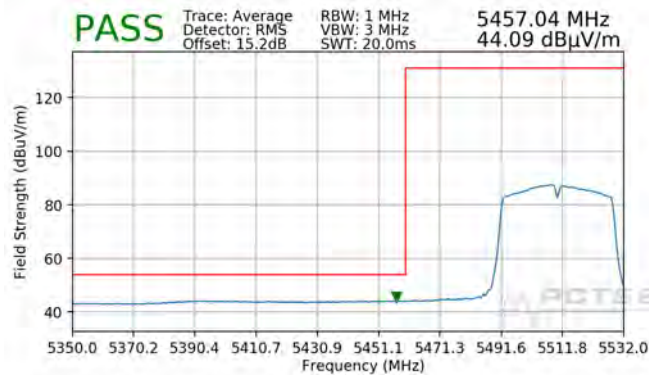
Plot 7-96. Radiated Lower Band Edge Plot (Average – UNII Band 2C)
