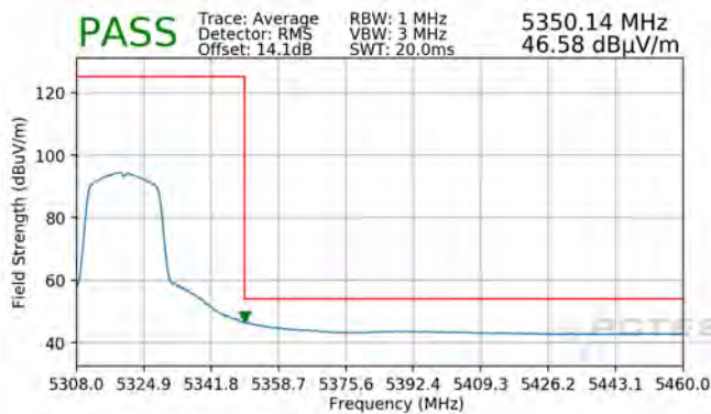
Plot 7-87. Radiated Upper Band Edge Plot (Average – UNII Band 2A)
