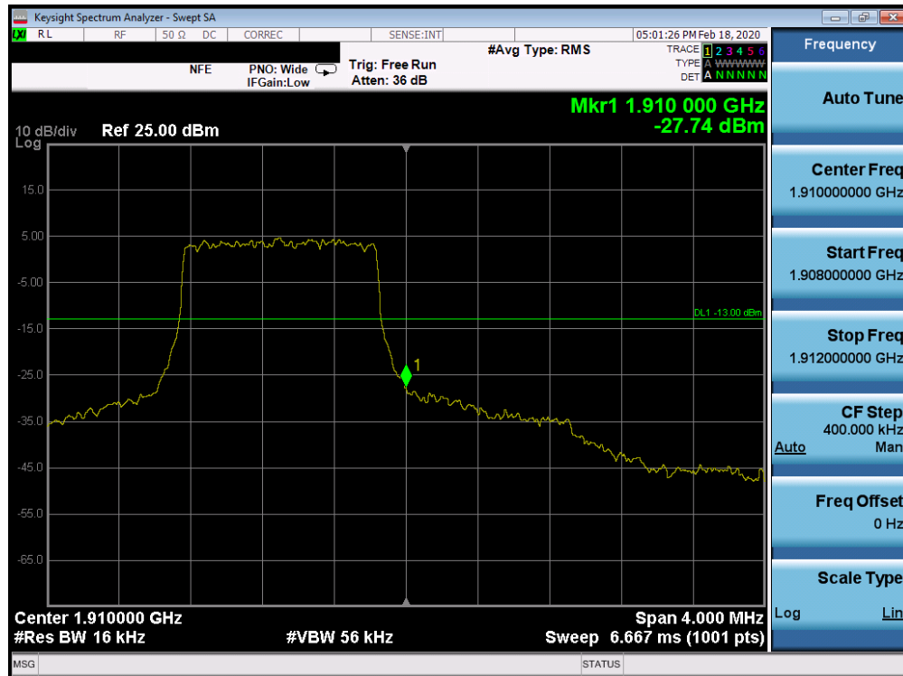
Plot 7-172. Upper Band Edge Plot (Band 2 - 1.4MHz QPSK - Full RB Configuration)
