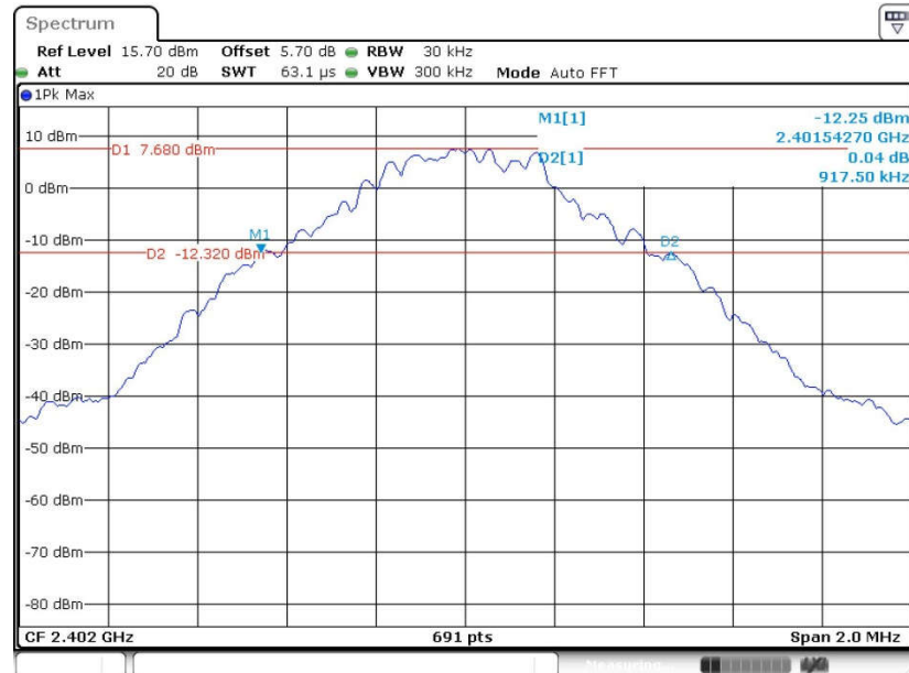
20 dB Bandwidth Plot on Channel 00
