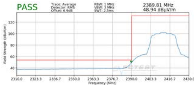
Plot 7-55. Radiated Restricted Lower Band Edge Measurement (Average)
