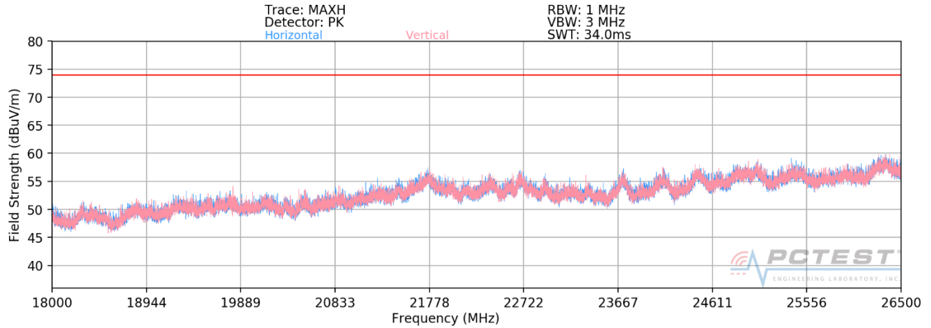
Plot 7-54. Radiated Spurious Plot above 18GHz
