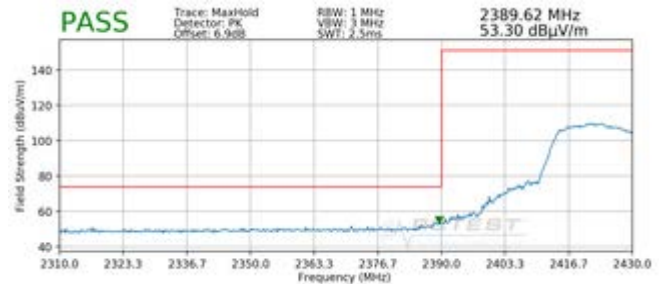
Plot 7-60. Radiated Restricted Lower Band Edge Measurement (Peak)
