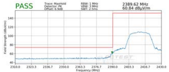
Plot 7-56. Radiated Restricted Lower Band Edge Measurement (Peak)
