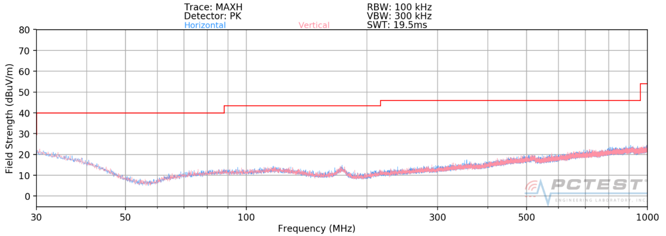
Plot 7-67. Radiated Spurious Plot below 1GHz
