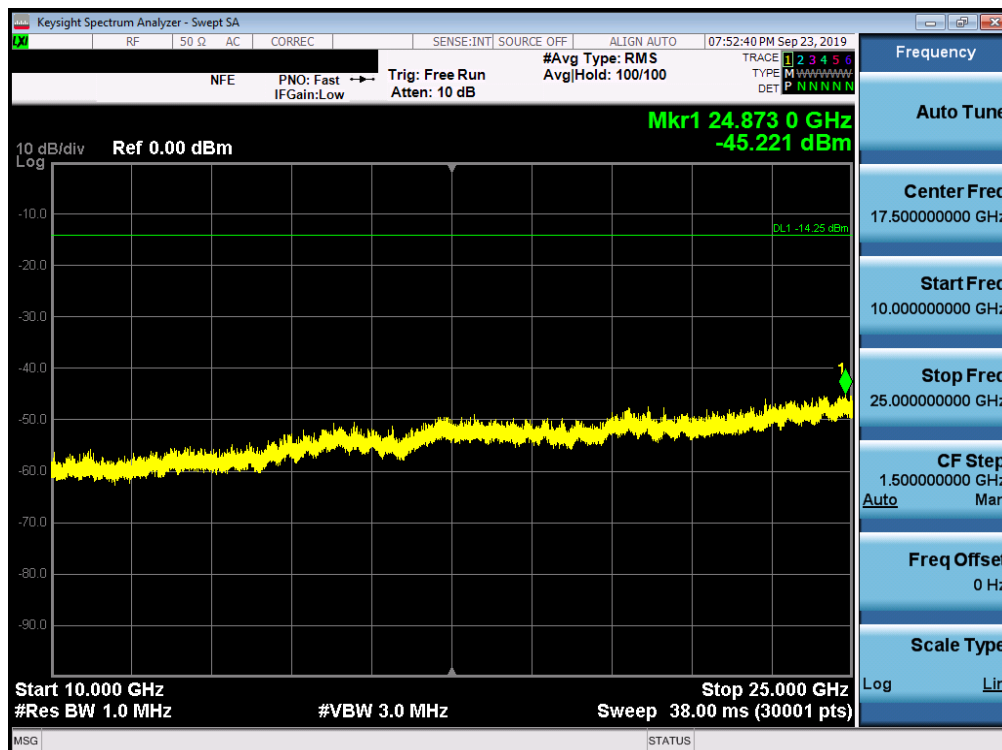
Plot 7-48. Conducted Spurious Plot (802.11ac – Ch. 6)
