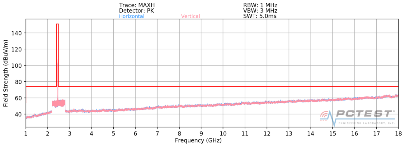
Plot 7-53. Radiated Spurious Plot above 1GHz (802.11b – Ch. 11)
