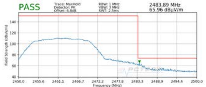
Plot 7-66. Radiated Restricted Upper Band Edge Measurement (Peak)
