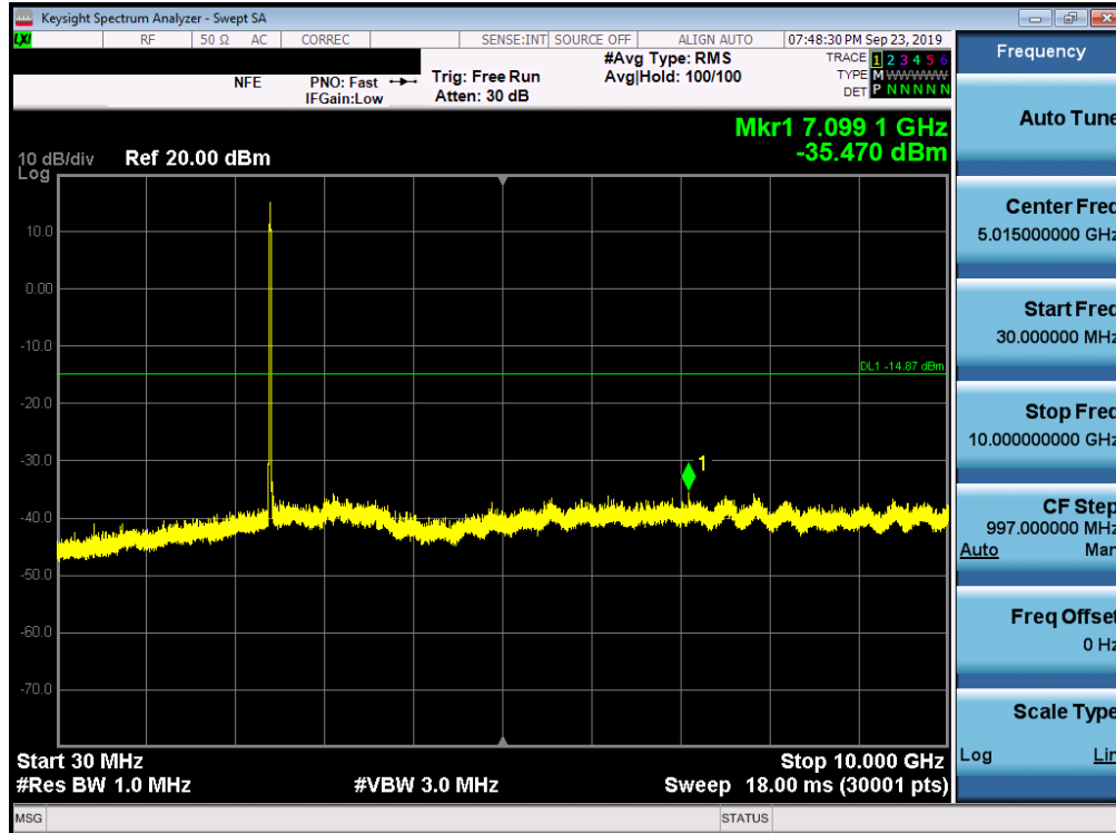
Plot 7-45. Conducted Spurious Plot (802.11ac – Ch. 1)
