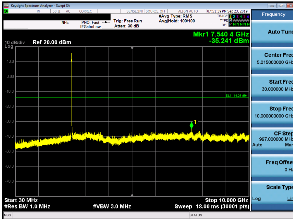
Plot 7-47. Conducted Spurious Plot (802.11ac – Ch. 6)
