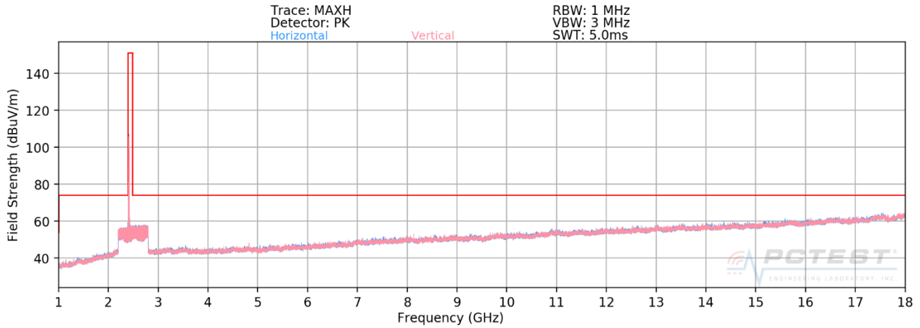
Plot 7-51. Radiated Spurious Plot above 1GHz (802.11b – Ch. 1)
