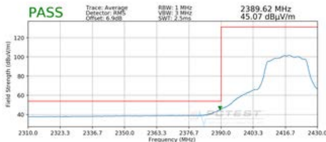
Plot 7-57. Radiated Restricted Lower Band Edge Measurement (Average)
