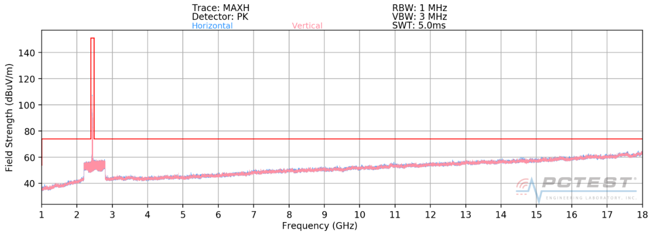
Plot 7-52. Radiated Spurious Plot above 1GHz (802.11b – Ch. 6)
