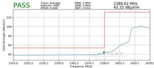
Plot 7-59. Radiated Restricted Lower Band Edge Measurement (Average)
