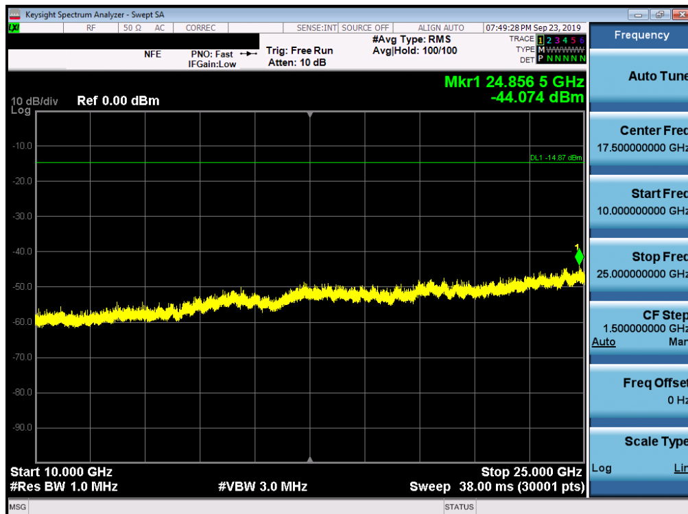
Plot 7-46. Conducted Spurious Plot (802.11ac – Ch. 1)
