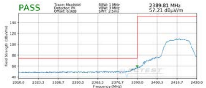
Plot 7-58. Radiated Restricted Lower Band Edge Measurement (Peak)
