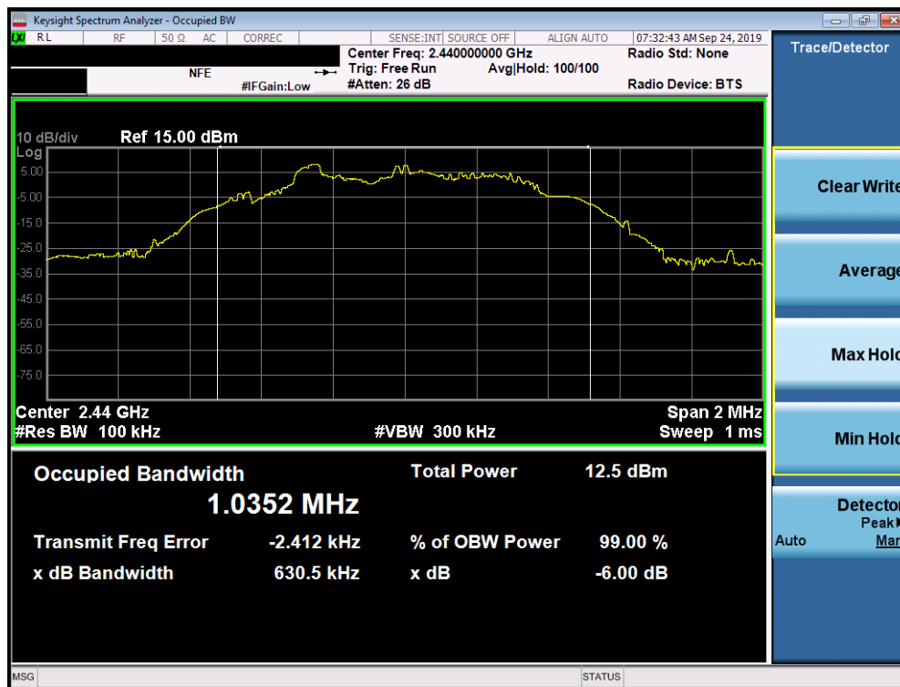
Plot 7-5. 6dB Bandwidth Plot (Bluetooth (LE), 500kbps – Ch. 19)
