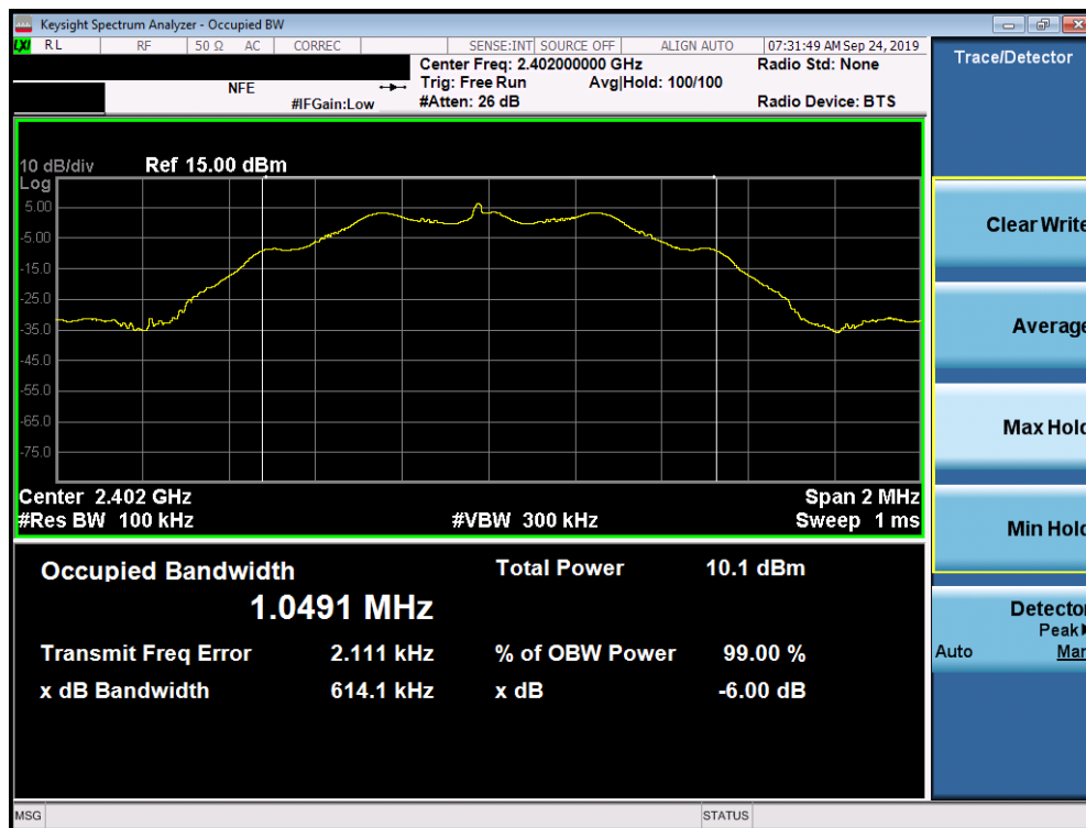
Plot 7-1. 6dB Bandwidth Plot (Bluetooth (LE), 125kbps – Ch. 0)
