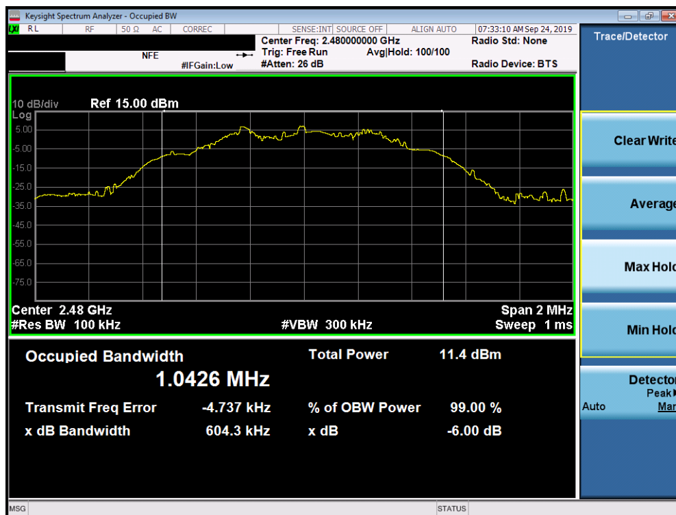
Plot 7-6. 6dB Bandwidth Plot (Bluetooth (LE), 500kbps – Ch. 39)
