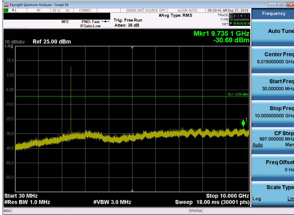
Plot 7-36. Conducted Spurious Plot (Bluetooth, 1Mbps - Ch. 0)
