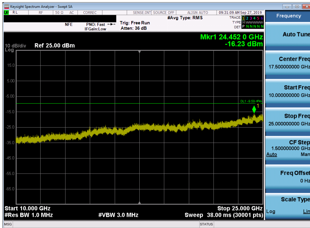
Plot 7-37. Conducted Spurious Plot (Bluetooth, 1Mbps - Ch. 0)
