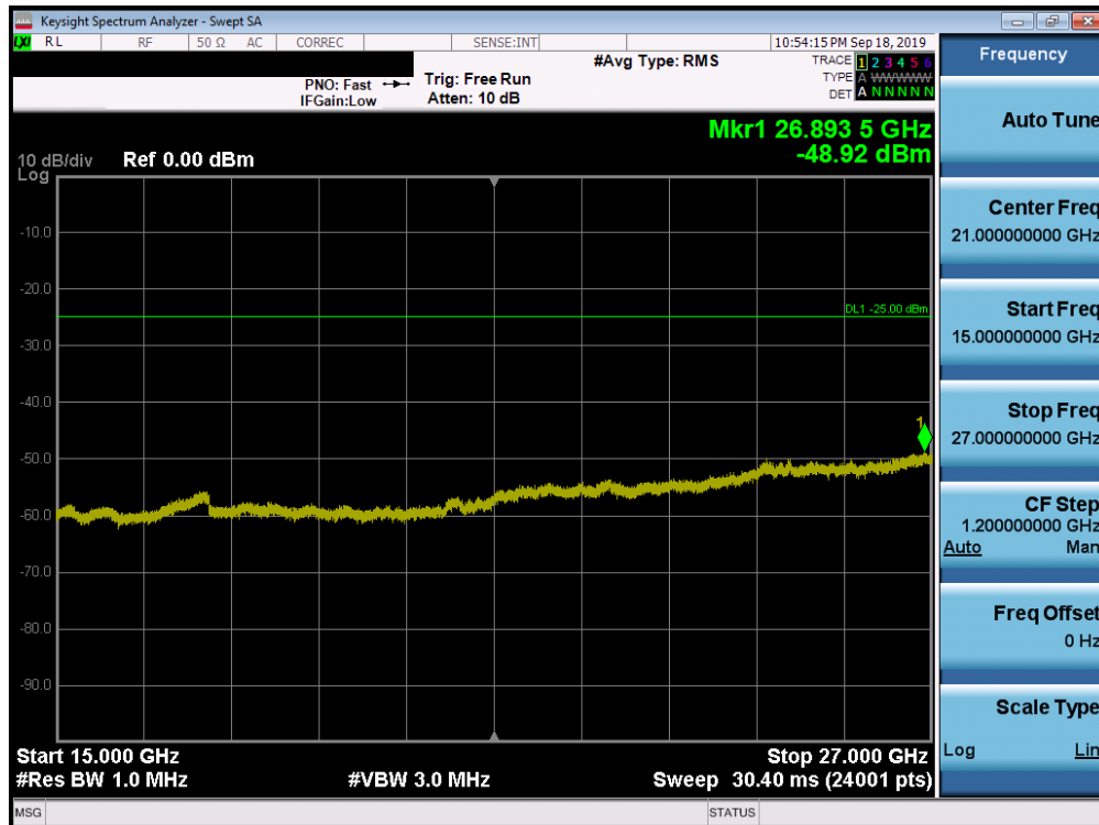
Plot 7-159. Conducted Spurious Plot (Band 7 - 20.0MHz QPSK - RB Size 1, RB Offset 0 - Mid Channel)
