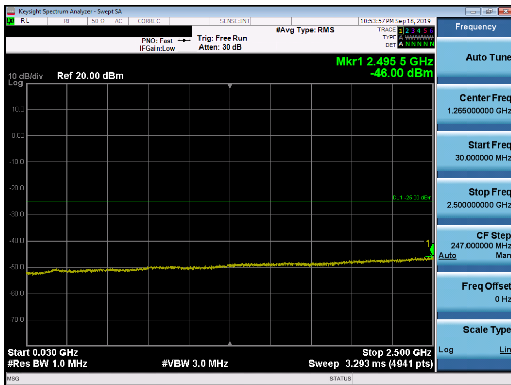
Plot 7-157. Conducted Spurious Plot (Band 7 - 20.0MHz QPSK - RB Size 1, RB Offset 0 - Mid Channel)
