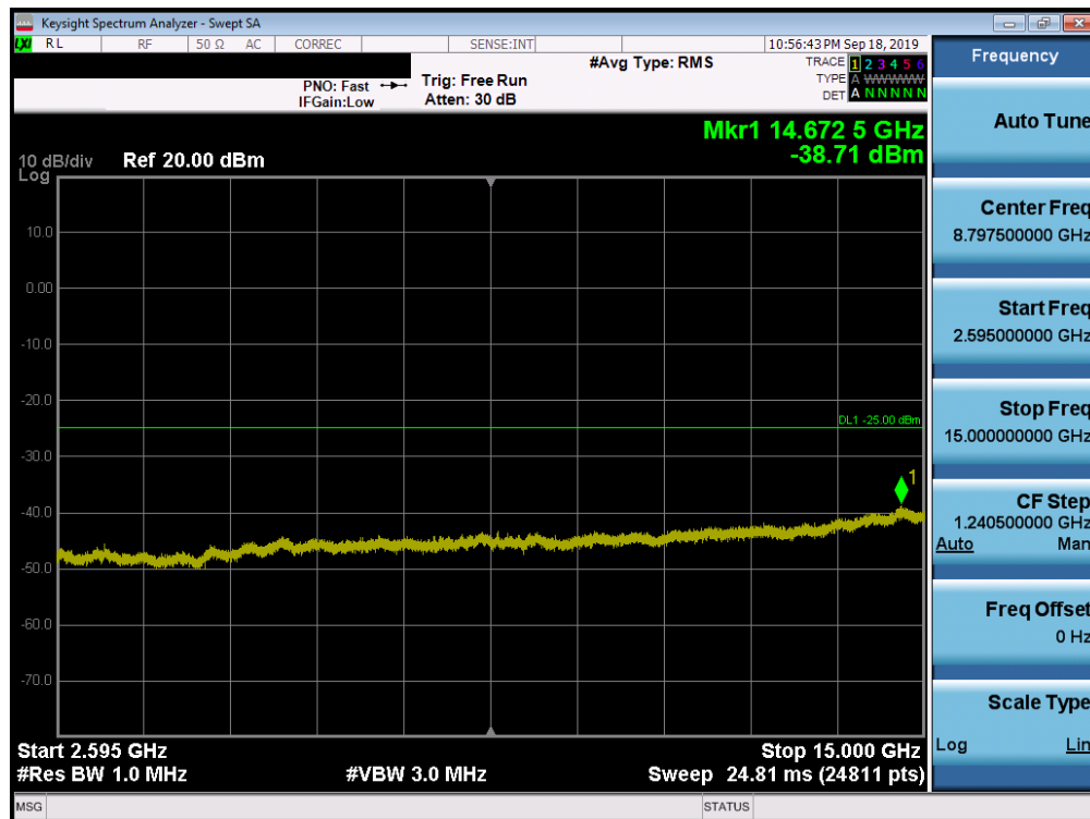
Plot 7-161. Conducted Spurious Plot (Band 7 - 20.0MHz QPSK - RB Size 1, RB Offset 0 - High Channel)
