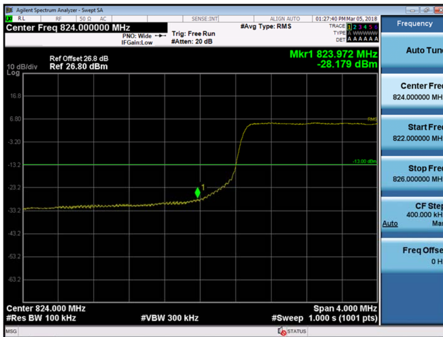
BAND 5. Lower Band Edge Plot (10M BW Ch.20450 QPSK_RB50_Offset 0)
