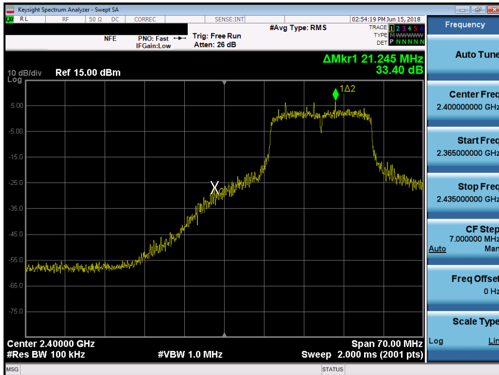
Plot 7-28. Band Edge Plot (802.11n (2.4GHz) – Ch. 2)
