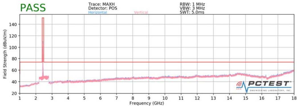
Plot 7-38. Radiated Spurious Plot above 1GHz (802.11b – Ch. 6)
