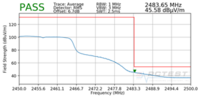
Plot 7-45. Radiated Restricted Upper Band Edge Measurement (Average)
