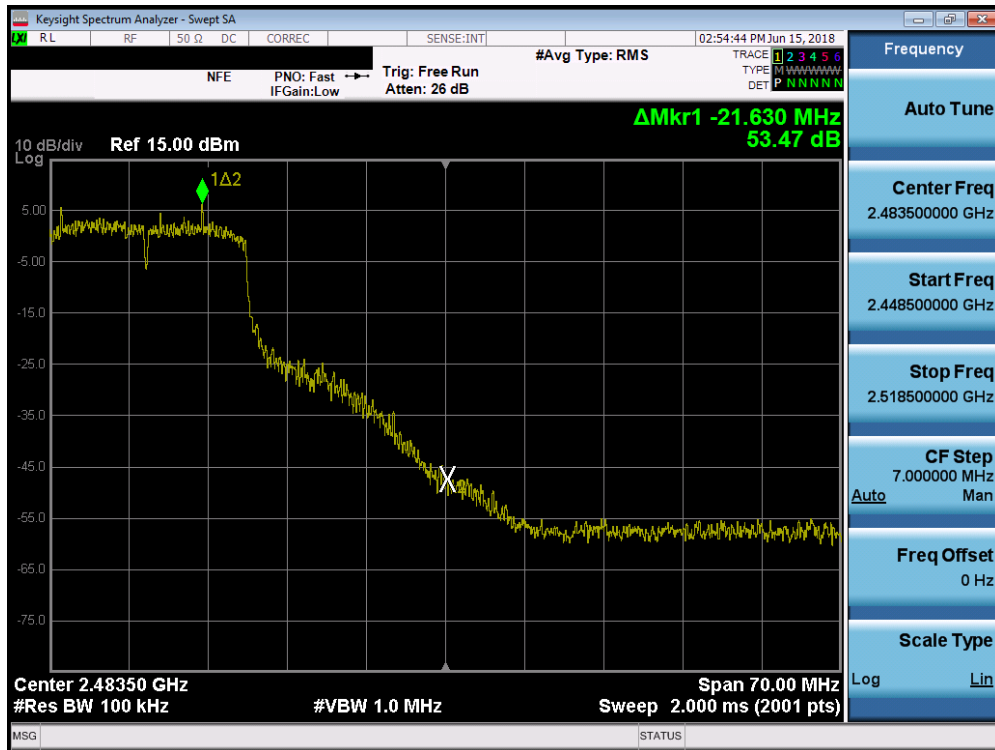
Plot 7-29. Band Edge Plot (802.11n (2.4GHz) – Ch. 10)
