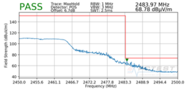
Plot 7-46. Radiated Restricted Upper Band Edge Measurement (Peak)
