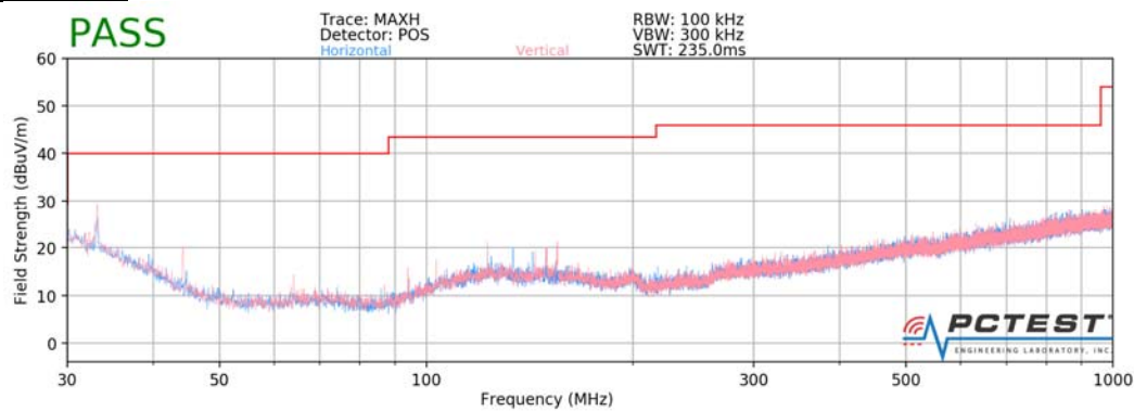
Plot 7-49. Radiated Spurious Plot below 1GHz
