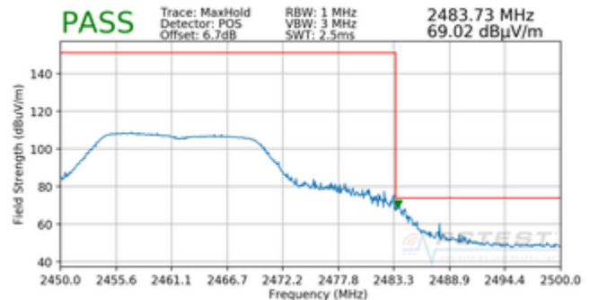
Plot 7-48. Radiated Restricted Upper Band Edge Measurement (Peak)
