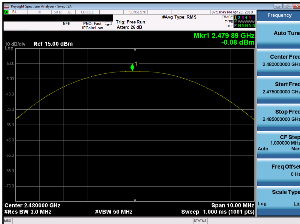
Plot 7-6. Peak Output Power Plot (Bluetooth (LE) – Ch. 39)
