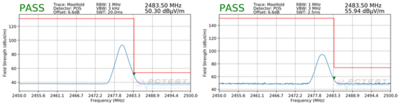
Plot 7-18. Radiated Restricted Upper Band Edge Measurement (Average & Peak)
