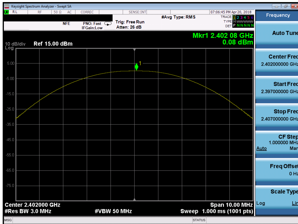
Plot 7-4. Peak Output Power Plot (Bluetooth (LE) – Ch. 0)
