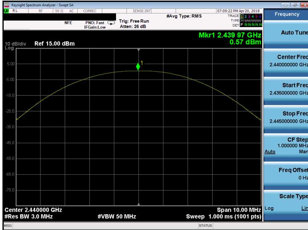
Plot 7-5. Peak Output Power Plot (Bluetooth (LE) – Ch. 19)
