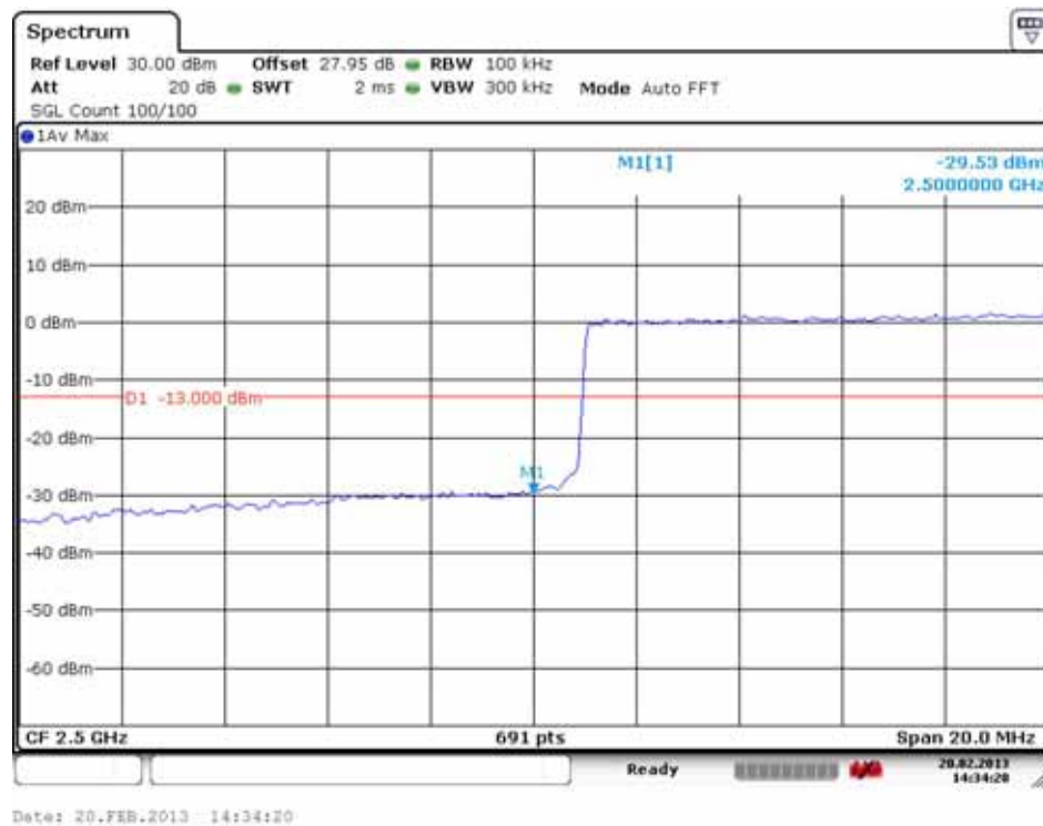
Low Band Edge Plot (20850 ch_20 MHz_QPSK_RB 100_0)
