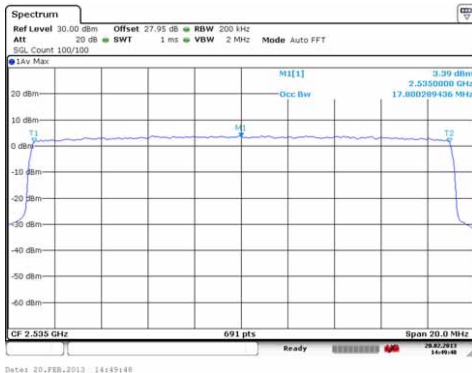
Occupied Bandwidth Plot (21100 ch_20 MHz_16-Q`AM_RB 100)
