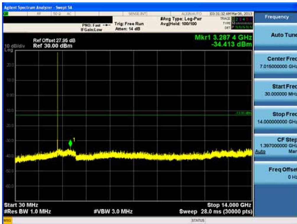
Conducted Spurious Plot_1 (21100 ch_5 MHz_QPSK_RB 1_0) -1
