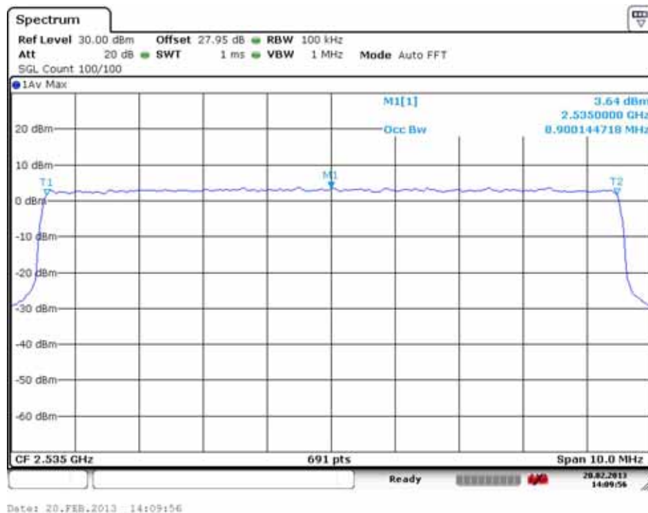
Occupied Bandwidth Plot (21100 ch_10 MHz_16-QAM_RB 50)
