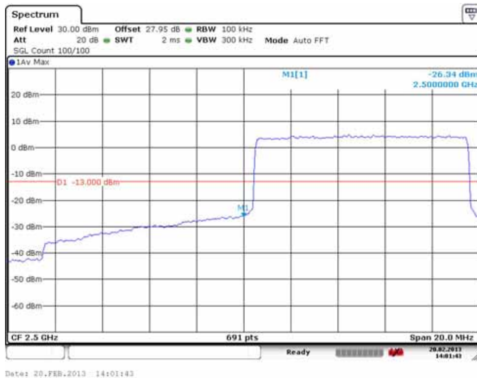
Low Band Edge Plot (20800 ch_10 MHz_QPSK_RB 50_0)
