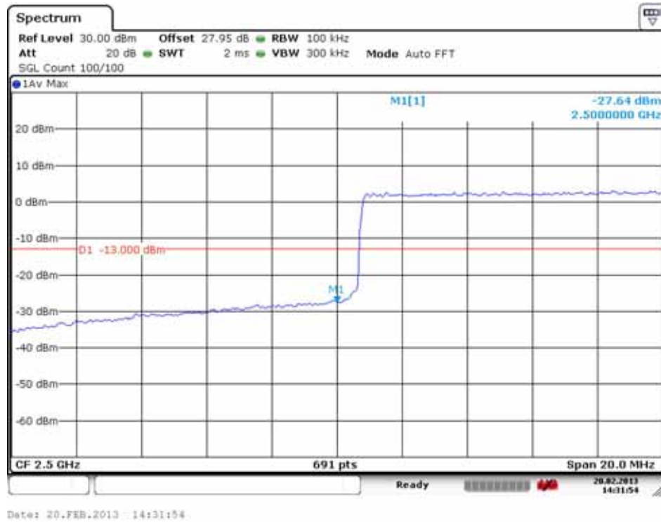
Low Band Edge Plot (20825 ch_15 MHz_QPSK_RB 75_0)
