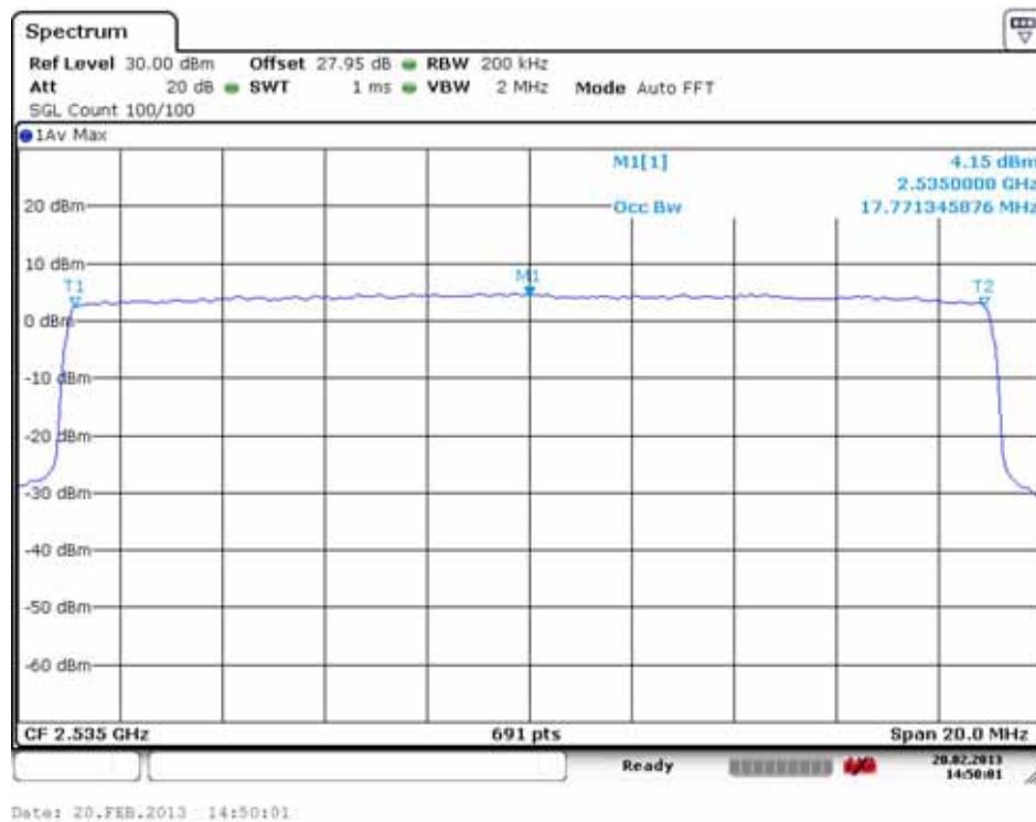
Occupied Bandwidth Plot (21100 ch_20 MHz_QPSK_RB 100)
