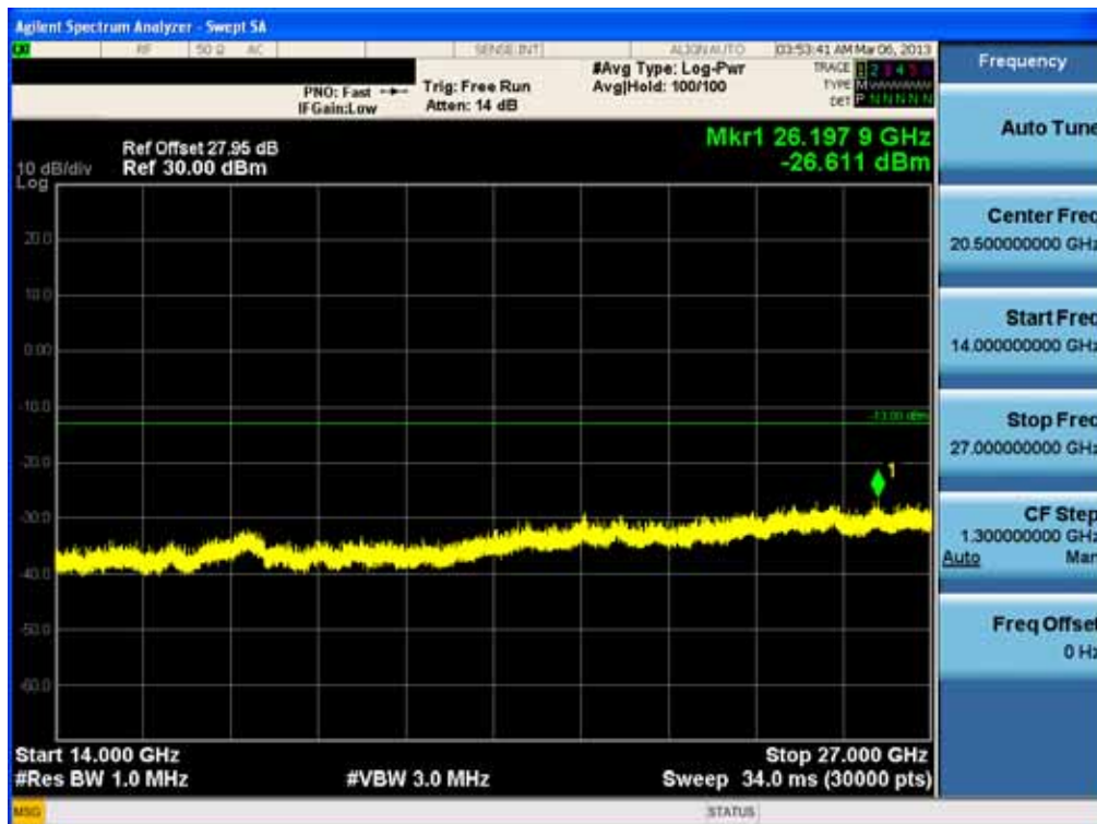
Conducted Spurious Plot_2 (21100 ch_5 MHz_QPSK_RB 1_0) -2
