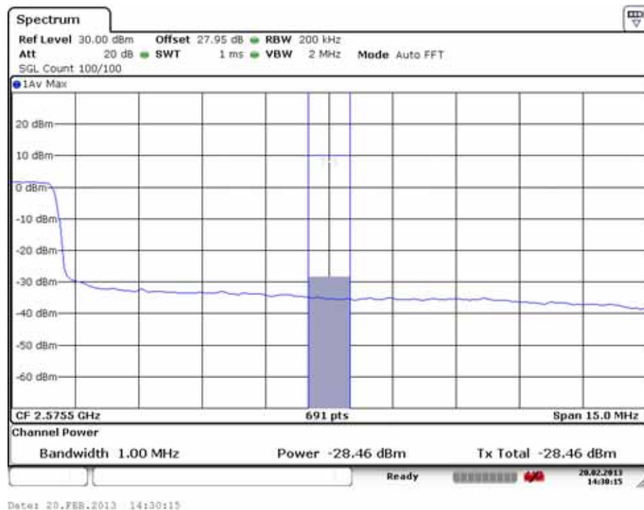
High Extended Band Edge Plot (21350 ch_20 MHz_QPSK_RB 100_0)
