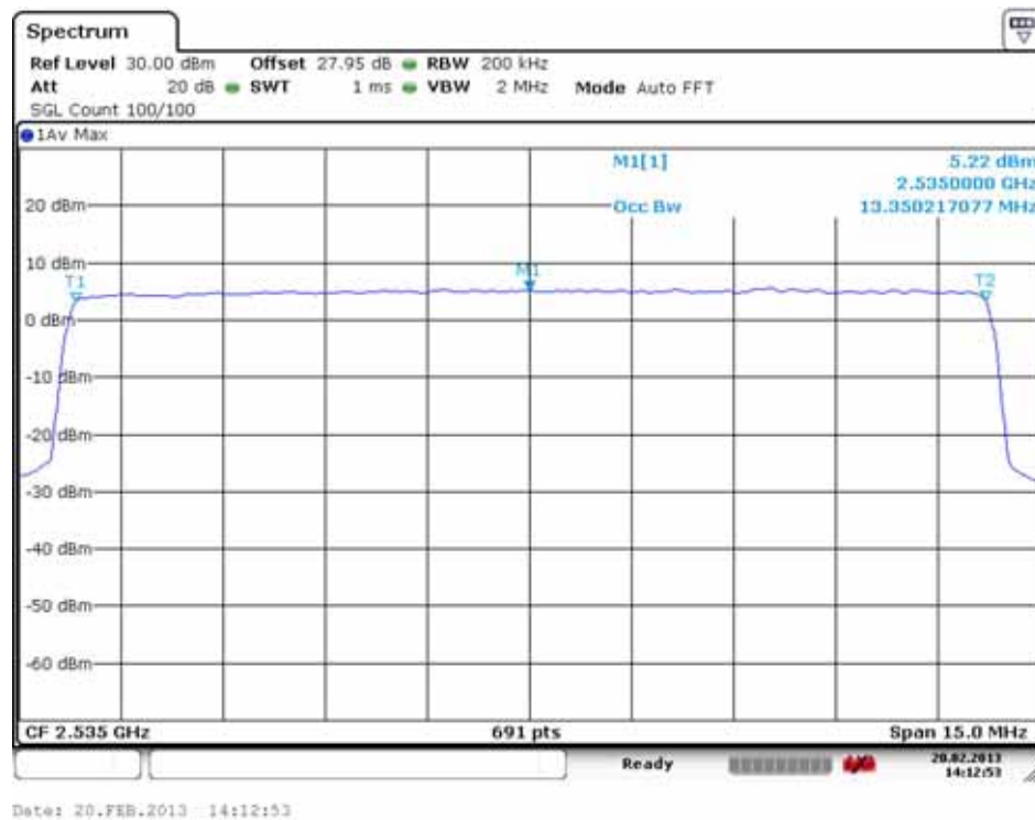
Occupied Bandwidth Plot (21100 ch_15 MHz_QPSK_RB Size 75)
