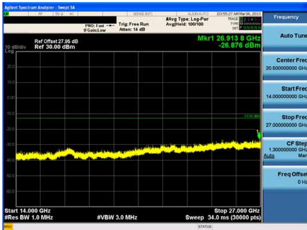
Conducted Spurious Plot_2 (21425 ch_5 MHz_QPSK_RB 1_0) -2
