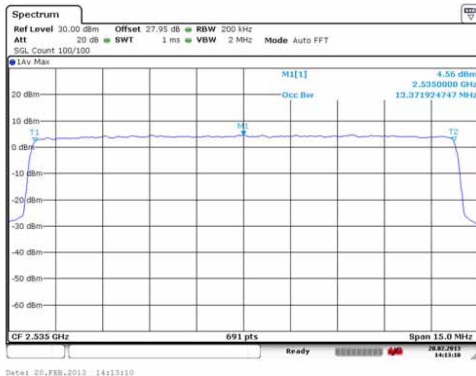
Occupied Bandwidth Plot (21100 ch_15 MHz_16-QAM_RB 75)
