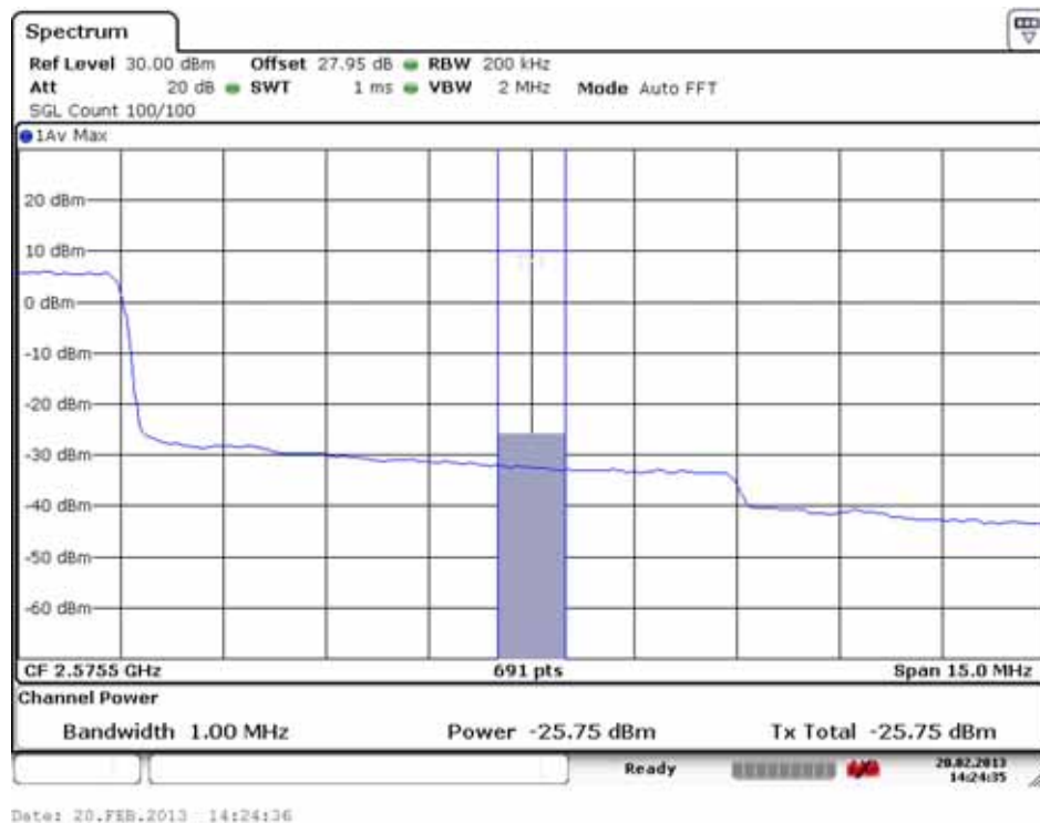
High Extended Band Edge Plot (21400 ch_10 MHz_QPSK_RB 50_0)
