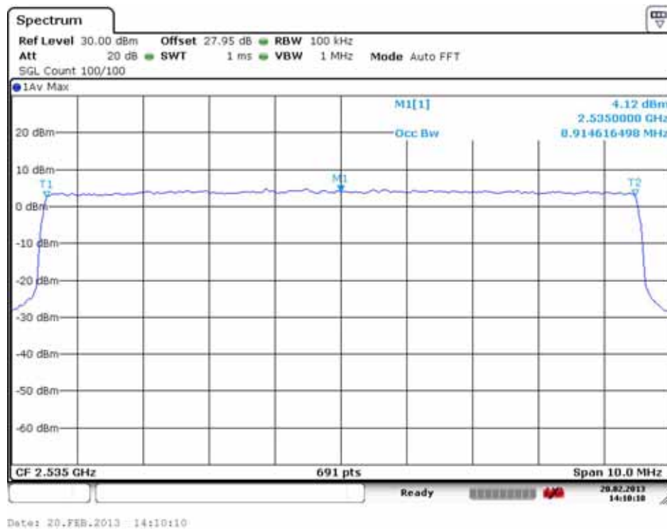
Occupied Bandwidth Plot (21100 ch_10 MHz_QPSK_RB 50)
