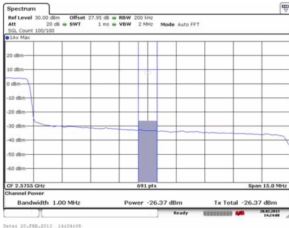
High Extended Band Edge Plot (21375 ch_15 MHz_QPSK_RB 75_0)
