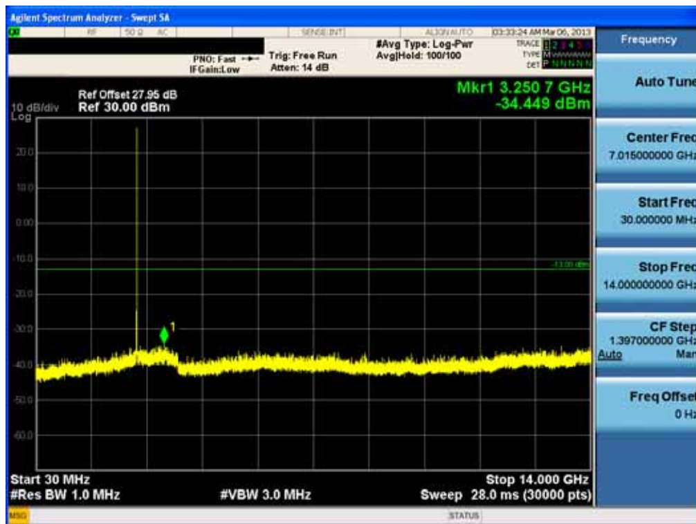
Conducted Spurious Plot_1 (21425 ch_5 MHz_QPSK_RB 1_0) -1
