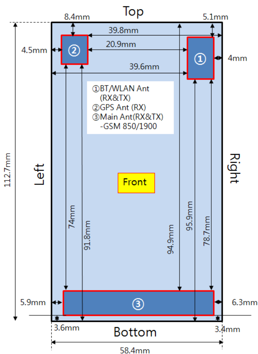
Figure 12.1 Identification of Sides for SAR Testing
