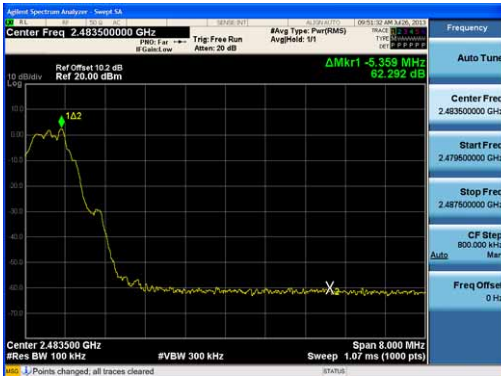
BandEdge (High-CH 39)
