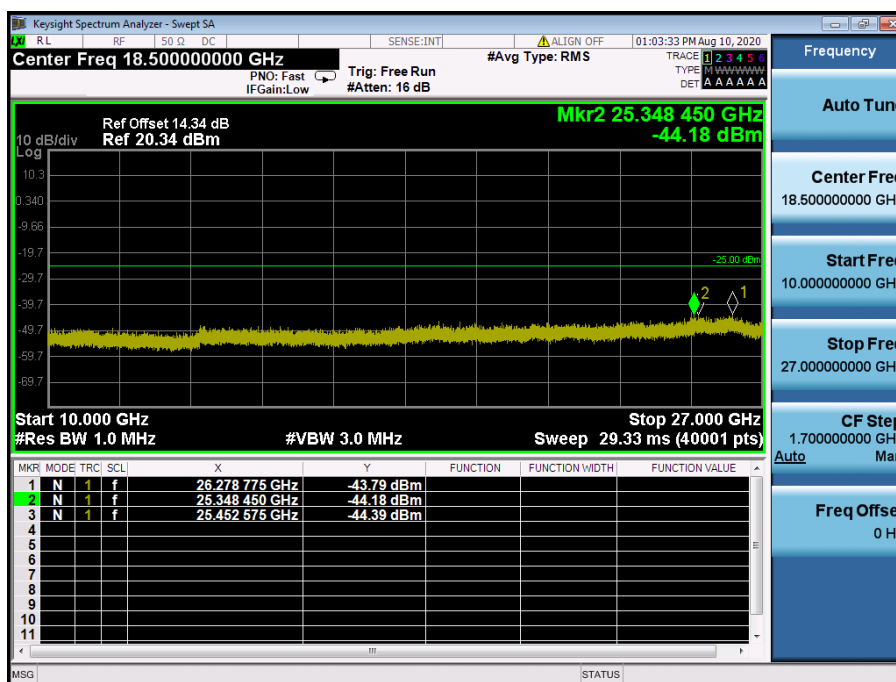
LTE Band 41 / 10 MHz / QPSK - RB Size/Offset (1/0) – Mid Channel
