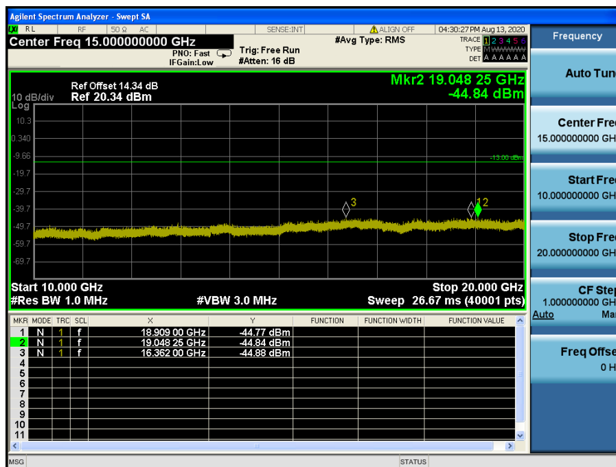
LTE Band 4 / 1.4 MHz / QPSK - RB Size/Offset (3/2) – Low Channel
