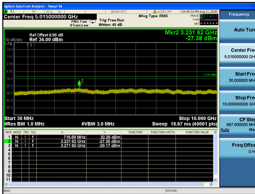
LTE Band 12 / 1.4 MHz / 16QAM - RB Size/Offset (1/2) – High Channel
