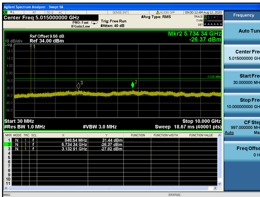
LTE Band 5 / 1.4 MHz / QPSK - RB Size/Offset (1/2) – High Channel
