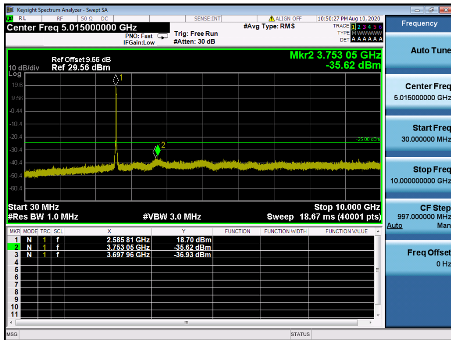
LTE Band 41 / 20 MHz / 64QAM - RB Size/Offset (100/0) – Mid Channel
