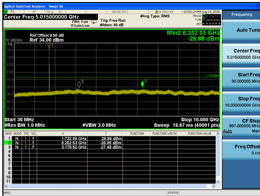
LTE Band 4 / 10 MHz / 64QAM - RB Size/Offset (1/25) – Mid Channel
