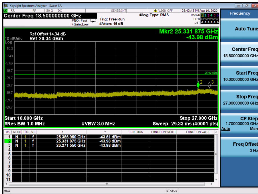
LTE Band 41 / 15 MHz / 16QAM - RB Size/Offset (1/36) – Low Channel
