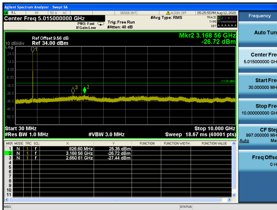
LTE Band 5 / 10 MHz / 64QAM - RB Size/Offset (25/0) – Low Channel
