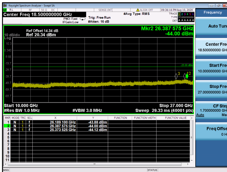
LTE Band 41 / 15 MHz / 64QAM - RB Size/Offset (1/0) – Mid Channel
