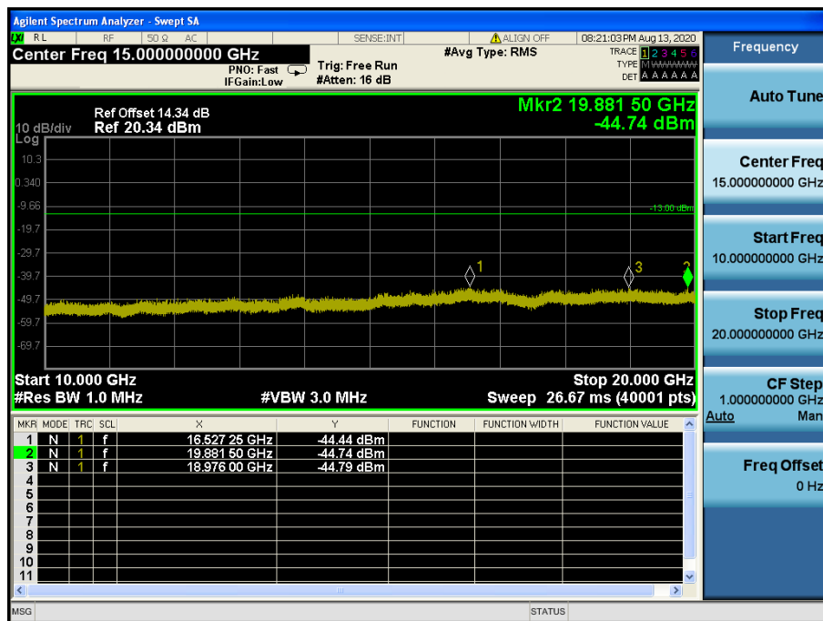
LTE Band 4 / 20 MHz / QPSK - RB Size/Offset (1/0) – Mid Channel
