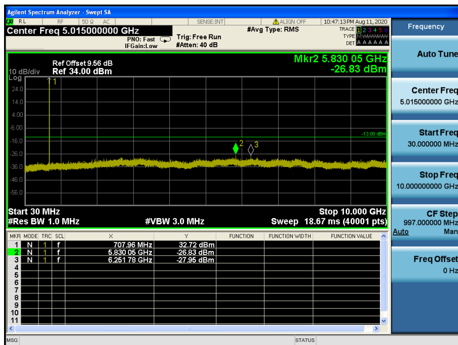
LTE Band 12 / 3 MHz / 64QAM - RB Size/Offset (1/7) – Mid Channel
