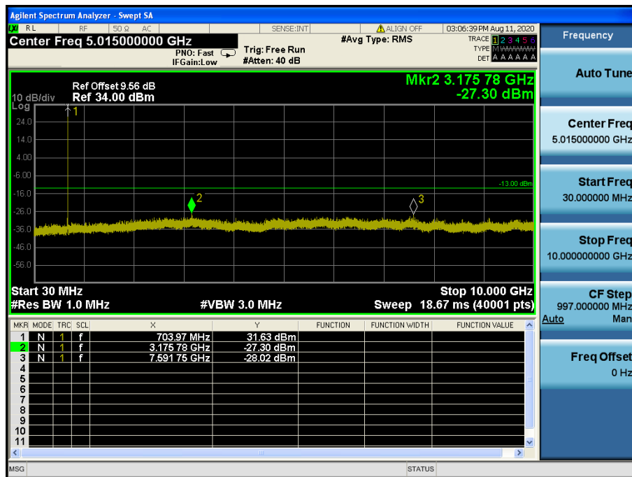
LTE Band 12 / 5 MHz / QPSK - RB Size/Offset (1/24) – Low Channel
