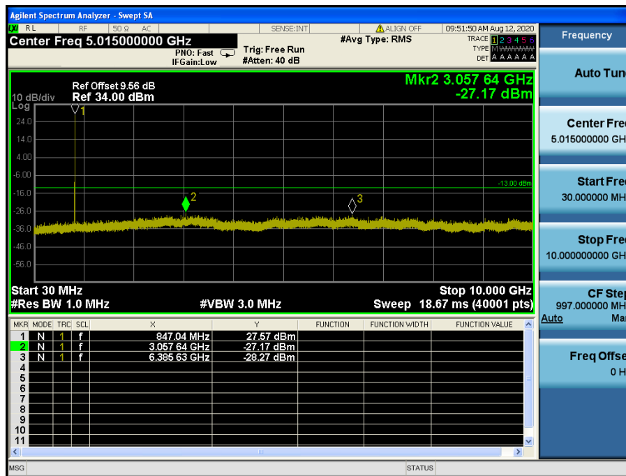
LTE Band 5 / 3 MHz / QPSK - RB Size/Offset (15/0) – High Channel
