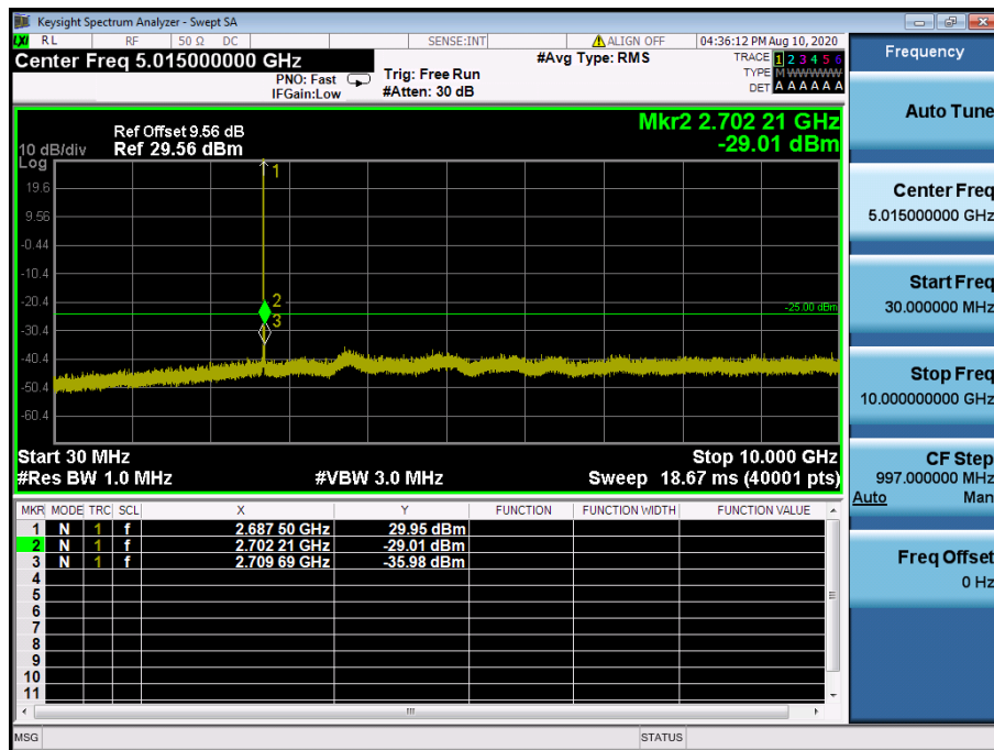
LTE Band 41 / 5 MHz / 16QAM - RB Size/Offset (1/12) – High Channel
