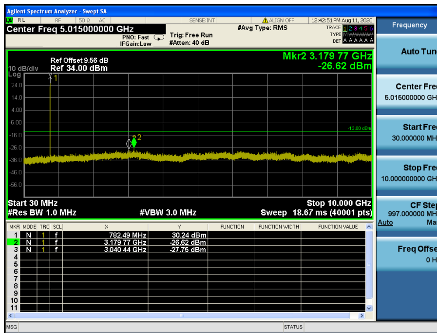
LTE Band 13 / 10 MHz / 64QAM - RB Size/Offset (1/25) – Low Channel
