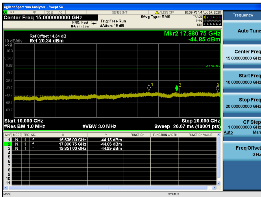
LTE Band 4 / 5 MHz / 16QAM - RB Size/Offset (12/0) – Low Channel
