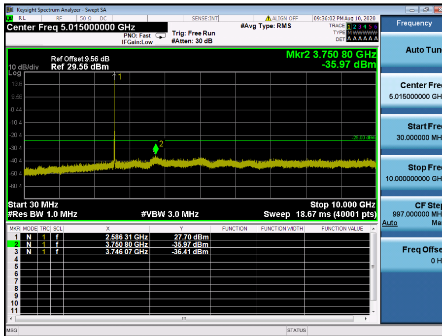
LTE Band 41 / 15 MHz / 64QAM - RB Size/Offset (1/0) – Mid Channel
