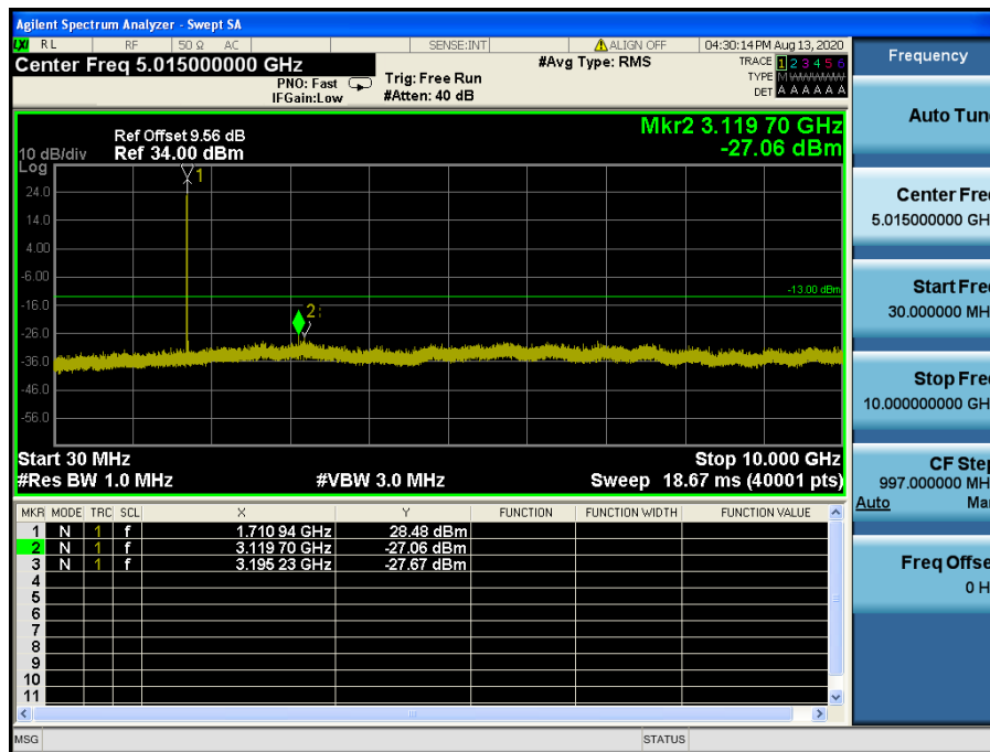
LTE Band 4 / 1.4 MHz / QPSK - RB Size/Offset (3/2) – Low Channel
