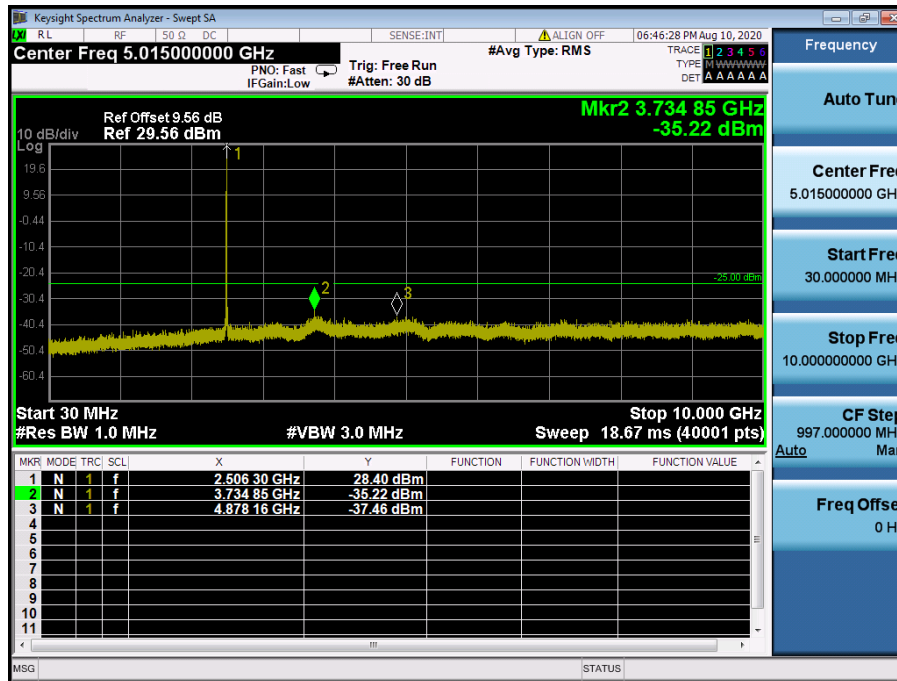
LTE Band 41 / 20 MHz / 16QAM - RB Size/Offset (1/50) – Low Channel
