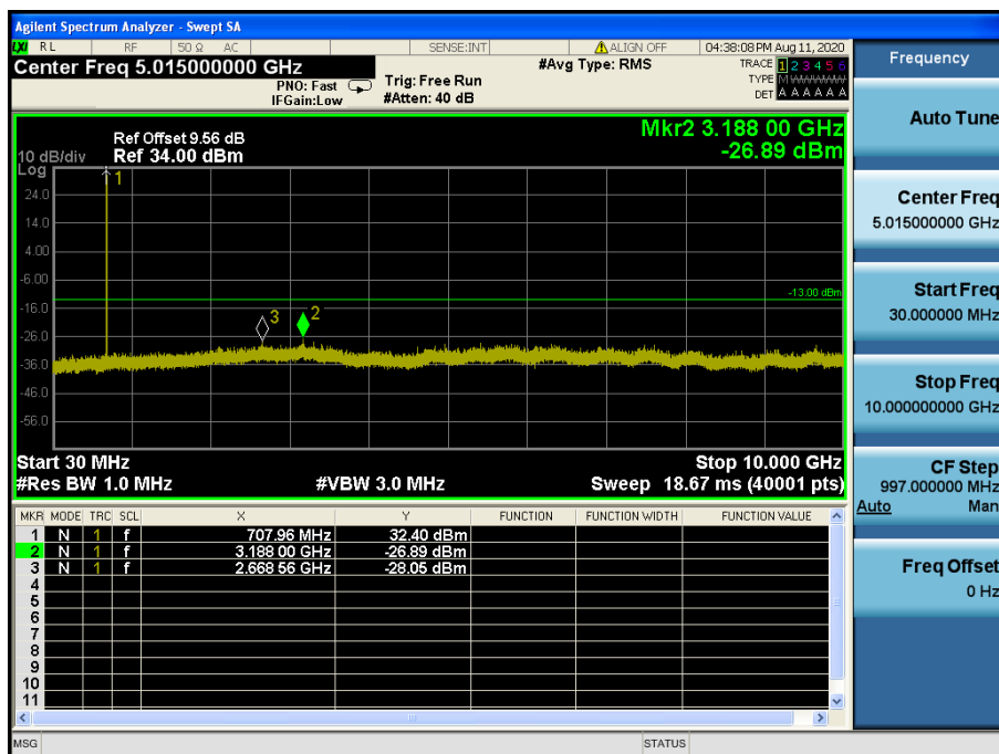
LTE Band 12 / 1.4 MHz / 16QAM - RB Size/Offset (1/2) – Mid Channel
