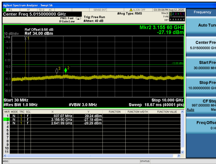
LTE Band 5 / 1.4 MHz / 64QAM - RB Size/Offset (6/0) – Mid Channel
