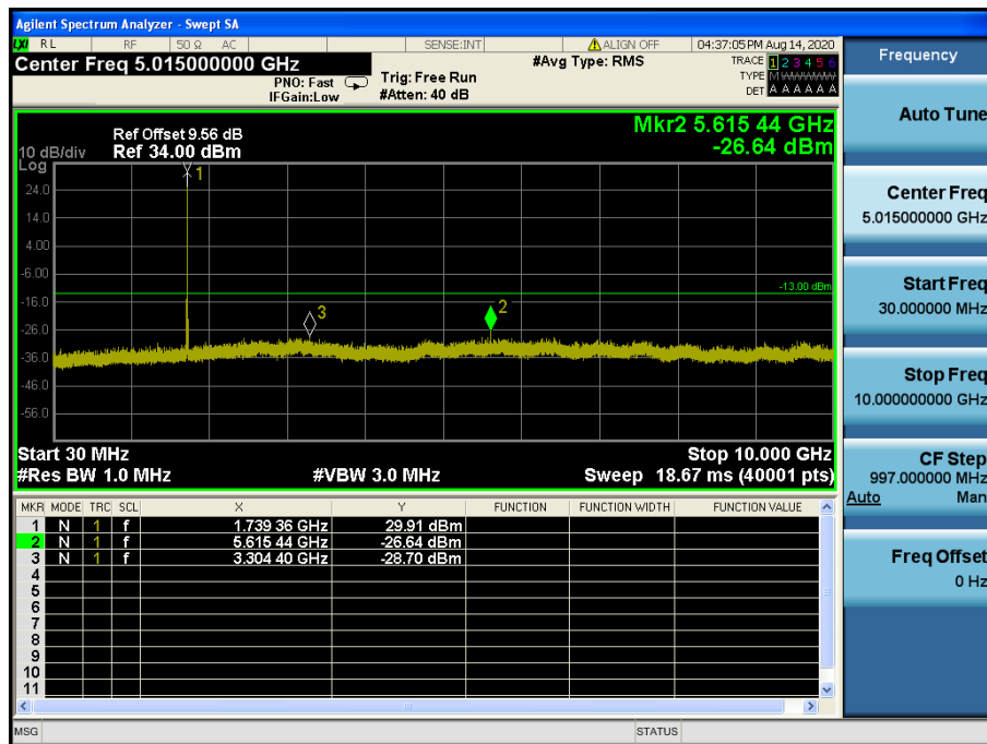
LTE Band 4 / 15 MHz / 64QAM - RB Size/Offset (1/74) – Mid Channel
