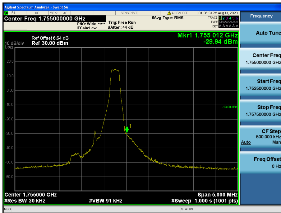
LTE Band 4 / 1.4 MHz / 64QAM - RB Size/Offset (1/5)
