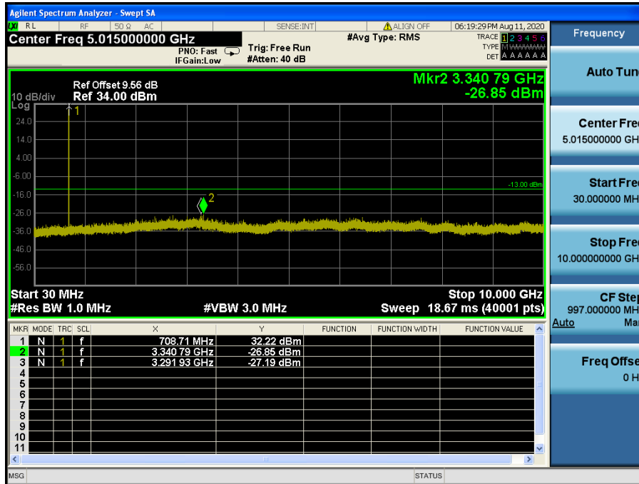
LTE Band 12 / 10 MHz / 16QAM - RB Size/Offset (1/49) – Low Channel
