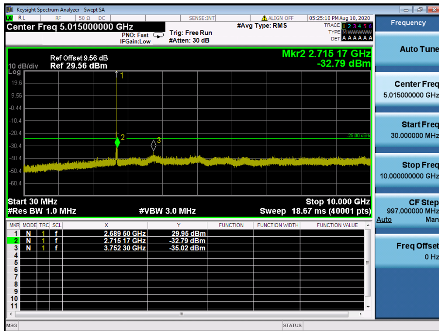
LTE Band 41 / 10 MHz / 16QAM - RB Size/Offset (1/49) – High Channel
