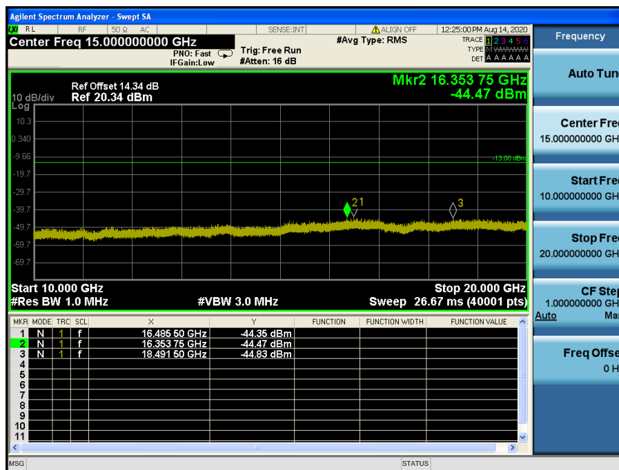
LTE Band 4 / 20 MHz / 16QAM - RB Size/Offset (50/0) – Low Channel
