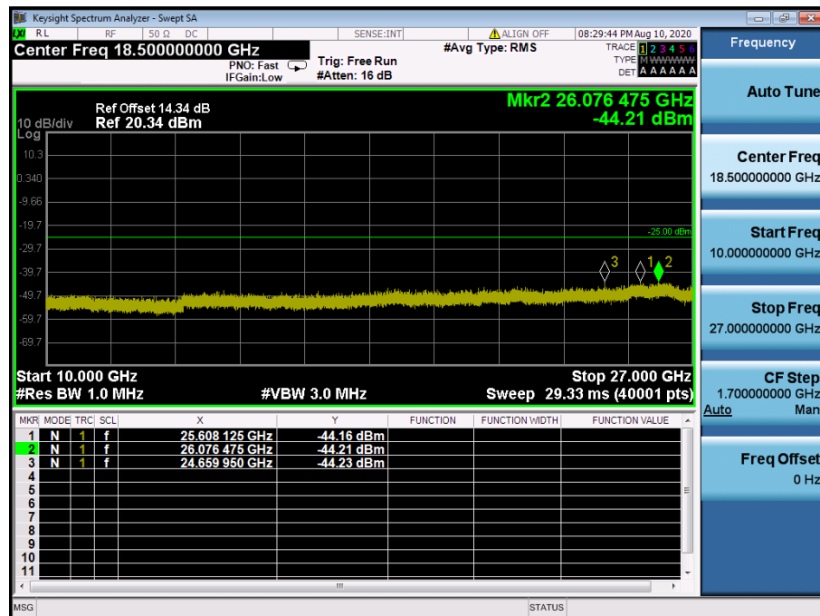
LTE Band 41 / 10 MHz / 64QAM - RB Size/Offset (1/49) – Low Channel
