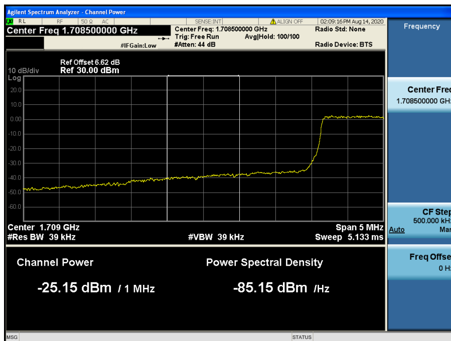
LTE Band 4 / 3 MHz / 64QAM - RB Size/Offset (15/0)
