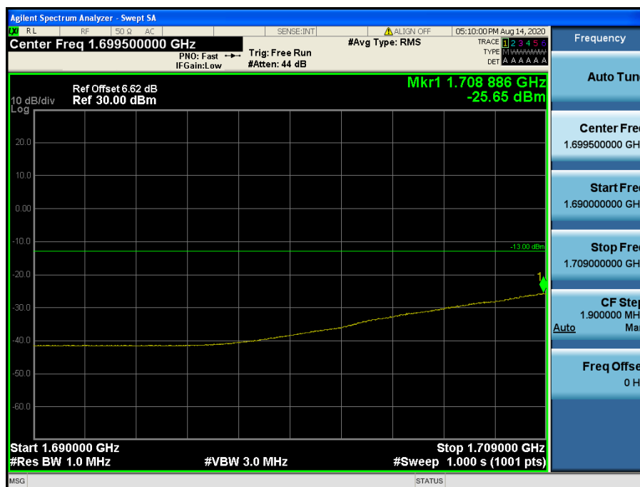
LTE Band 4 / 20 MHz / 64QAM - RB Size/Offset (50/0)
