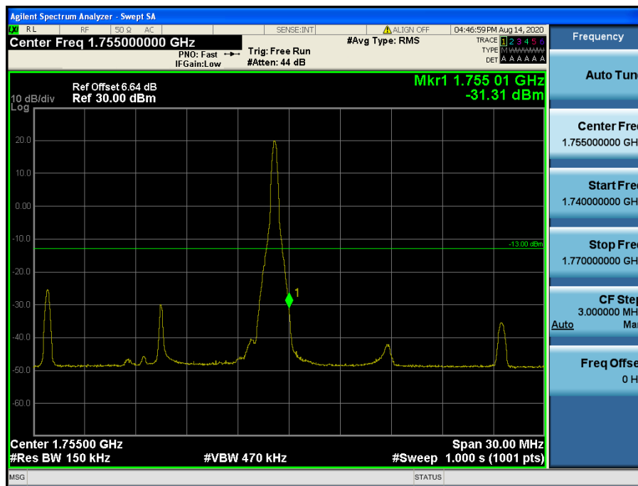
LTE Band 4 / 15 MHz / 64QAM - RB Size/Offset (36/39)
