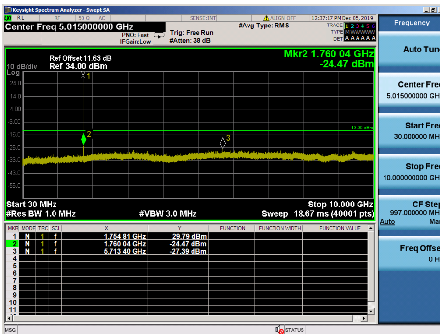
LTE Band 4 / 1.4MHz / 16QAM - RB Size/Offset (3/3) – High Channel
