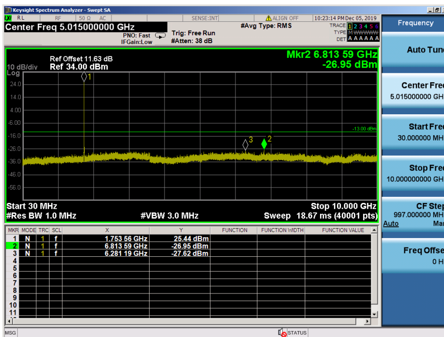
LTE Band 4 / 5MHz / 64QAM - RB Size/Offset (12/13) – High Channel
