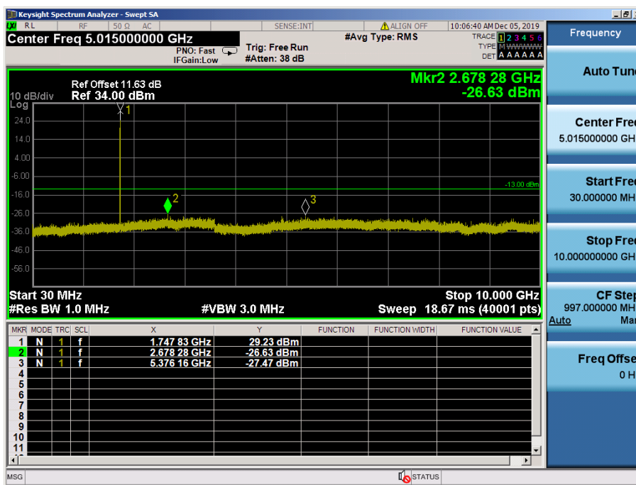
LTE Band 4 / 15MHz / QPSK - RB Size/Offset (1/36) – High Channel
