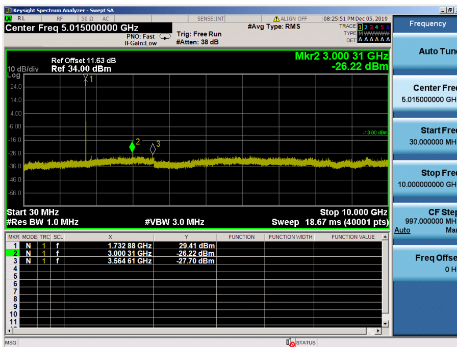
LTE Band 4 / 1.4MHz / 64QAM - RB Size/Offset (1/2) – Mid Channel
