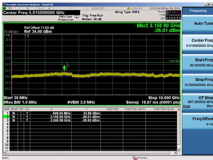
LTE Band 5 / 1.4MHz / 64QAM - RB Size/Offset (1/5) – High Channel
