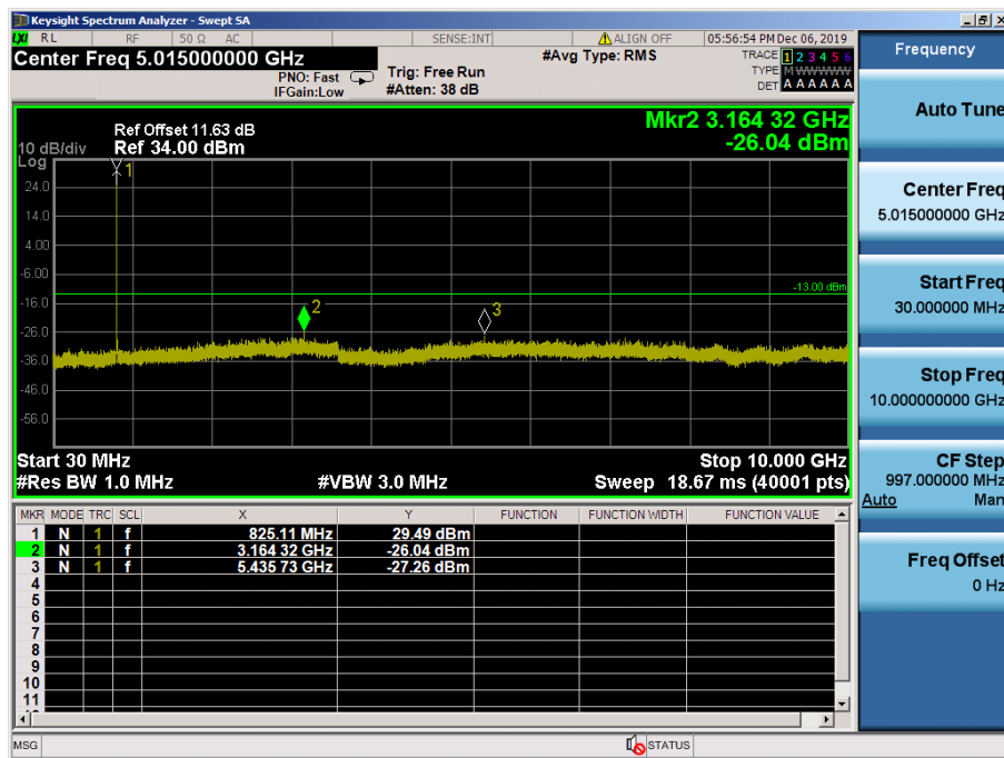
LTE Band 5 / 3MHz / 64QAM - RB Size/Offset (8/0) – Low Channel
