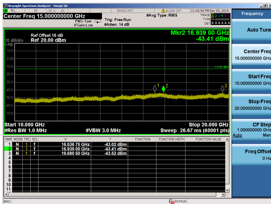
LTE Band 4 / 15MHz / 64QAM - RB Size/Offset (1/74)–Low Channel
