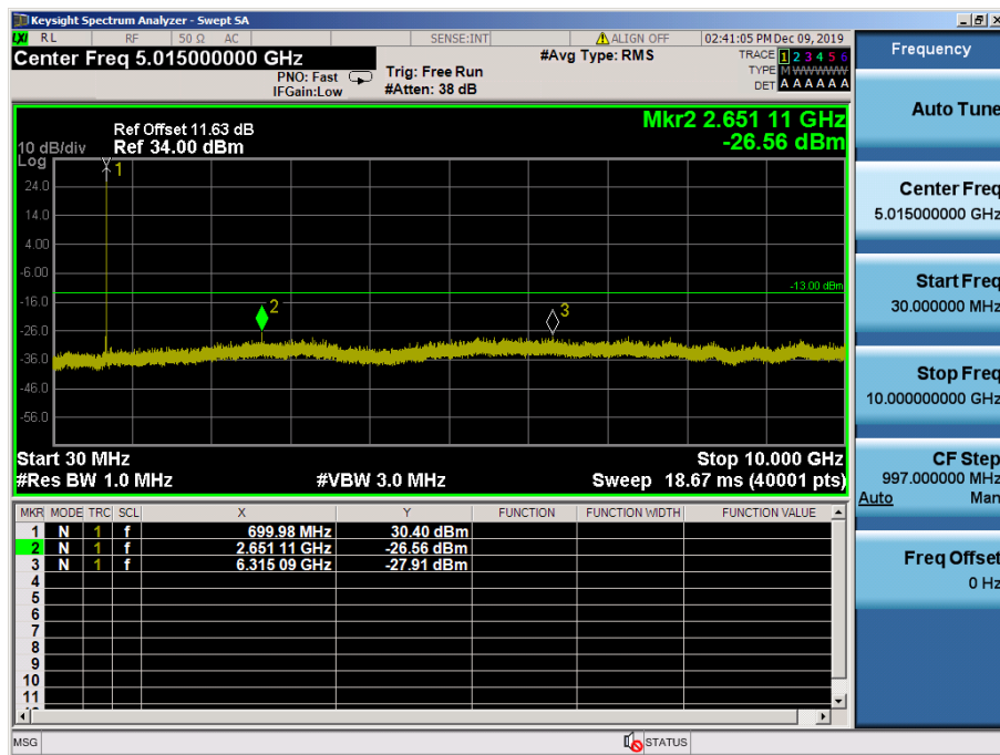
LTE Band 12 / 1.4MHz / 64QAM - RB Size/Offset (6/0) – Low Channel
