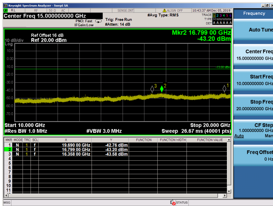
LTE Band 4 / 20MHz / QPSK - RB Size/Offset (50/50)–Mid Channel
