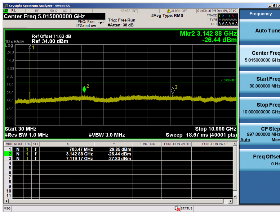
LTE Band 12, 17 / 5MHz / 16QAM - RB Size/Offset (12/13) – Low Channel
