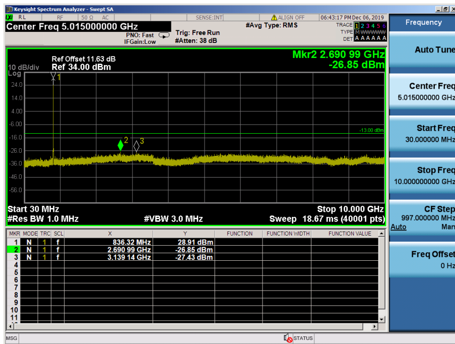
LTE Band 5 / 5MHz / 64QAM - RB Size/Offset (12/0) – Mid Channel
