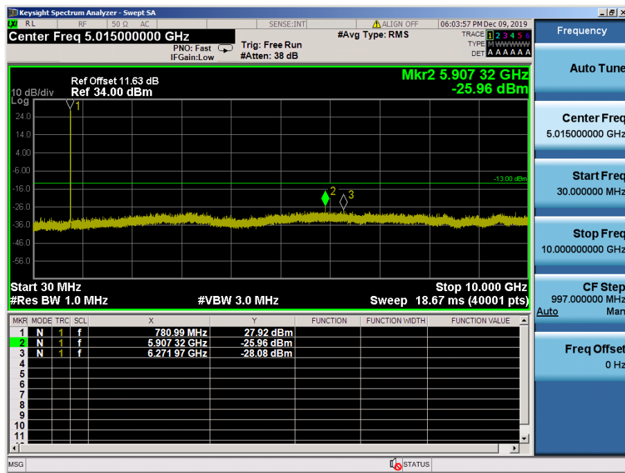
LTE Band 13 / 10MHz / QPSK - RB Size/Offset (25/12) – Low Channel
