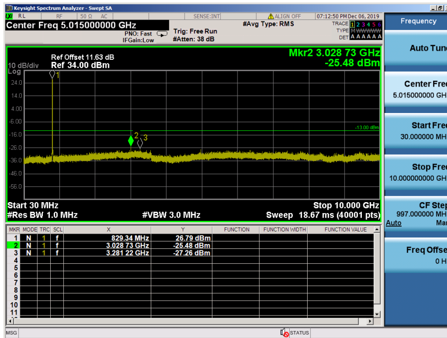
LTE Band 5 / 10MHz / 64QAM - RB Size/Offset (25/12) – Low Channel
