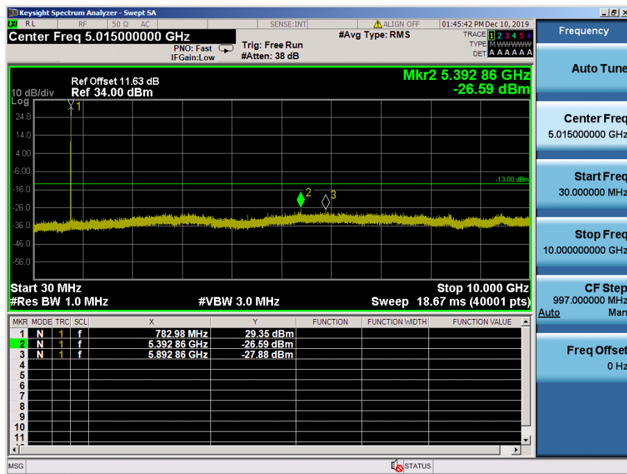
LTE Band 13 / 5MHz / QPSK - RB Size/Offset (12/0) – High Channel
