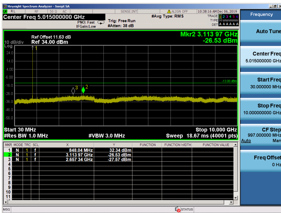
LTE Band 5 / 3MHz / QPSK - RB Size/Offset (1/7) – High Channel
