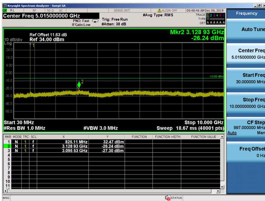
LTE Band 5 / 1.4MHz / QPSK - RB Size/Offset (3/2) – Low Channel
