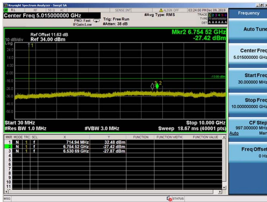
LTE Band 12 / 3MHz / 64QAM - RB Size/Offset (1/7) – High Channel
