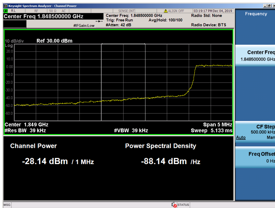
LTE Band 2 / 3MHz / 64QAM - RB Size/Offset (15/0)
