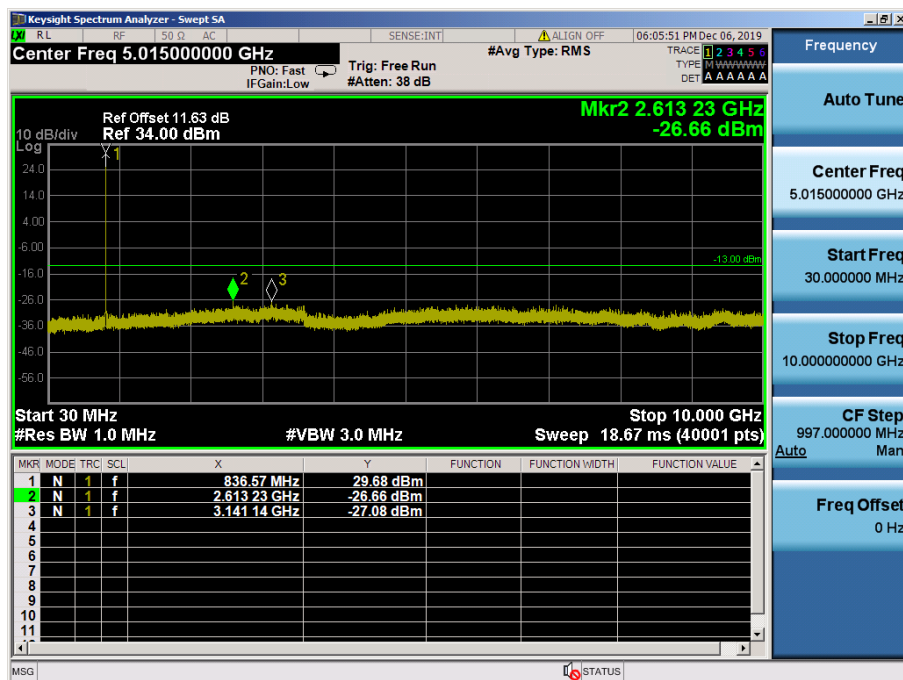
LTE Band 5 / 3MHz / 64QAM - RB Size/Offset (8/0) – Mid Channel
