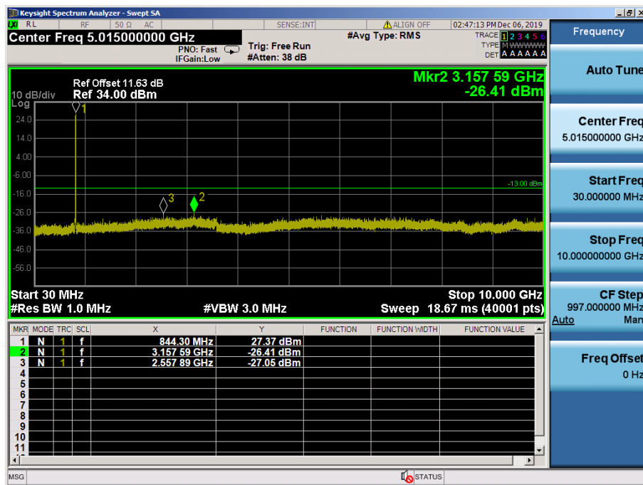
LTE Band 5 / 10MHz / 16QAM - RB Size/Offset (25/12) – High Channel
