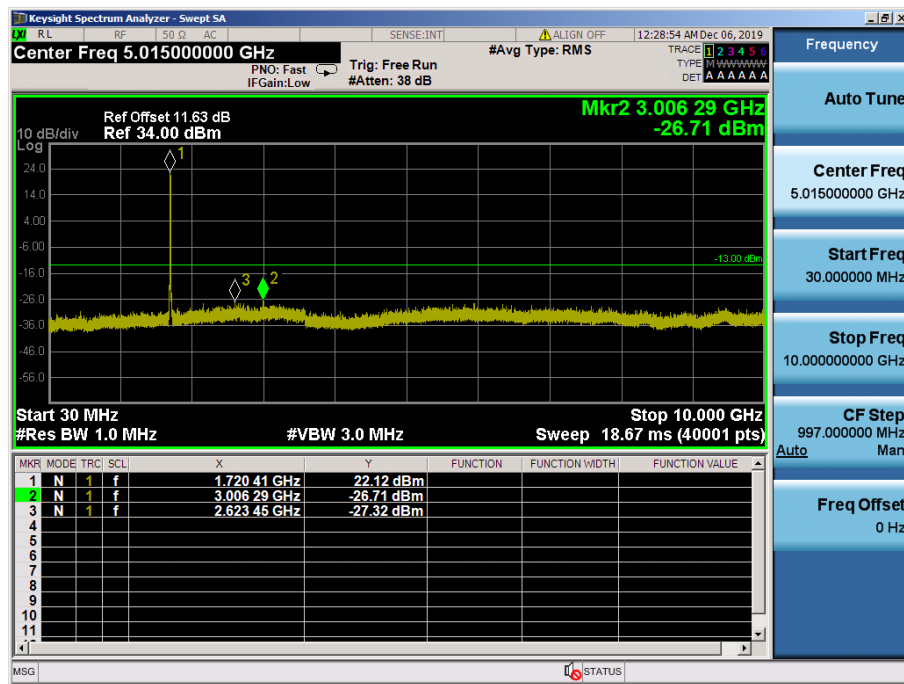
LTE Band 4 / 20MHz / 64QAM - RB Size/Offset (50/25) –Low Channel
