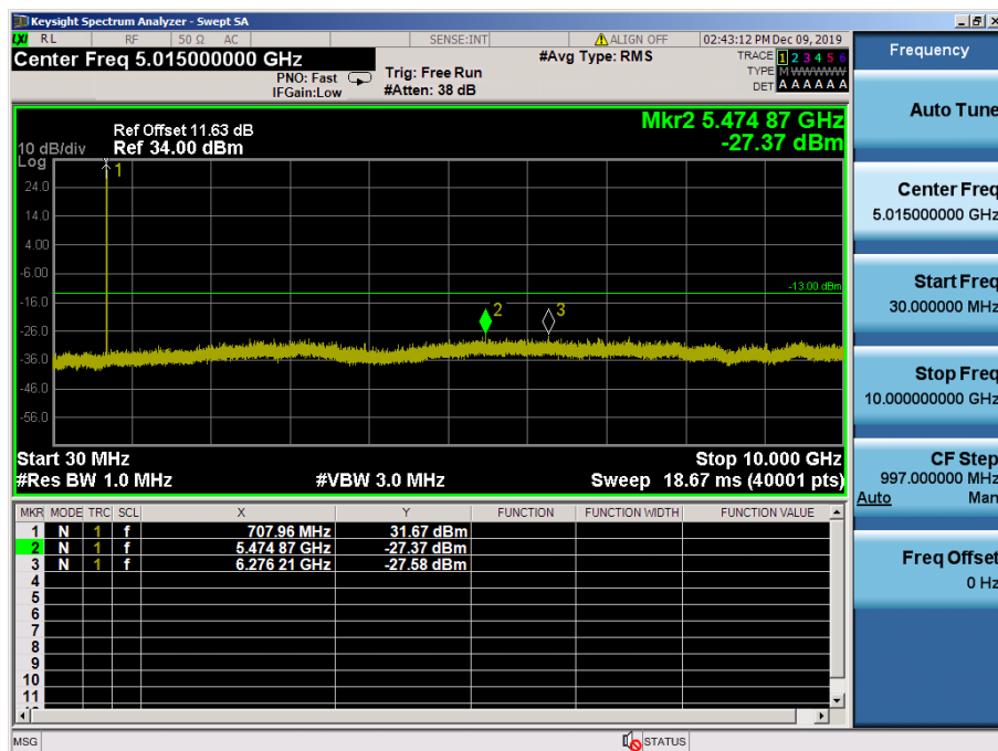
LTE Band 12 / 1.4MHz / 64QAM - RB Size/Offset (3/2) – Mid Channel
