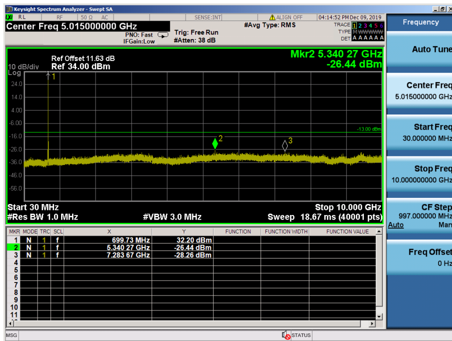
LTE Band 12, 17 / 10MHz / 64QAM - RB Size/Offset (1/0) – Low Channel
