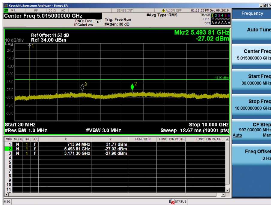
LTE Band 12, 17 / 5MHz / 16QAM - RB Size/Offset (1/12) – High Channel
