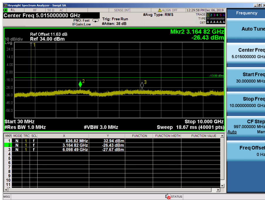
LTE Band 5 / 1.4MHz / 16QAM - RB Size/Offset (3/3) – Mid Channel
