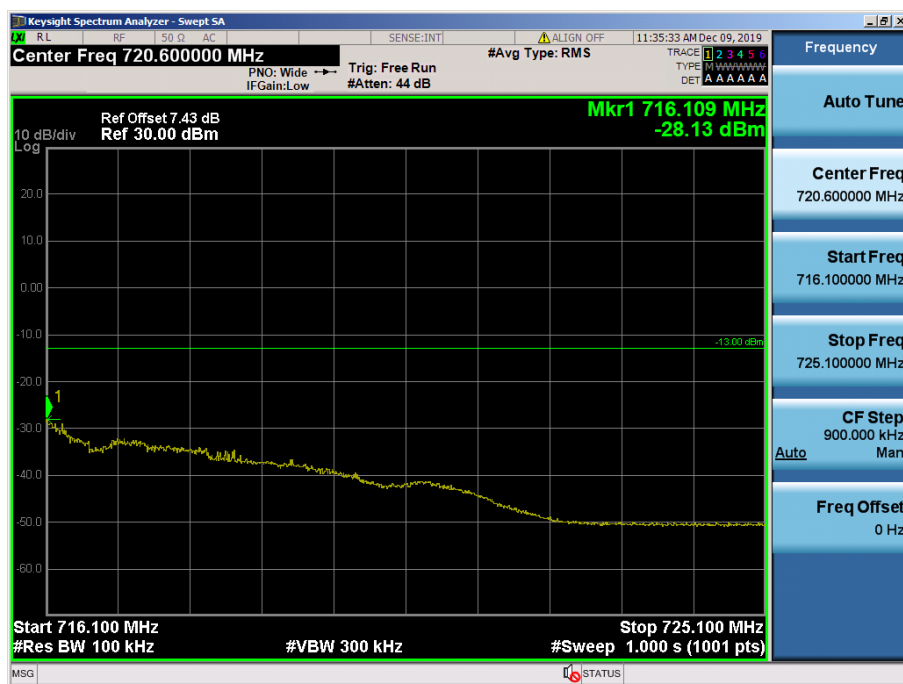
LTE Band 12, 17 / 10MHz / QPSK - RB Size/Offset (25/25)
