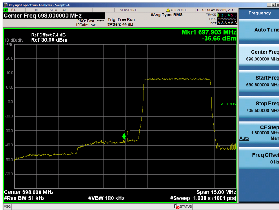
LTE Band 12, 17 / 5MHz / QPSK - RB Size/Offset (25/0)
