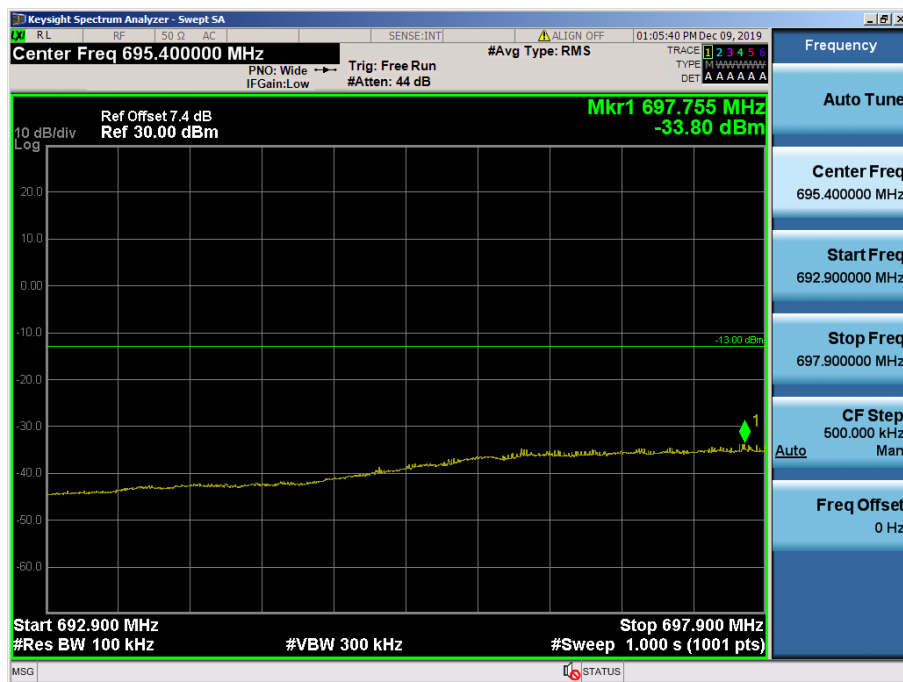
LTE Band 12, 17 / 5MHz / 16QAM - RB Size/Offset (25/0)
