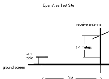
Figure 3-1. Diagram of 3-meter test range
