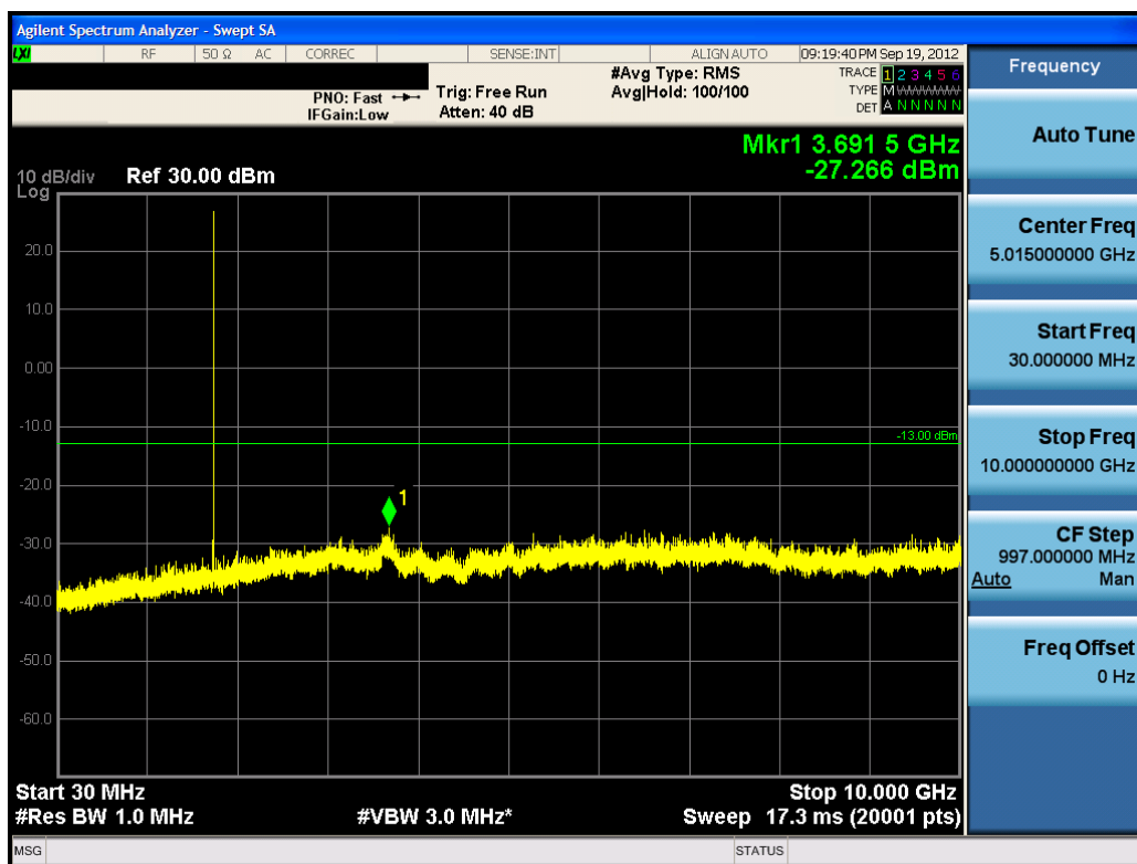
Plot 7-11. Conducted Spurious Plot (QPSK – RB Size 1, RB Offset 0 – High Channel)
