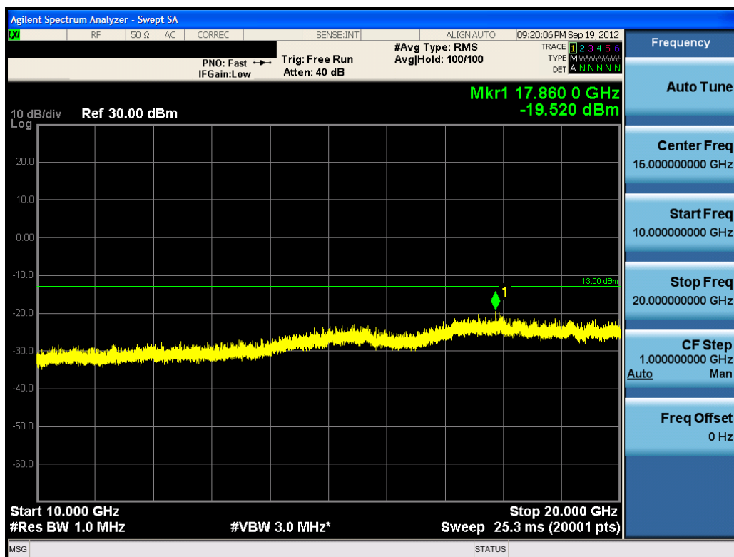
Plot 7-12. Conducted Spurious Plot (QPSK – RB Size 1, RB Offset 0 – High Channel)
