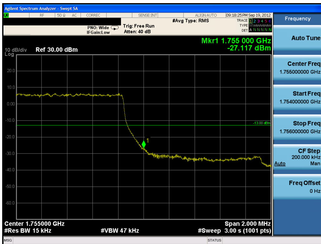
Plot 7-13. Upper Band Edge Plot (QPSK – RB Size 6)
