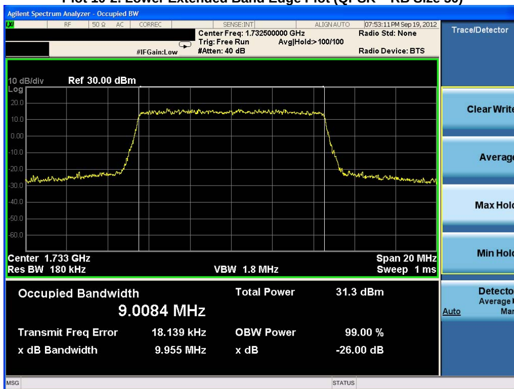
Plot 10-3. Occupied Bandwidth Plot (QPSK – RB Size 50)
