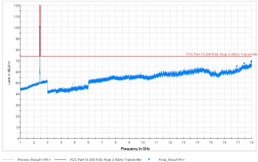
Plot 7-34. Radiated Spurious Plot above 1GHz (802.11b – Ch. 6, Ant. Pol. V)
