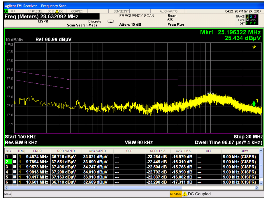
Plot 7-45. Line Conducted Plot with 802.11b (L1)
