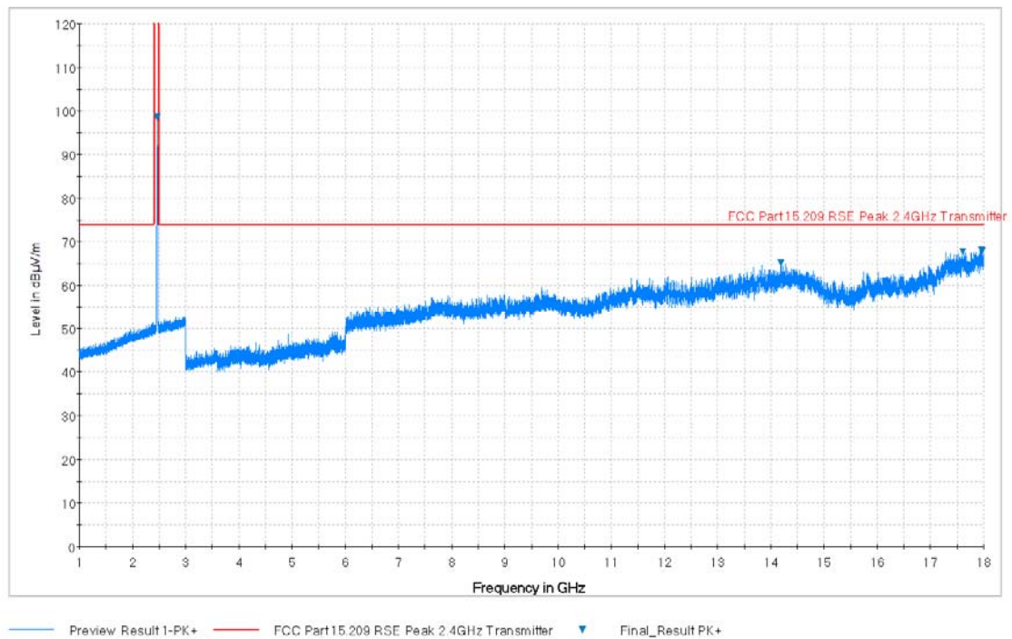
Plot 7-36. Radiated Spurious Plot above 1GHz (802.11b – Ch. 11, Ant. Pol. V)
