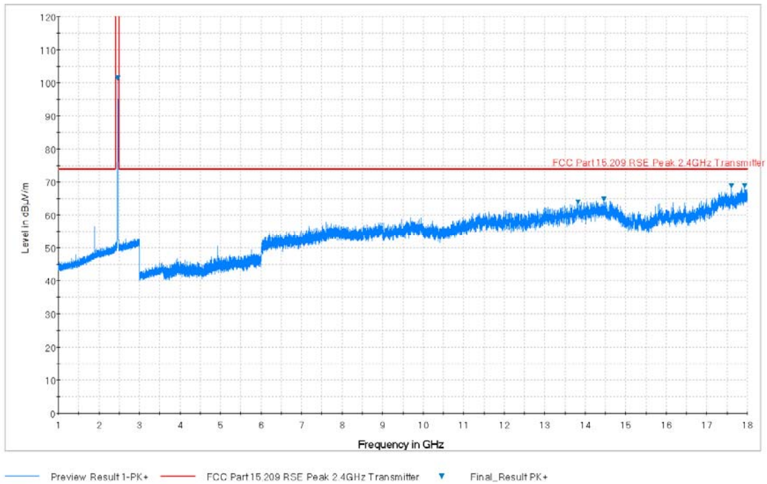
Plot 7-35. Radiated Spurious Plot above 1GHz (802.11b – Ch. 11, Ant. Pol. H)
