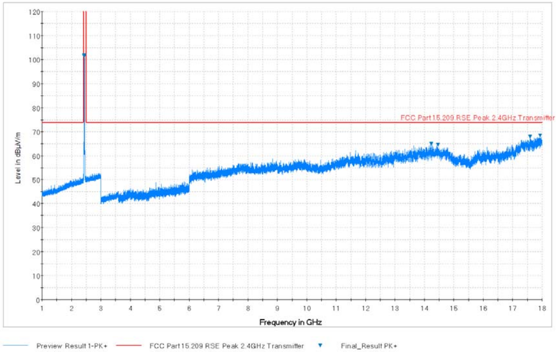
Plot 7-33. Radiated Spurious Plot above 1GHz (802.11b – Ch. 6, Ant. Pol. H)
