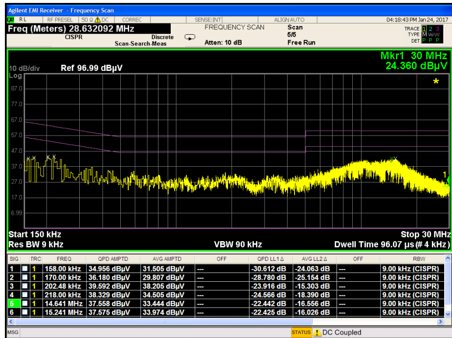
Plot 7-46. Line Conducted Plot with 802.11b (N)
