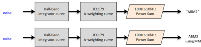
Figure 4-9 ABM2 Validation Block Diagram
