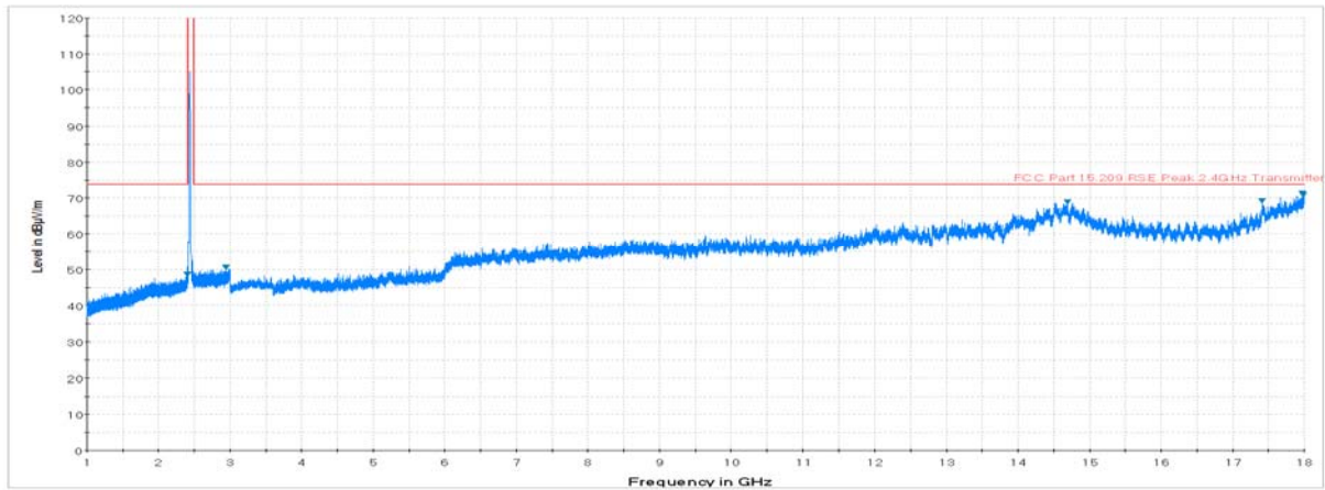
Plot 7-12. Radiated Spurious Plot above 1GHz (802.11b – Ch. 6, Ant. Pol. V)
