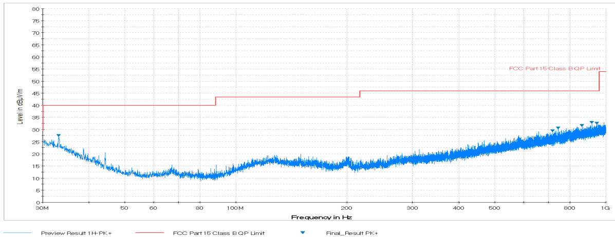
Plot 7-37. Radiated Spurious Plot below 1GHz (Pol. H)
