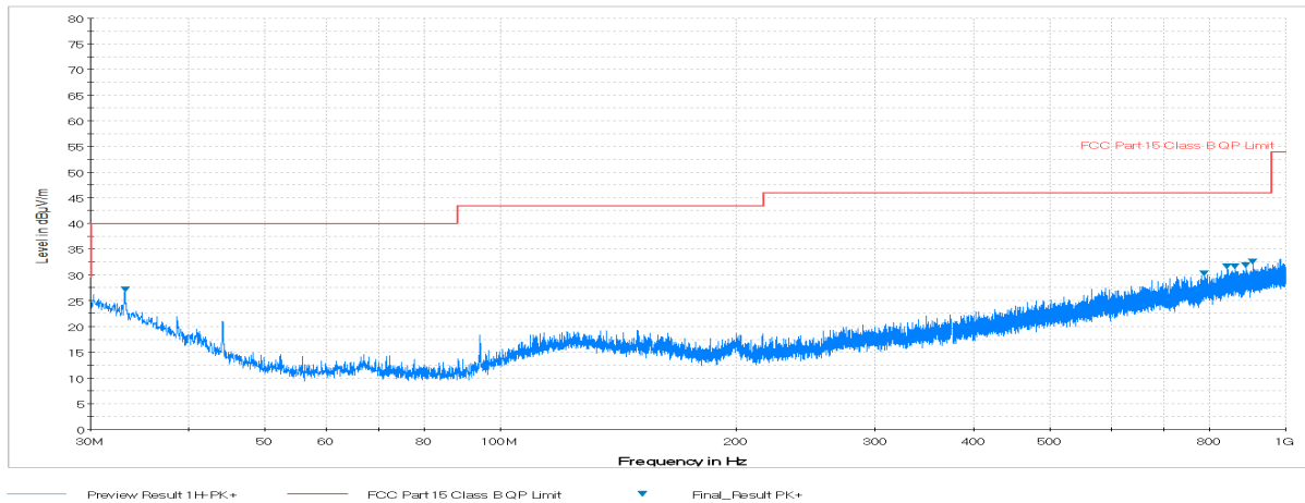
Plot 7-35. Radiated Spurious Plot below 1GHz (Pol. H)
