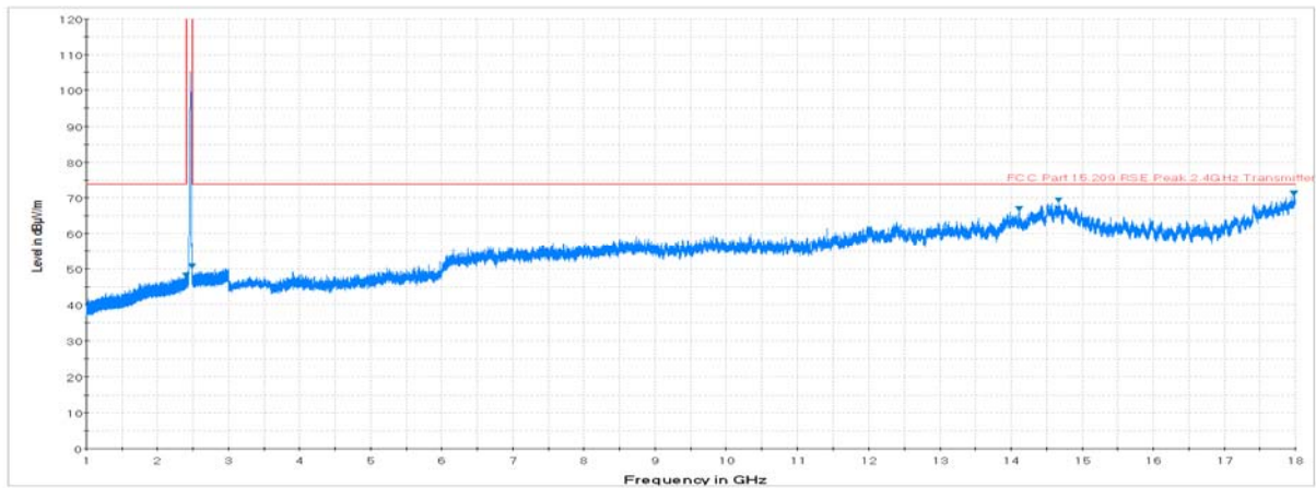
Plot 7-13. Radiated Spurious Plot above 1GHz (802.11b – Ch. 11, Ant. Pol. H)
