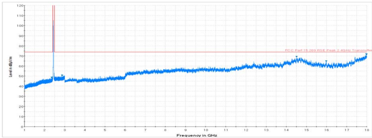
Plot 7-11. Radiated Spurious Plot above 1GHz (802.11b – Ch. 6, Ant. Pol. H)
