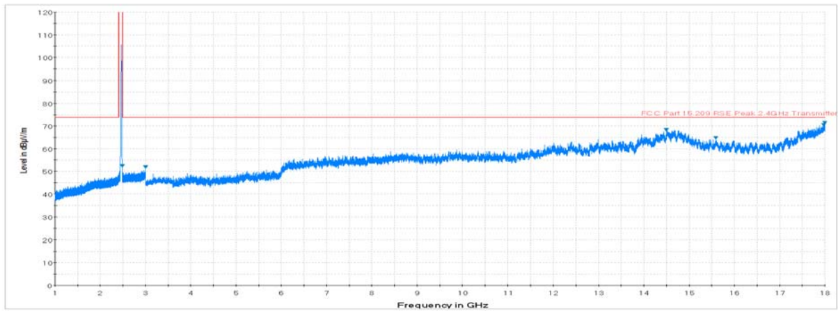
Plot 7-14. Radiated Spurious Plot above 1GHz (802.11b – Ch. 11, Ant. Pol. V)
