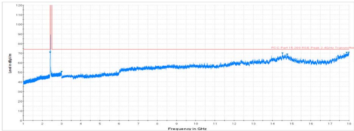
Plot 7-10. Radiated Spurious Plot above 1GHz (802.11b – Ch. 1, Ant. Pol. V)
