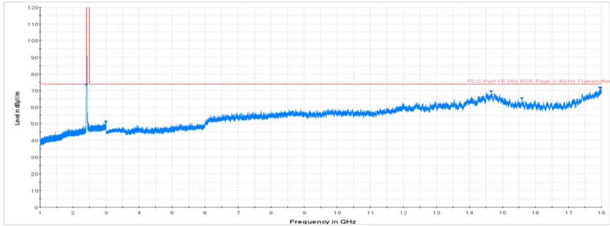
Plot 7-9. Radiated Spurious Plot above 1GHz (802.11b – Ch. 1, Ant. Pol. H)
