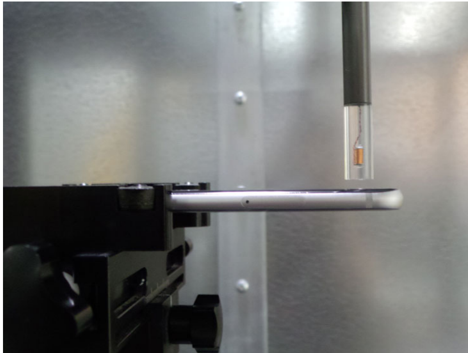
Figure 13-2 Test Setup for Wireless Device
