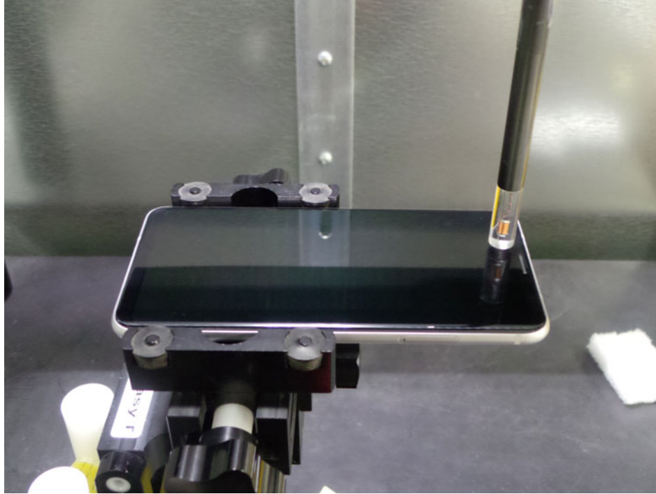
Figure 13-1 Test Setup for Wireless Device
