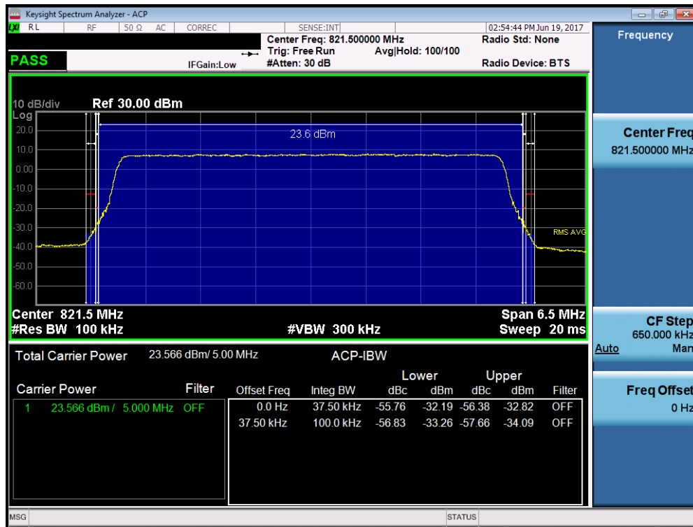
Plot 7-28. Channel Edge Plot (5MHz QPSK – RB Size 25– Low Channel)
