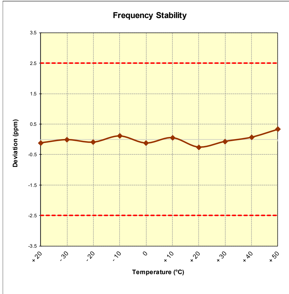
Figure 7-6. CDMA BC10 Frequency Stability Graph (Ch. 476)
