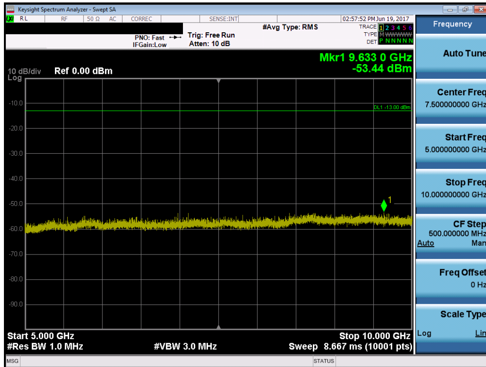
Plot 7-20. Conducted Spurious Plot ( 831.5MHz QPSK – RB Size 1, RB Offset 0 – Low Channel)
