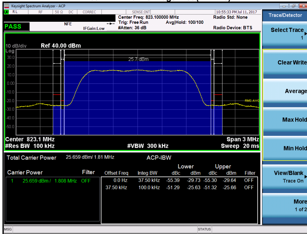
Plot 7-22. Channel Edge Plot (Ch. 684)
