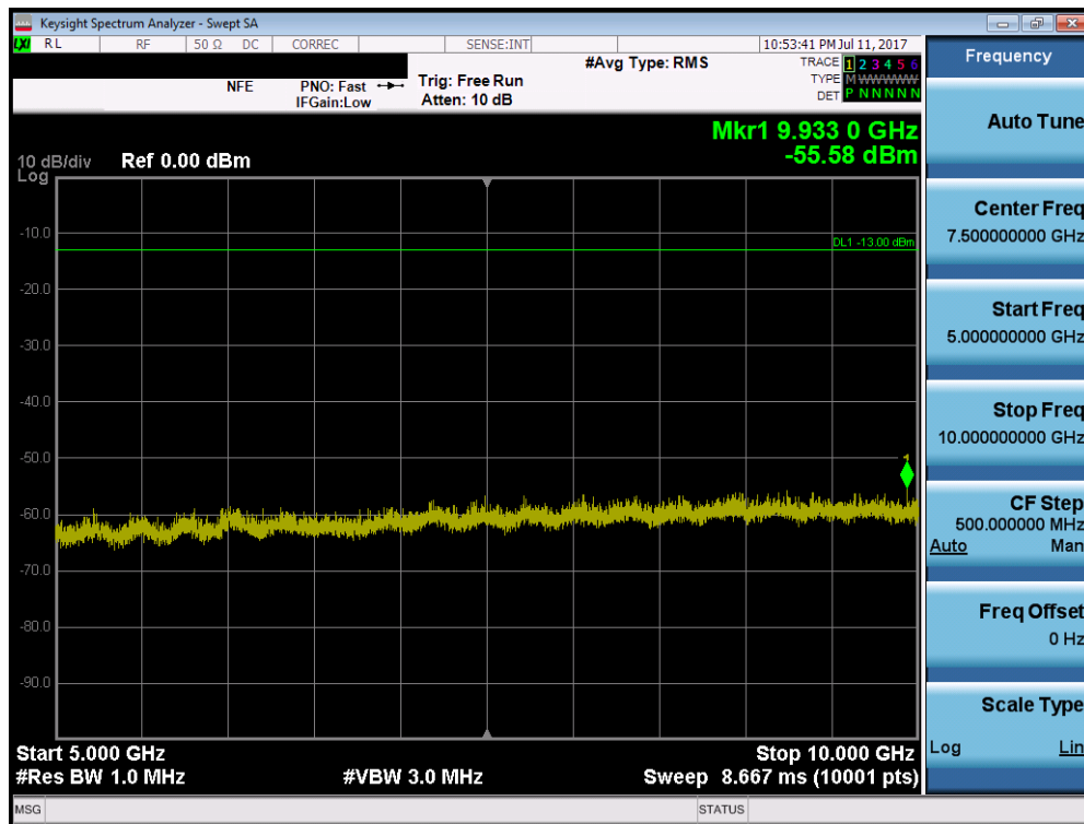
Plot 7-16. Conducted Spurious Plot (Ch. 476)
