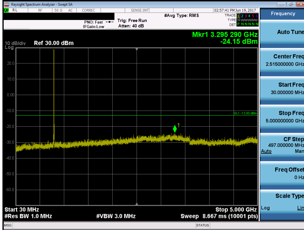
Plot 7-19. Conducted Spurious Plot ( 831.5 MHz QPSK – RB Size 1, RB Offset 0 – Low Channel)
