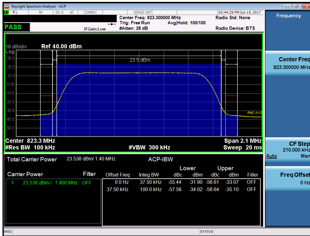
Plot 7-24. Channel Edge Plot (1.4MHz QPSK – RB Size 6 – High Channel)
