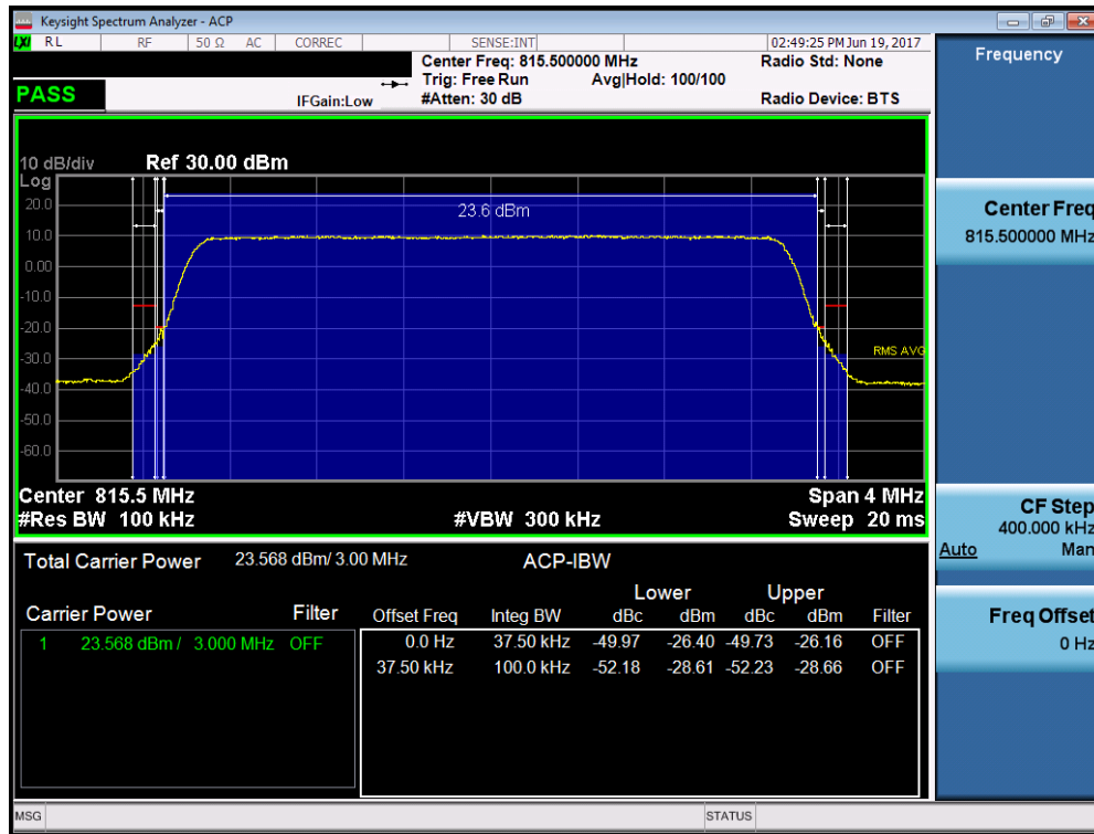
Plot 7-25. Channel Edge Plot (3MHz QPSK – RB Size 15– Low Channel)
