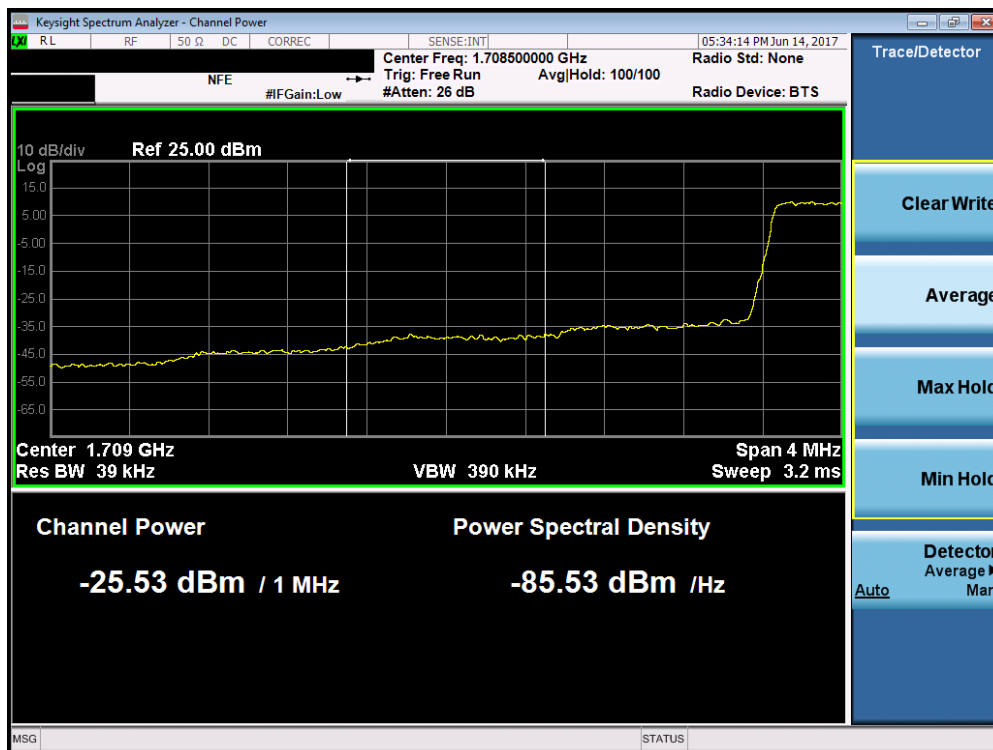
Plot 7-159. Lower Extended Band Edge Plot (Band 4 – 1.4MHz QPSK – RB Size 6)
