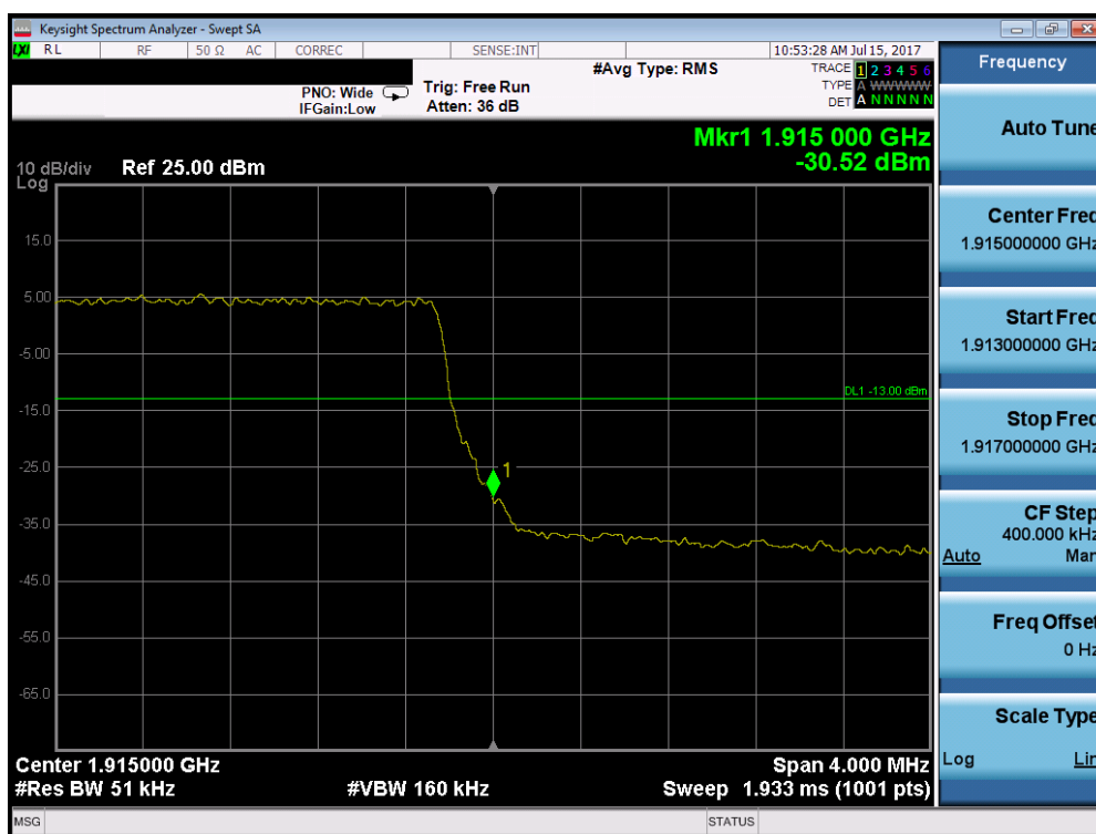
Plot 7-198. Upper Band Edge Plot (Band 25 – 5.0MHz QPSK – RB Size 25)
