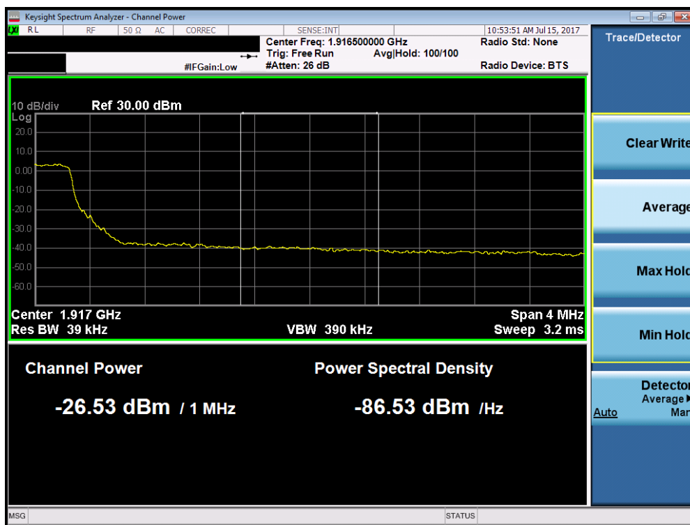
Plot 7-199. Upper Extended Band Edge Plot (Band 25 – 5.0MHz QPSK – RB Size 25)
