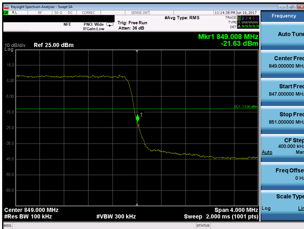
Plot 7-151. Upper Band Edge Plot (Band 5/26 - 3.0MHz QPSK - RB Size 15)
