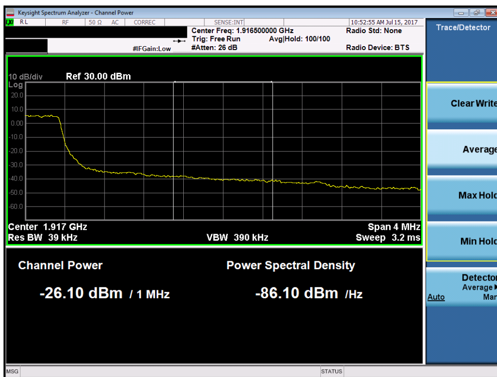
Plot 7-193. Upper Extended Band Edge Plot (Band 25 – 3.0MHz QPSK – RB Size 15)
