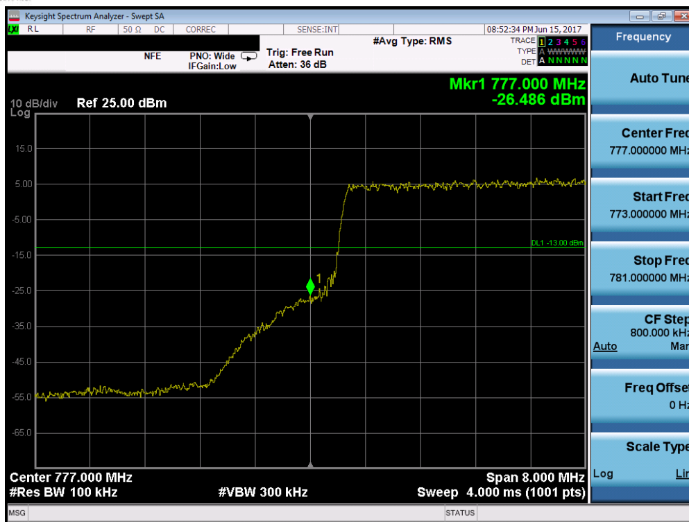
Plot 7-144. Lower Band Edge Plot (Band 13 – 10.0MHz QPSK – RB Size 50)
