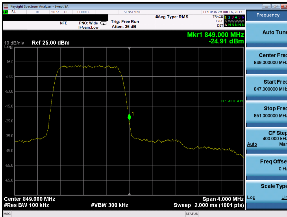
Plot 7-149. Upper Band Edge Plot (Band 5/26 – 1.4MHz QPSK – RB Size 6)
