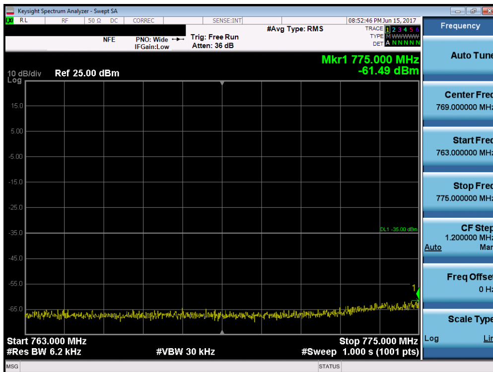
Plot 7-145. Lower Emission Mask Edge Plot (Band 13 – 10.0MHz QPSK – RB Size 50)
