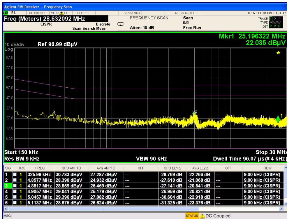
Plot 7-238. Line Conducted Plot with 802.11a UNII Band 2C (N)
