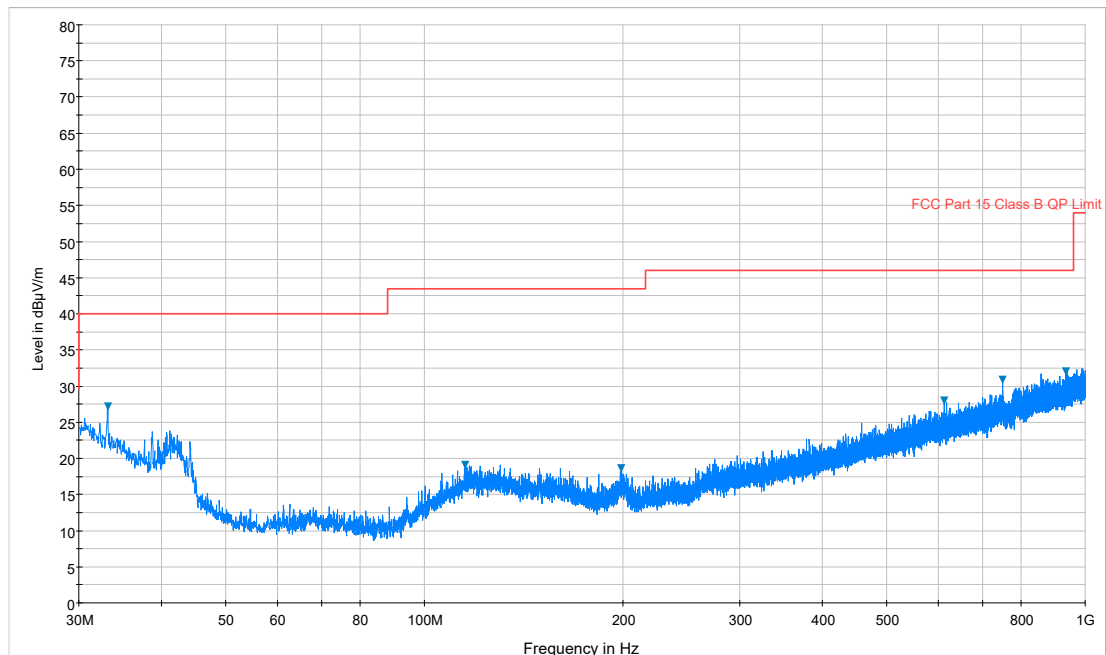
Plot 7-232. Radiated Spurious Plot below 1GHz (802.11a – U3 Ch. 157, Ant. Pol. V)
