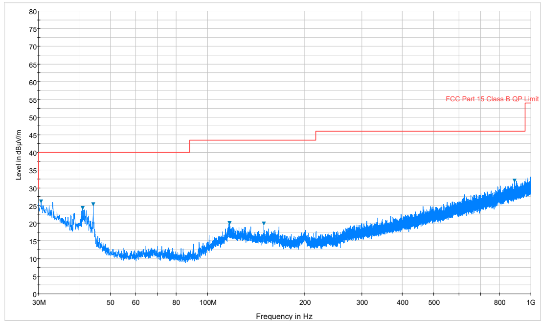
Plot 7-231. Radiated Spurious Plot below 1GHz (802.11a – U3 Ch. 157, Ant. Pol. H)
