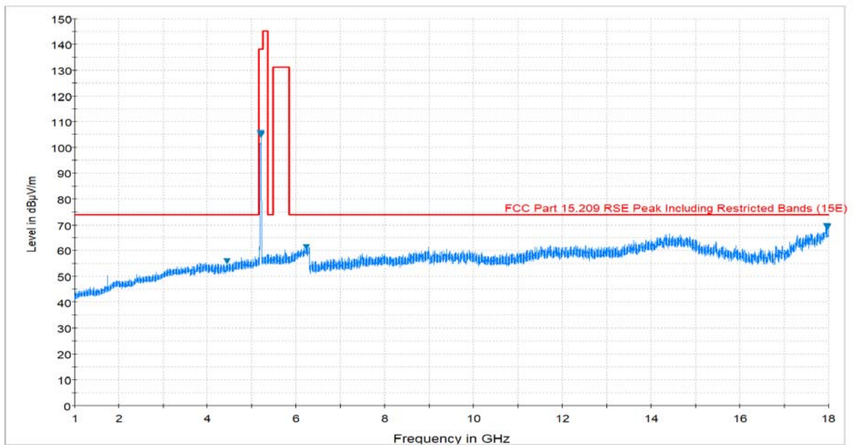
Plot 7-166. Radiated Spurious Plot above 1GHz (802.11a – U1 Ch. 40, Ant. Pol. V)
