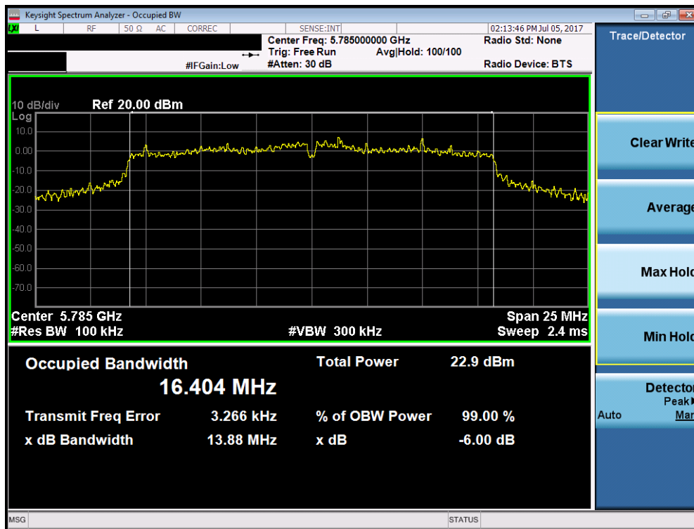
Plot 7-69. 6dB Bandwidth Plot (802.11a (UNII Band 3) – Ch. 157)
