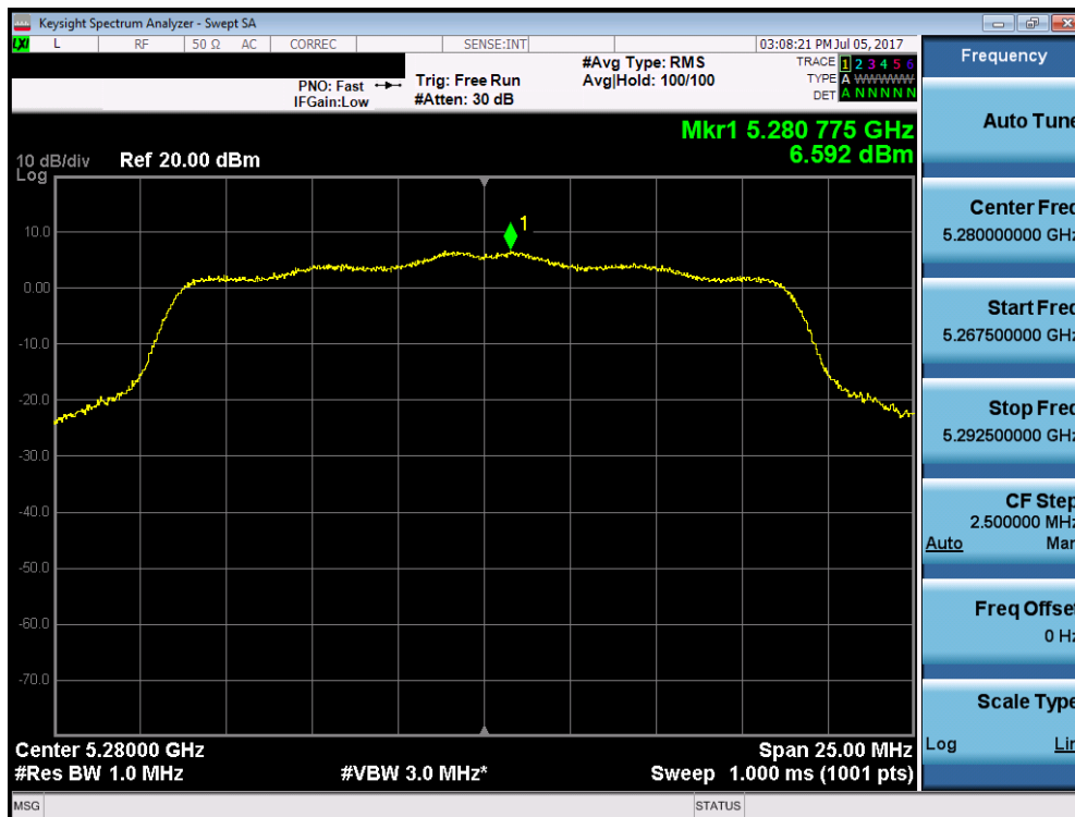
Plot 7-90. Power Spectral Density Plot (20MHz BW 802.11n (UNII Band 2A) – Ch. 56)
