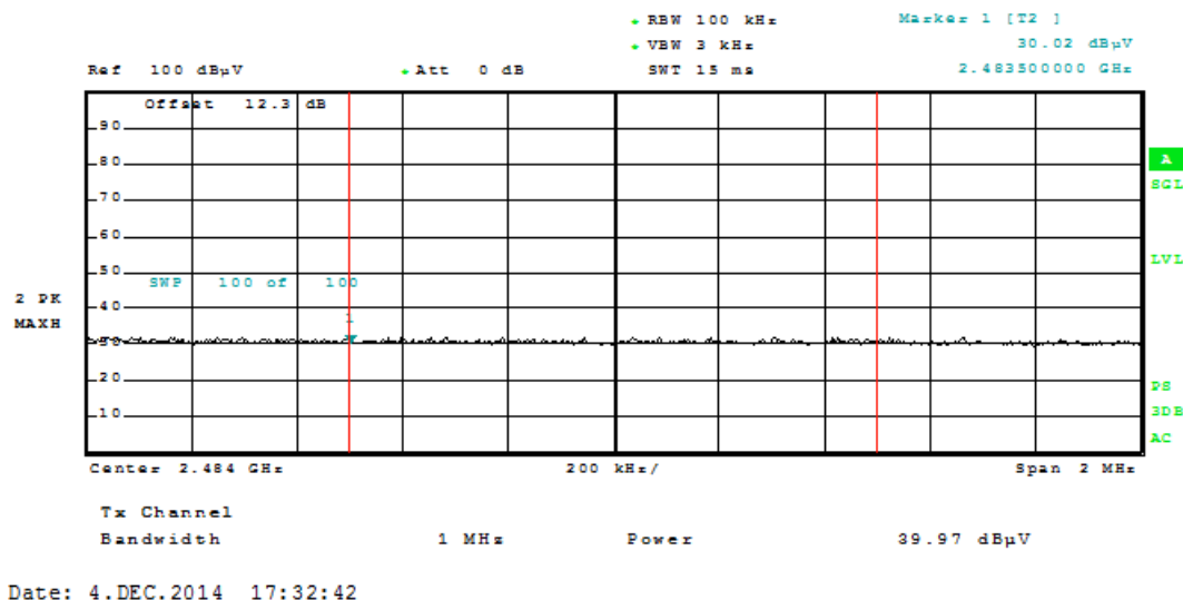
Plot 6-1. Radiated Restricted Upper Band Edge Measurement (Average)
