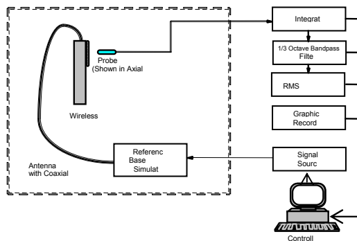
Figure 5-14 Audio Magnetic Field Test Setup
