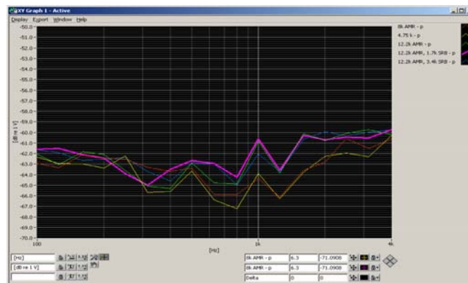
Figure 6-2 UMTS Audio Band Magnetic Noise
