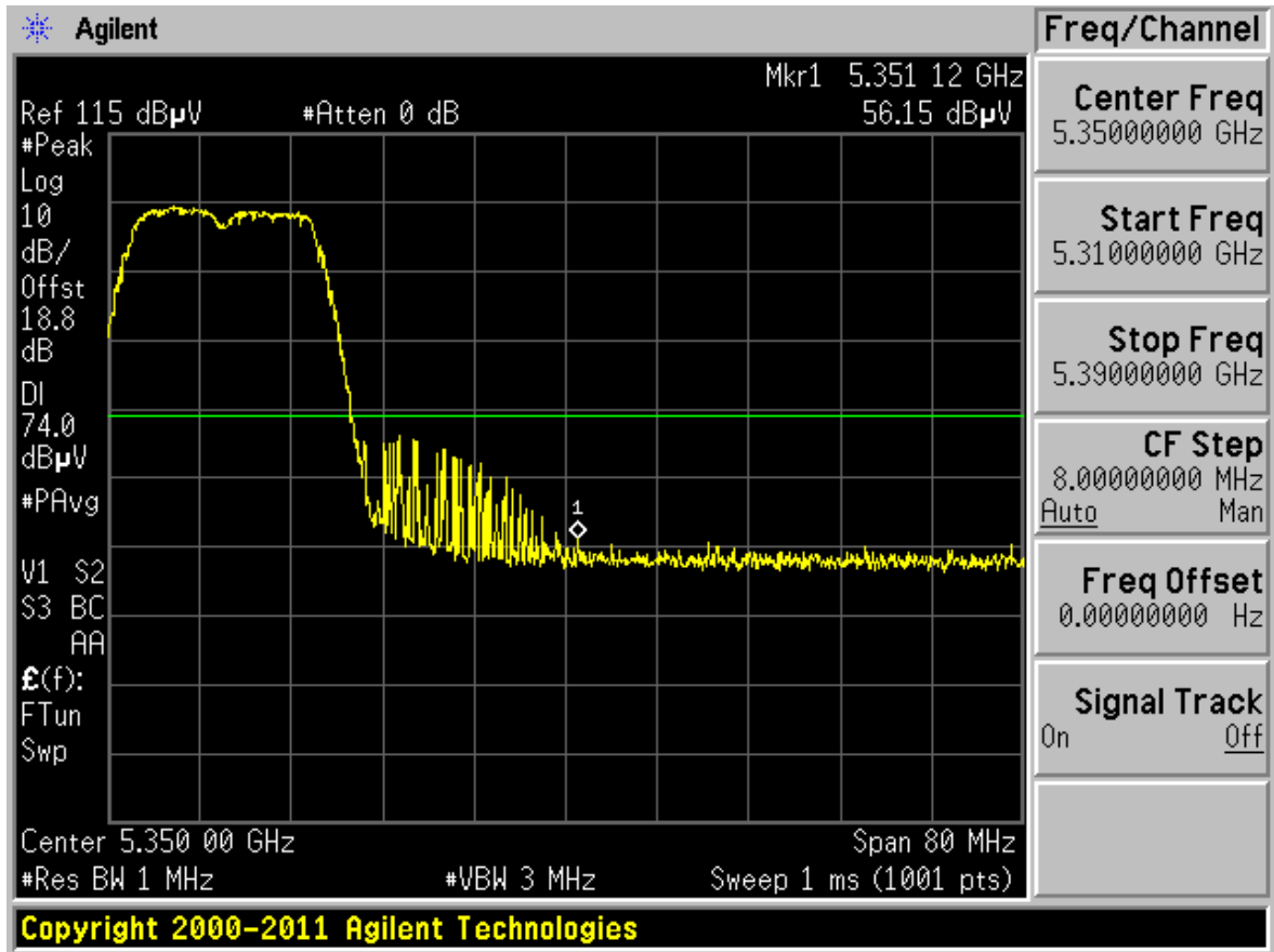
Plot 6-86. Radiated Restricted Upper Band Edge Plot (Peak – UNII Band 2)
