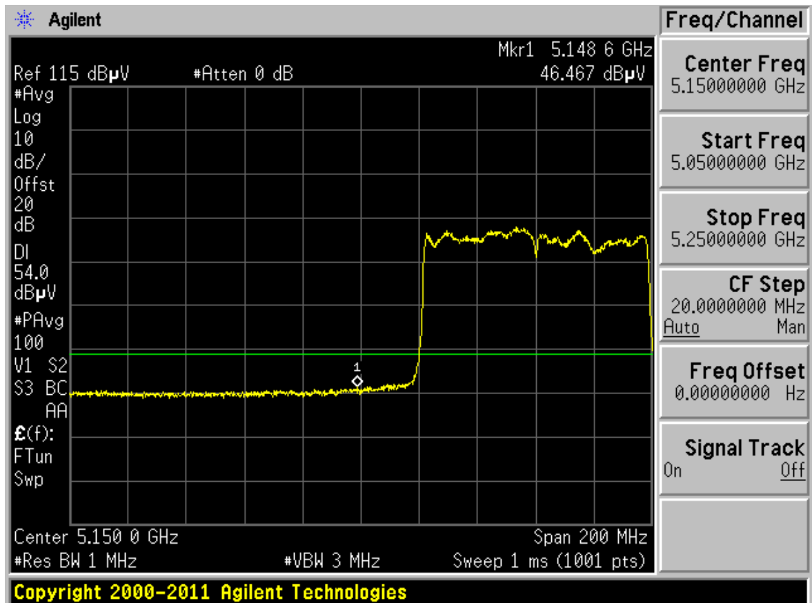
Plot 6-97. Radiated Restricted Lower Band Edge Plot (Average – UNII Band 1)
