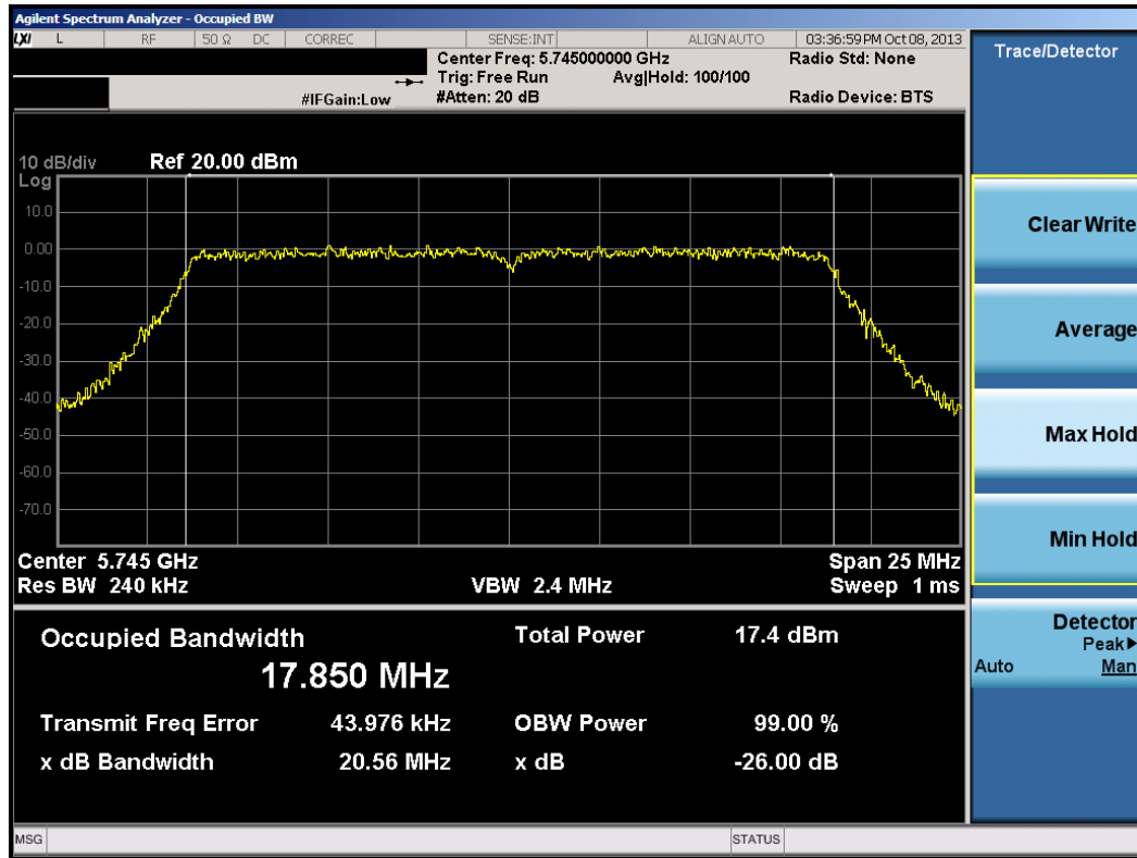
Plot 6-33. 26dB Bandwidth Plot (20MHz BW 802.11n (UNII Band 4) – Ch. 149)
