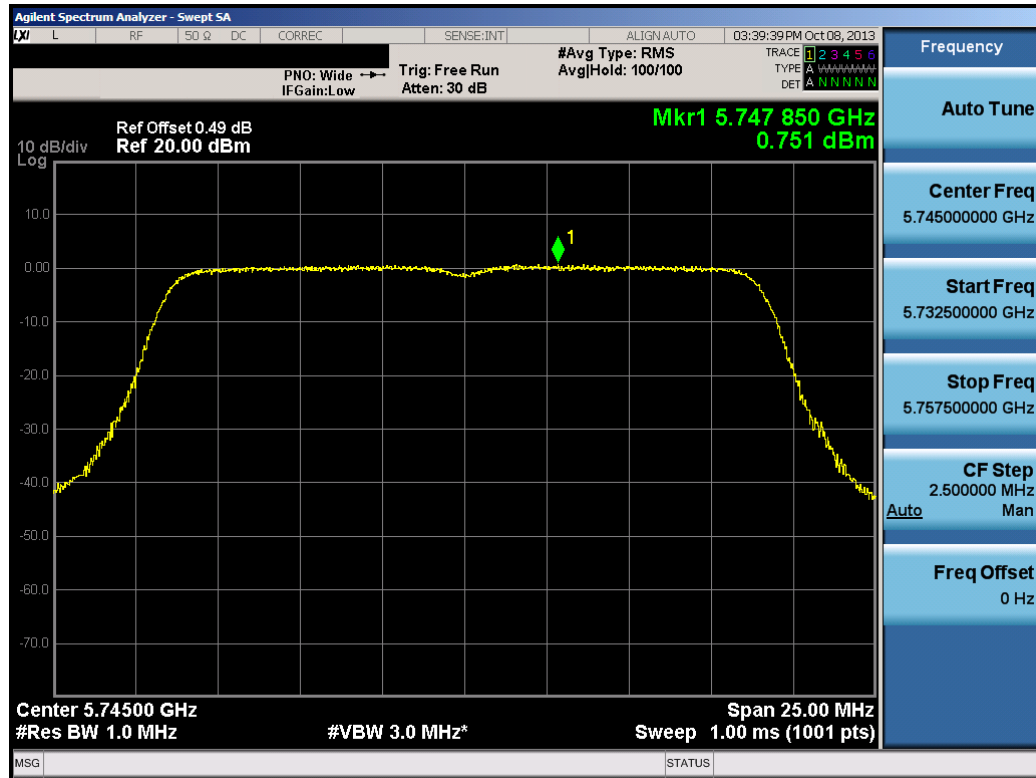
Plot 6-73. Peak Power Spectral Density Plot (20MHz BW 802.11n (UNII Band 4) – Ch. 149)
