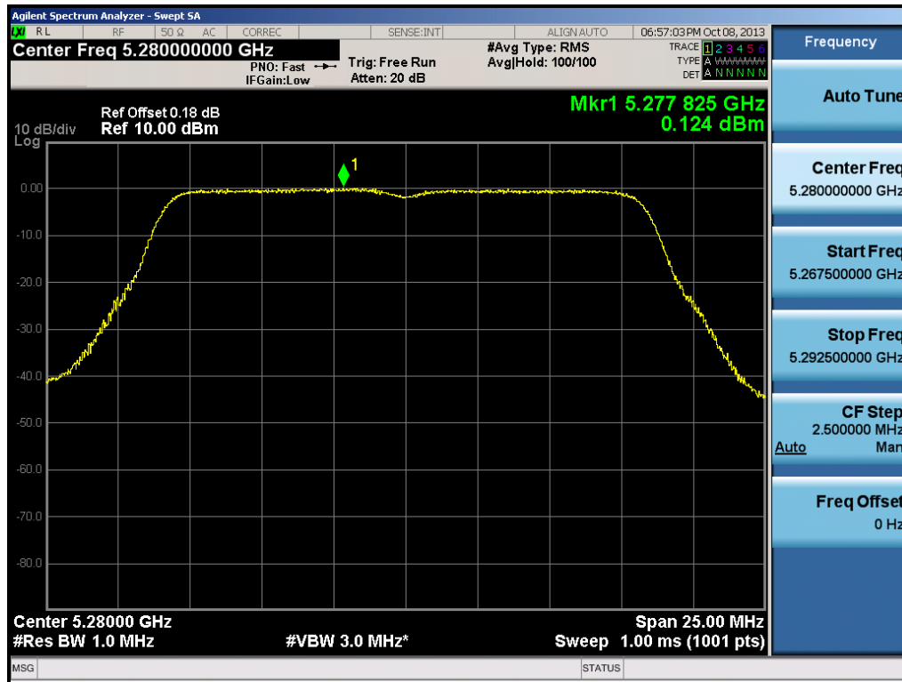
Plot 6-51. Peak Power Spectral Density Plot (802.11a (UNII Band 2) – Ch. 56)
