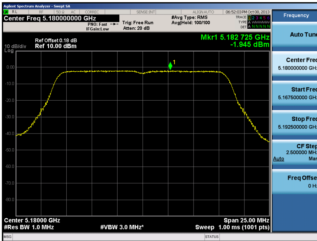
Plot 6-41. Peak Power Spectral Density Plot (802.11a (UNII Band 1) – Ch. 36)
