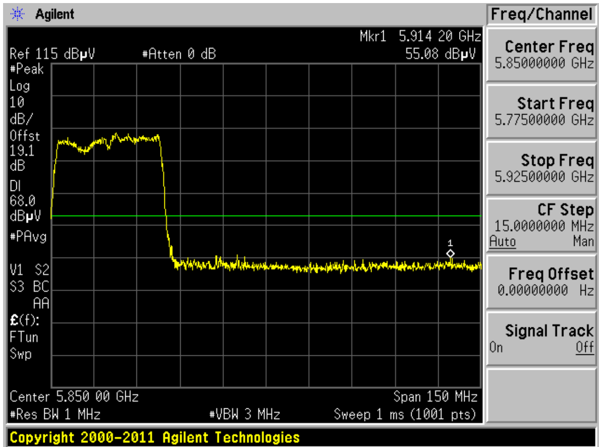
Plot 6-89. Radiated Upper Band Edge Plot (Peak – UNII Band 3)
