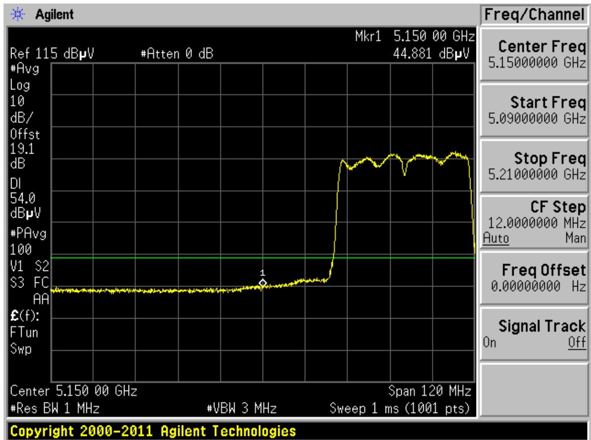
Plot 6-90. Radiated Restricted Lower Band Edge Plot (Average – UNII Band 1)
