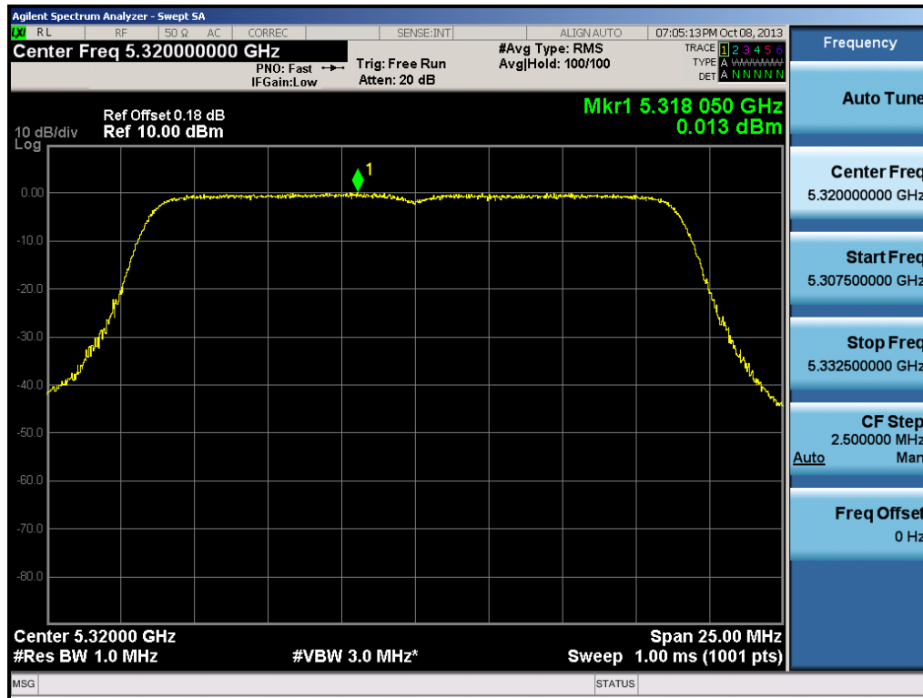
Plot 6-55. Peak Power Spectral Density Plot (20MHz BW 802.11n (UNII Band 2) – Ch. 64)
