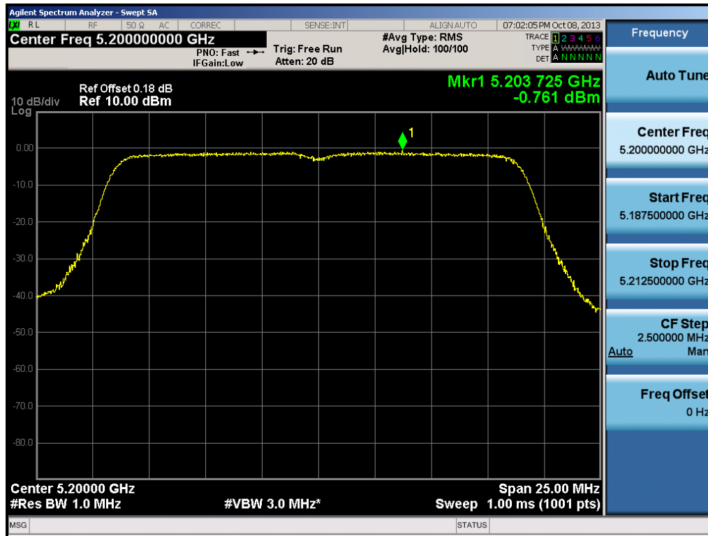
Plot 6-45. Peak Power Spectral Density Plot (20MHz BW 802.11n (UNII Band 1) – Ch. 40)
