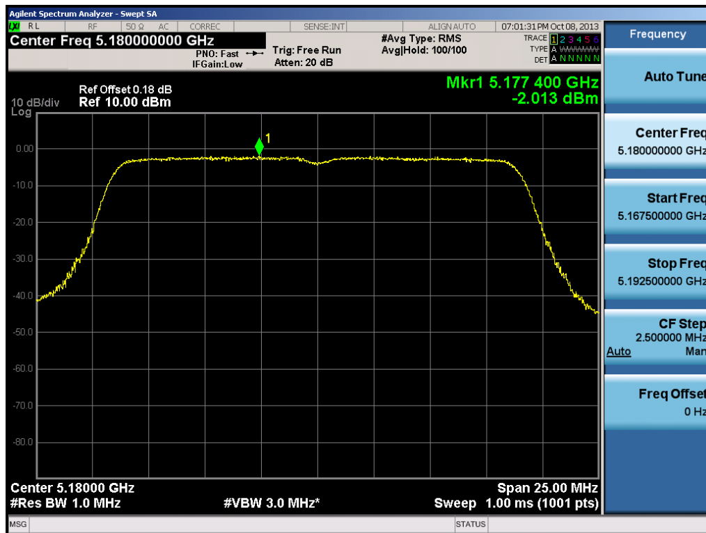
Plot 6-44. Peak Power Spectral Density Plot (20MHz BW 802.11n (UNII Band 1) – Ch. 36)
