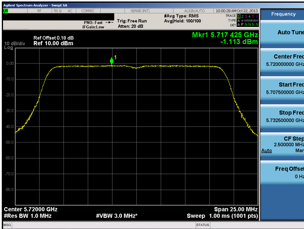
Plot 6-64. Peak Power Spectral Density Plot (20MHz BW 802.11n (UNII Band 3) – Ch. 144)
