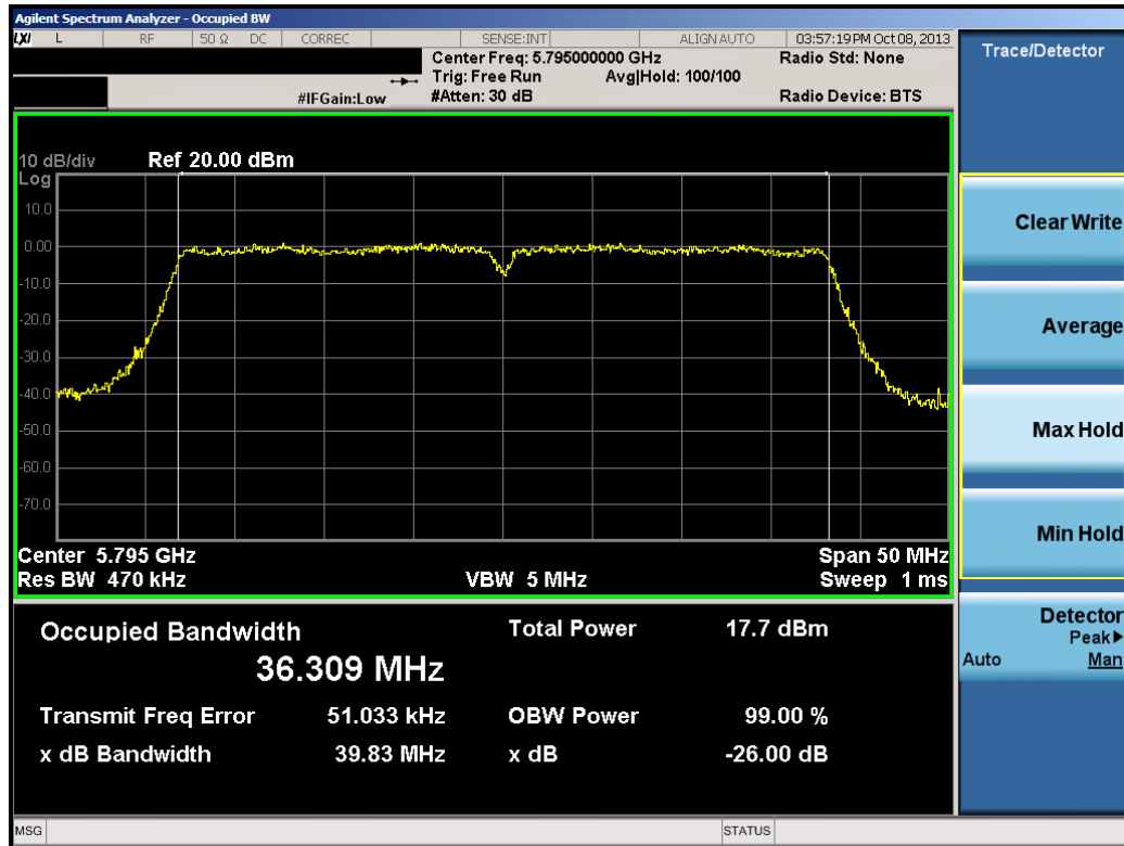
Plot 6-37. 26dB Bandwidth Plot (40MHz BW 802.11n (UNII Band 4) – Ch. 159)
