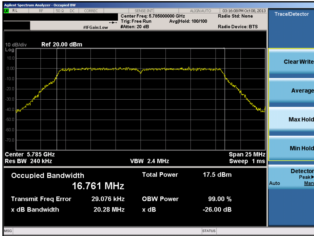
Plot 6-31. 26dB Bandwidth Plot (20MHz BW 802.11a (UNII Band 4) – Ch. 157)
