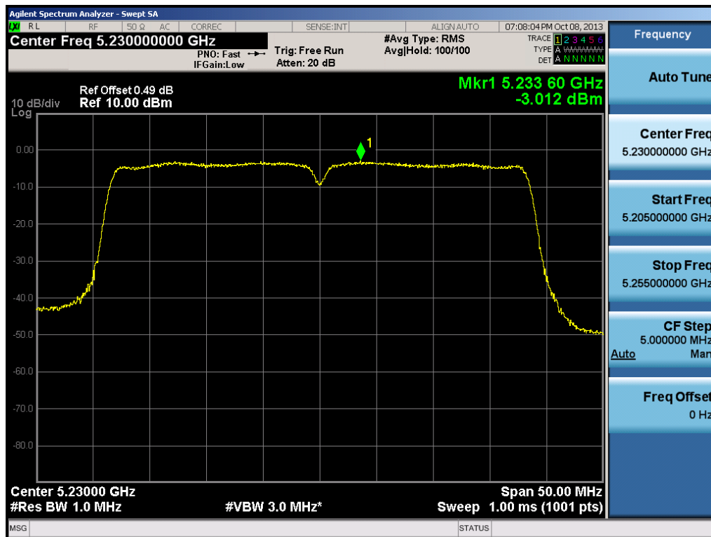
Plot 6-48. Peak Power Spectral Density Plot (40MHz BW 802.11n (UNII Band 1) – Ch. 46)
