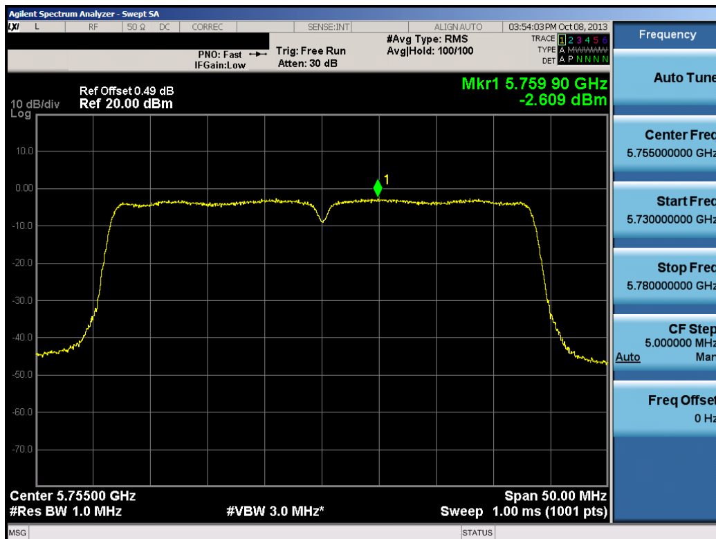
Plot 6-76. Peak Power Spectral Density Plot (40MHz BW 802.11n (UNII Band 4) – Ch. 151)
