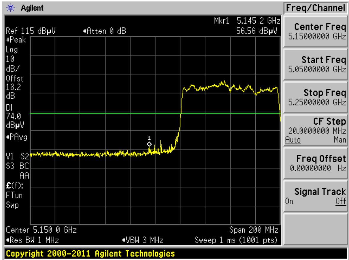
Plot 6-98. Radiated Restricted Lower Band Edge Plot (Peak – UNII Band 1)
