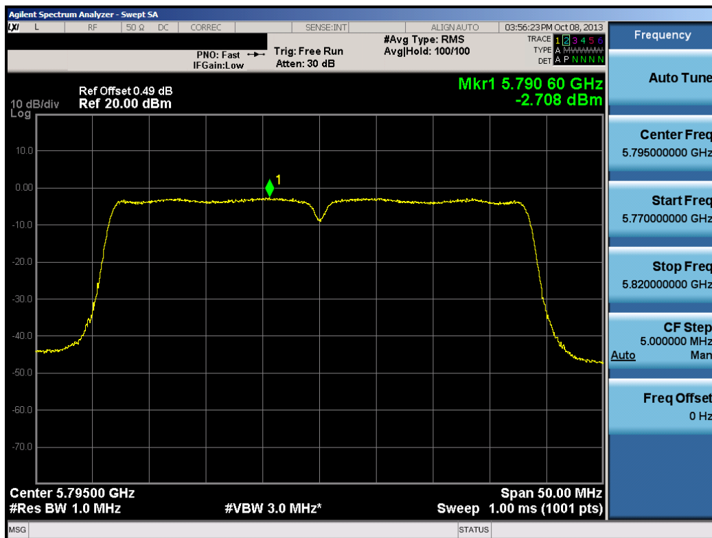
Plot 6-77. Peak Power Spectral Density Plot (40MHz BW 802.11n (UNII Band 4) – Ch. 159)
