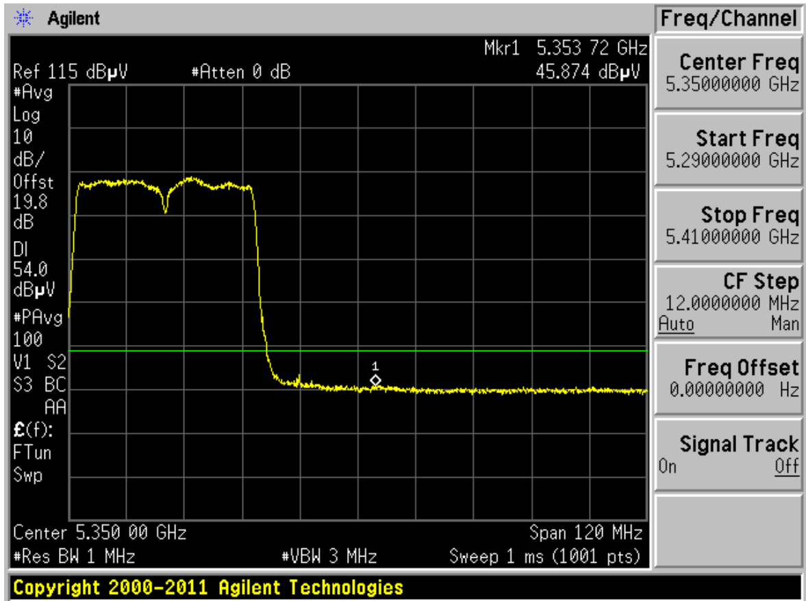
Plot 6-92. Radiated Restricted Upper Band Edge Plot (Average – UNII Band 2)
