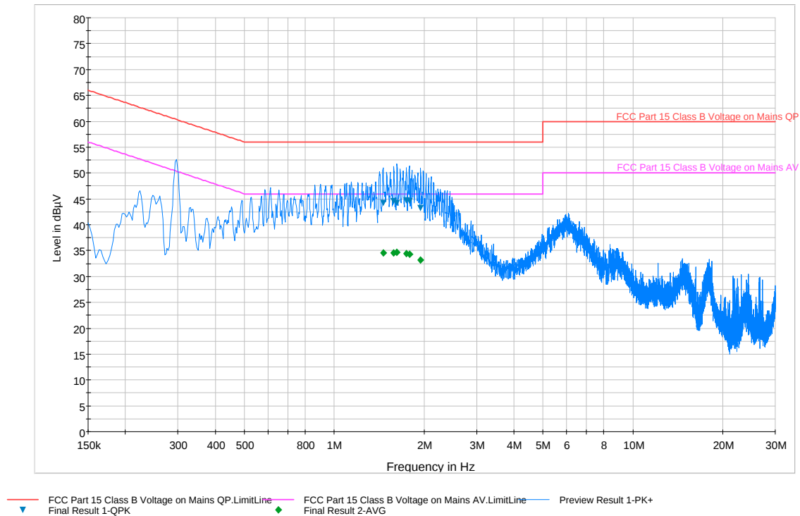
Plot 6-110. Line Conducted Plot with 802.11a UNII Band 4 (N)
