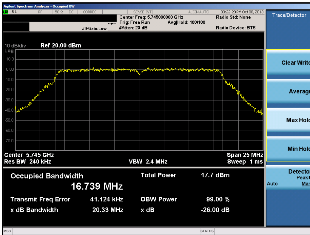
Plot 6-30. 26dB Bandwidth Plot (20MHz BW 802.11a (UNII Band 4) – Ch. 149)
