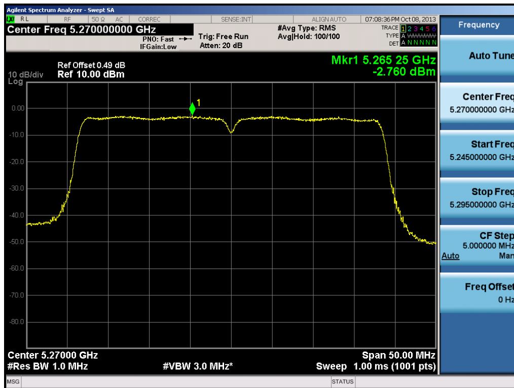
Plot 6-56. Peak Power Spectral Density Plot (40MHz BW 802.11n (UNII Band 2) – Ch. 54)
