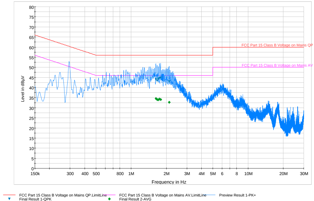
Plot 6-106. Line Conducted Plot with 802.11a UNII Band 2 (N)
