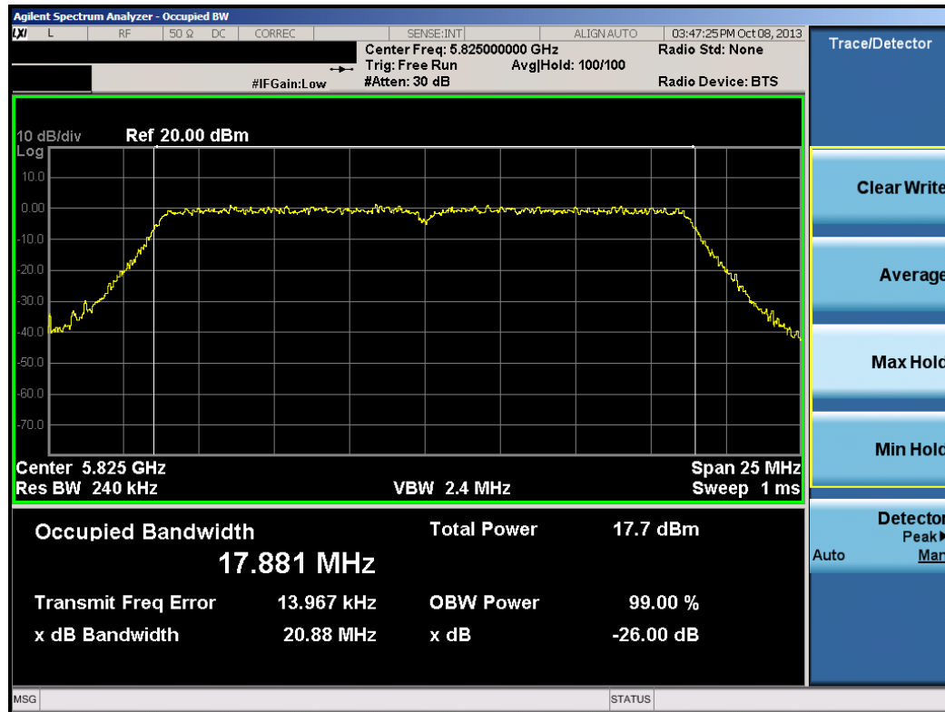
Plot 6-35. 26dB Bandwidth Plot (20MHz BW 802.11n (UNII Band 4) – Ch. 165)
