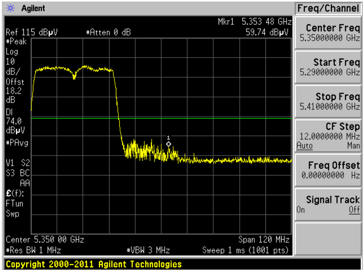
Plot 6-93. Radiated Restricted Upper Band Edge Plot (Peak – UNII Band 2)
