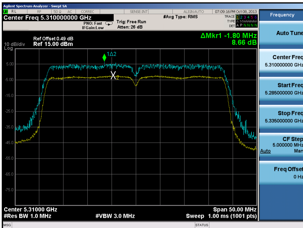
Plot 6-81. Peak Excursion Ratio Plot (40MHz BW 802.11n)
