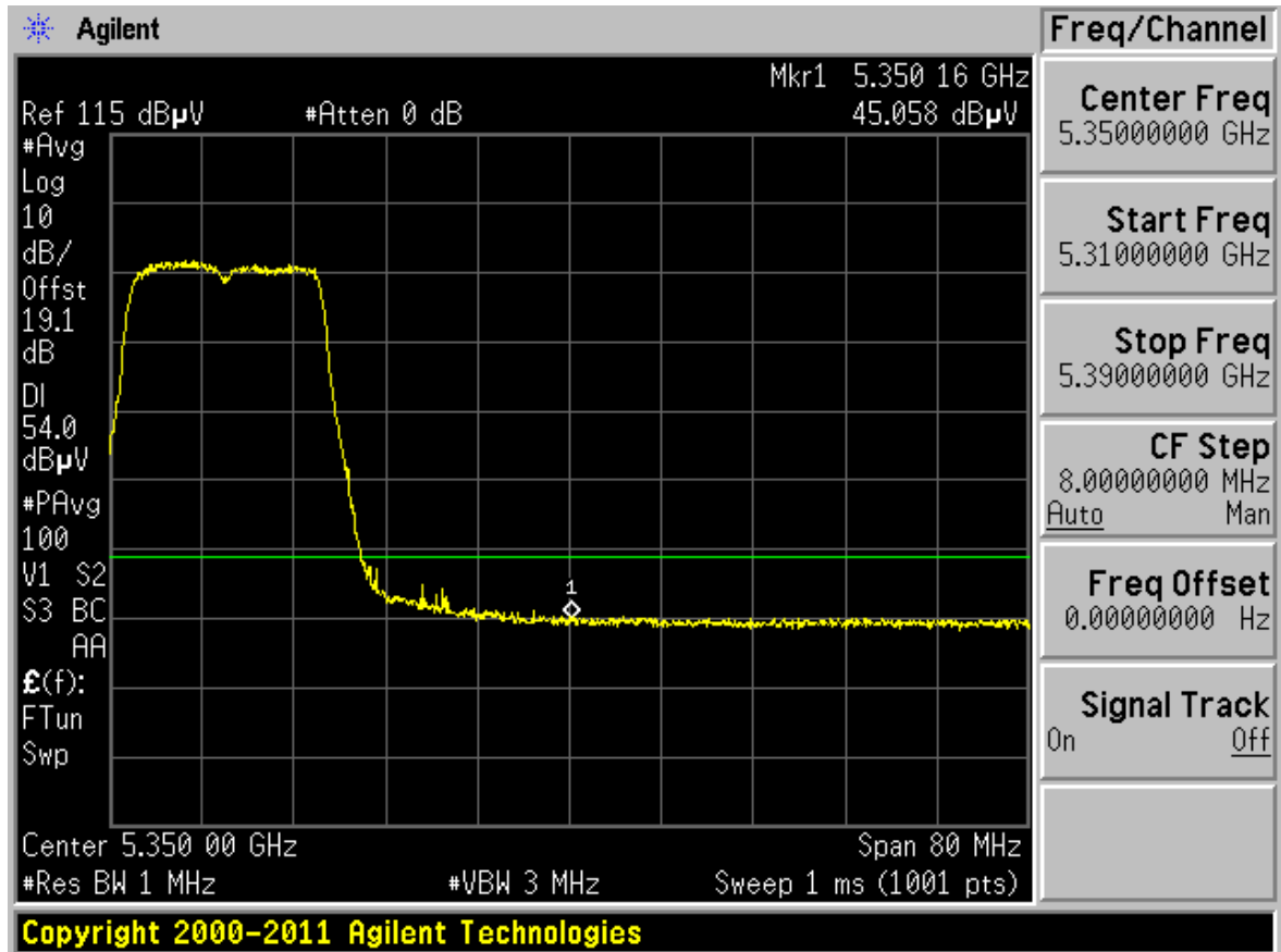
Plot 6-85. Radiated Restricted Upper Band Edge Plot (Average – UNII Band 2)
