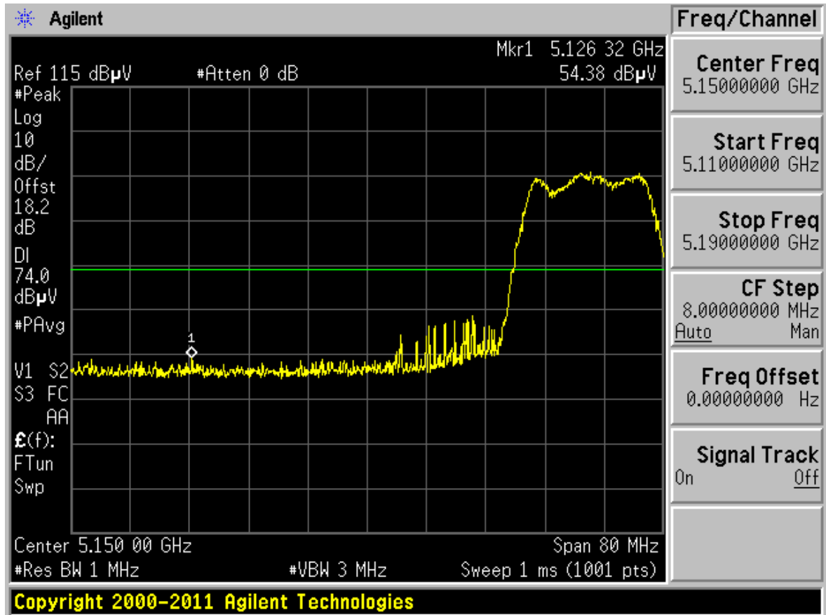
Plot 6-84. Radiated Restricted Lower Band Edge Plot (Peak – UNII Band 1)
