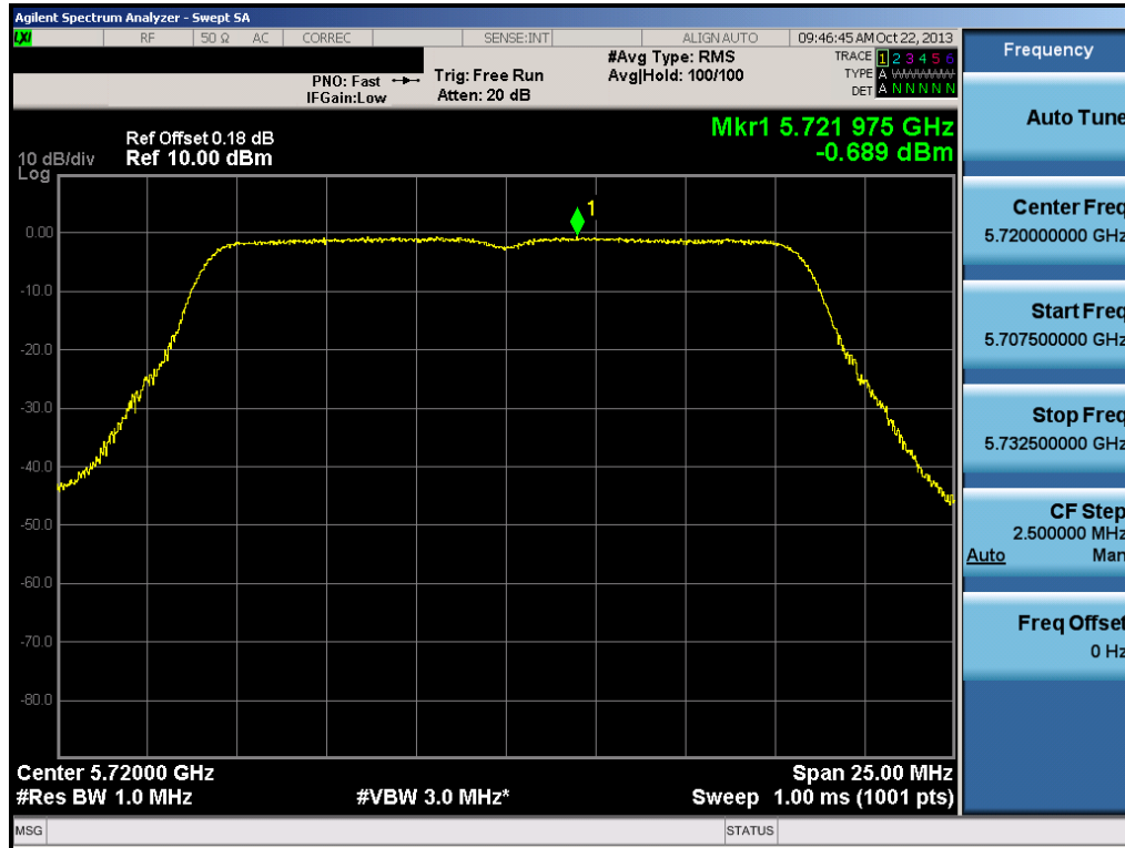
Plot 6-61. Peak Power Spectral Density Plot (802.11a (UNII Band 3) – Ch. 144)
