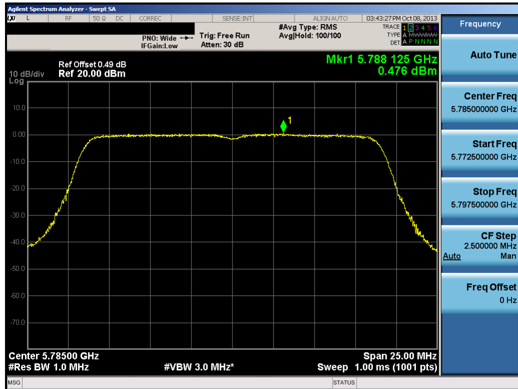
Plot 6-74. Peak Power Spectral Density Plot (20MHz BW 802.11n (UNII Band 4) – Ch. 157)
