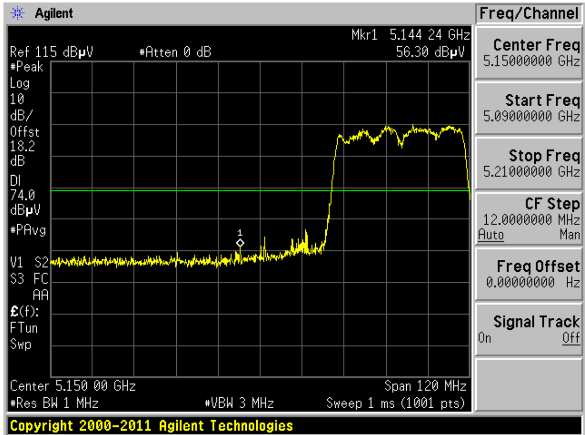
Plot 6-91. Radiated Restricted Lower Band Edge Plot (Peak – UNII Band 1)
