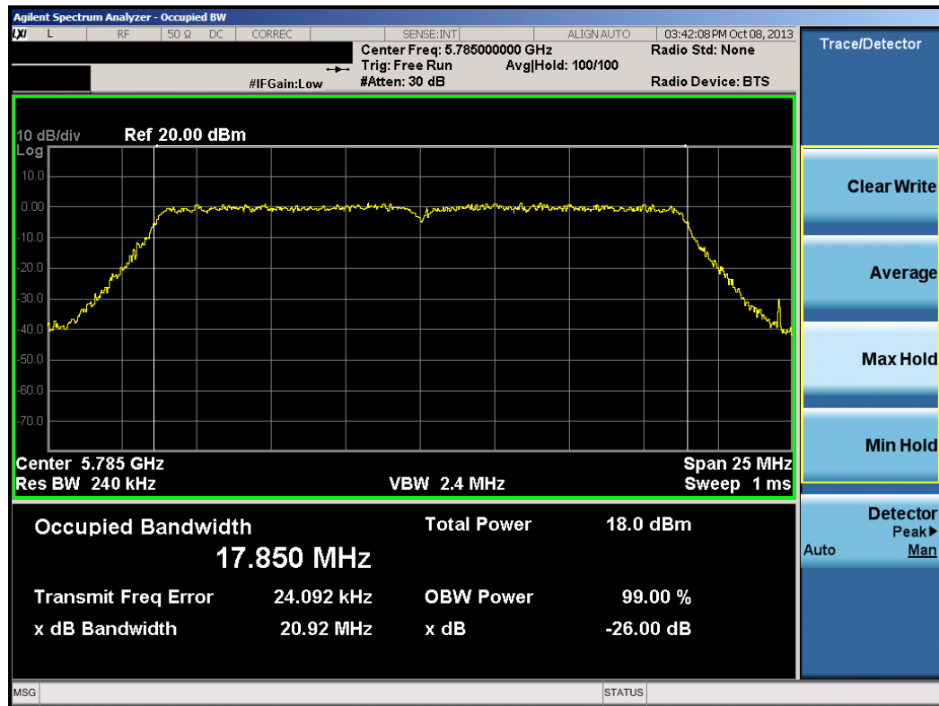
Plot 6-34. 26dB Bandwidth Plot (20MHz BW 802.11n (UNII Band 4) – Ch. 157)
