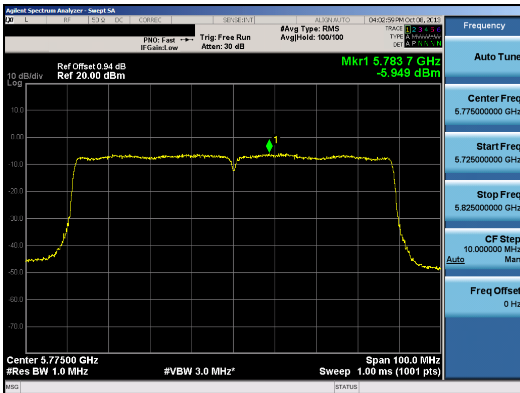
Plot 6-78. Peak Power Spectral Density Plot (80MHz BW 802.11ac (UNII Band 4) – Ch. 155)
