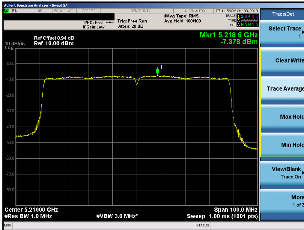
Plot 6-49. Peak Power Spectral Density Plot (80MHz BW 802.11ac (UNII Band 1) – Ch. 42)
