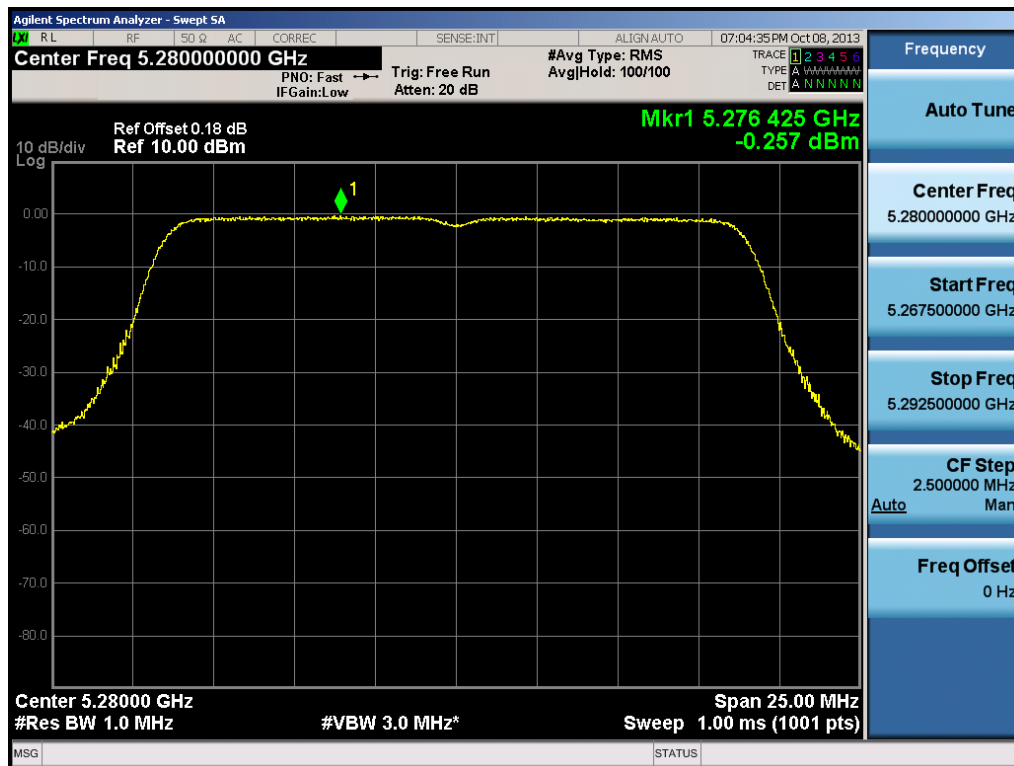
Plot 6-54. Peak Power Spectral Density Plot (20MHz BW 802.11n (UNII Band 2) – Ch. 56)
