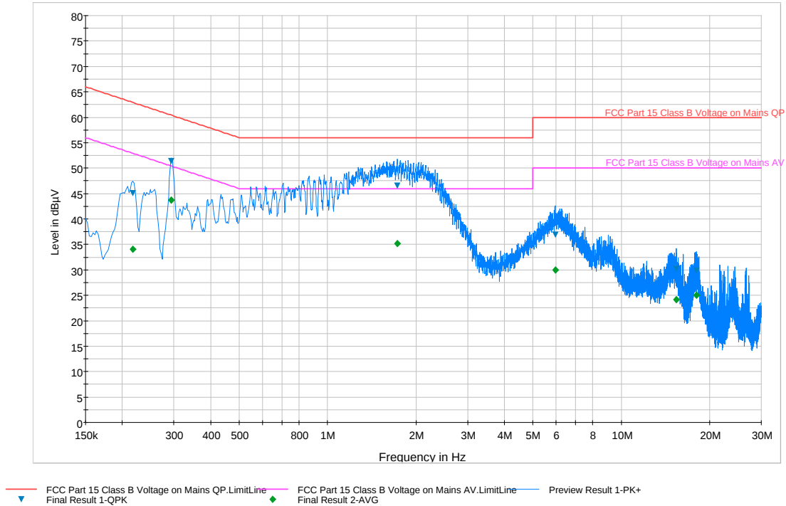
Plot 6-109. Line Conducted Plot with 802.11a UNII Band 4 (L1)
