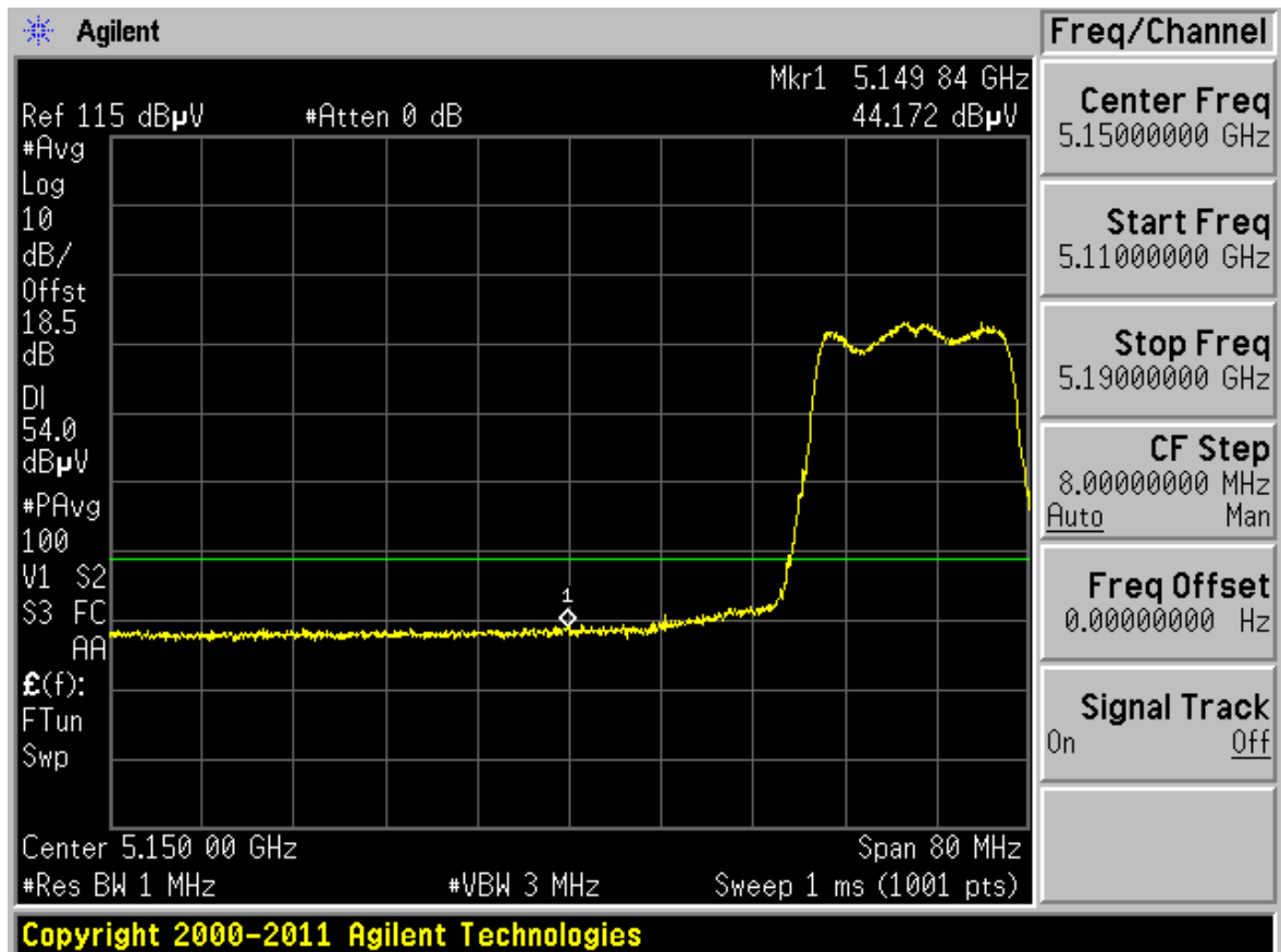
Plot 6-83. Radiated Restricted Lower Band Edge Plot (Average – UNII Band 1)
