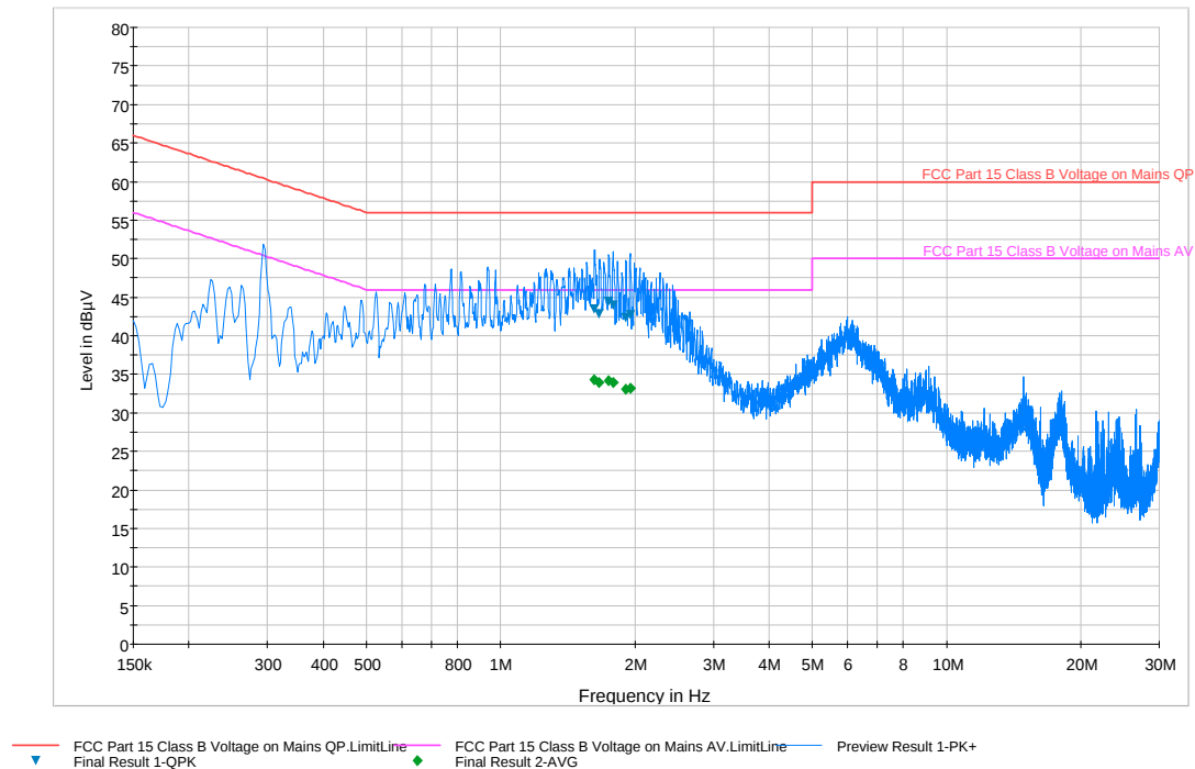
Plot 6-108. Line Conducted Plot with 802.11a UNII Band 3 (N)
