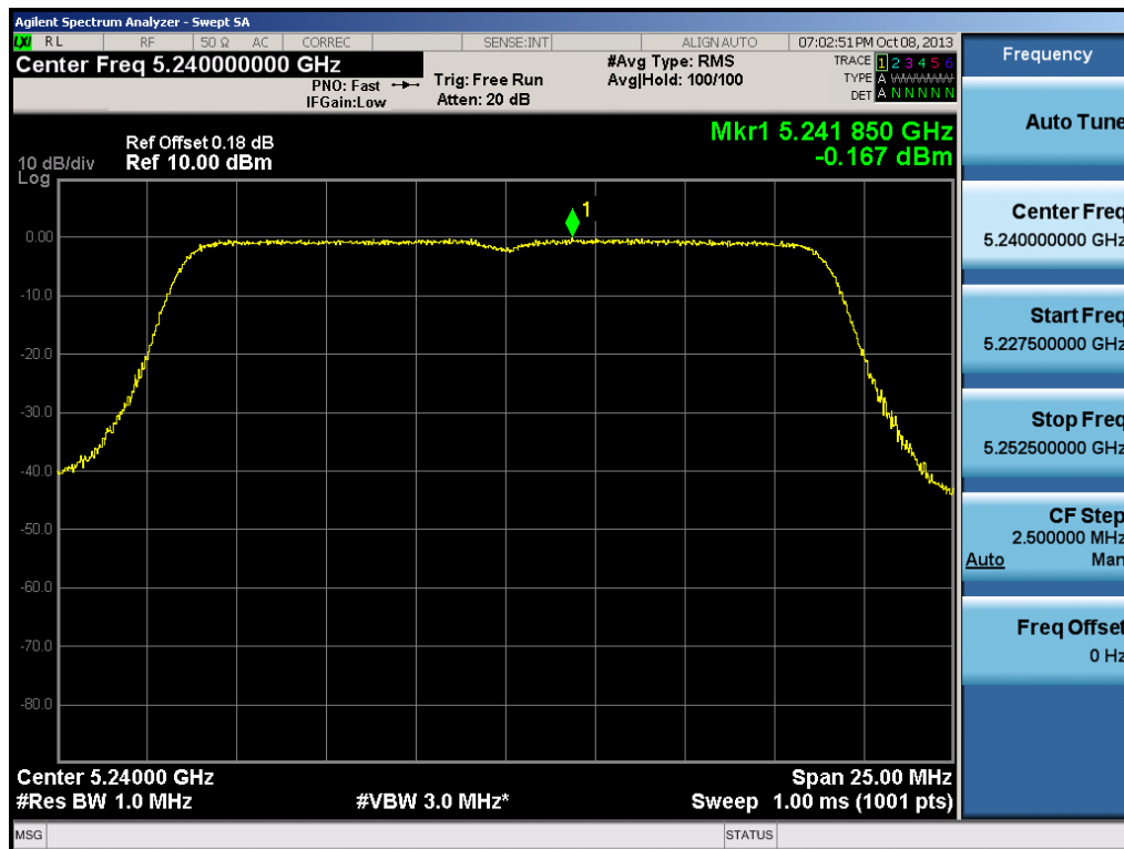
Plot 6-46. Peak Power Spectral Density Plot (20MHz BW 802.11n (UNII Band 1) – Ch. 48)
