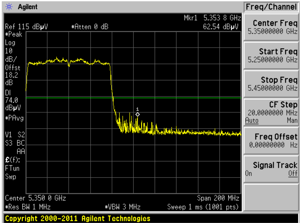
Plot 6-99. Radiated Restricted Upper Band Edge Plot (Average – UNII Band 2)
