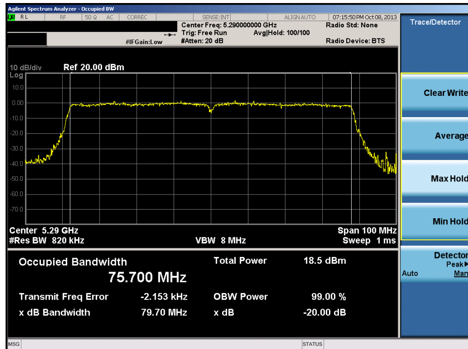
Plot 6-40. 20dB Bandwidth Plot (80MHz BW 802.11n (UNII Band 2) – Ch. 58)
