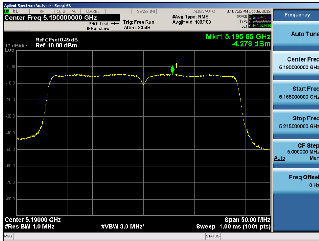
Plot 6-47. Peak Power Spectral Density Plot (40MHz BW 802.11n (UNII Band 1) – Ch. 38)
