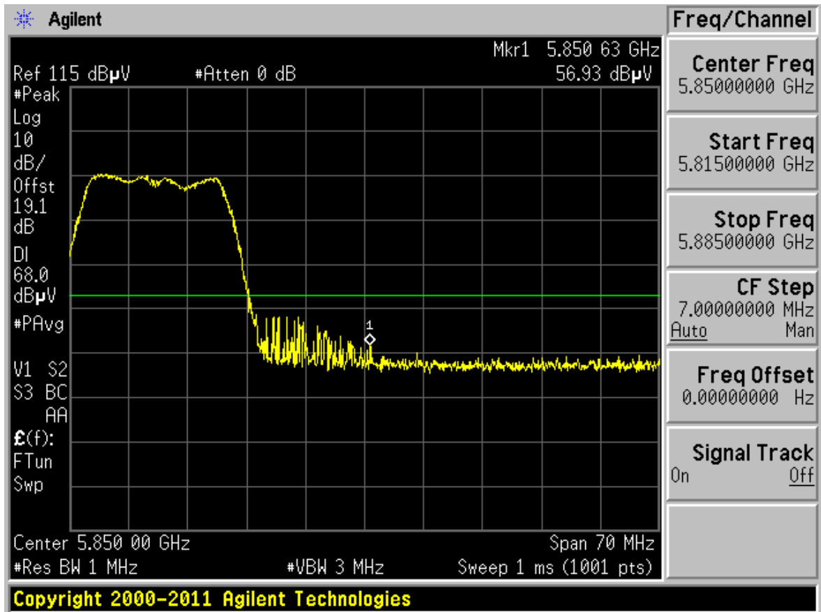
Plot 6-96. Radiated Upper Band Edge Plot (Peak – UNII Band 3)
