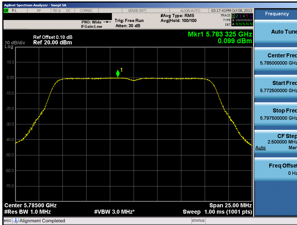
Plot 6-71. Peak Power Spectral Density Plot (20MHz BW 802.11a (UNII Band 4) – Ch. 157)
