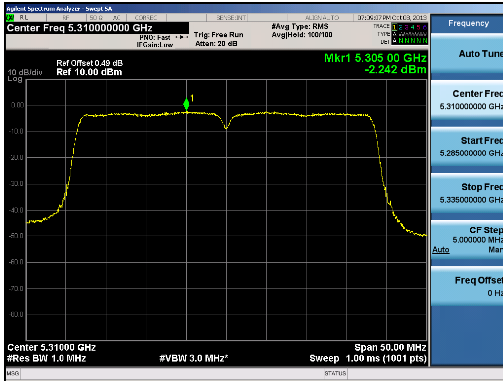
Plot 6-57. Peak Power Spectral Density Plot (40MHz BW 802.11n (UNII Band 2) – Ch. 62)
