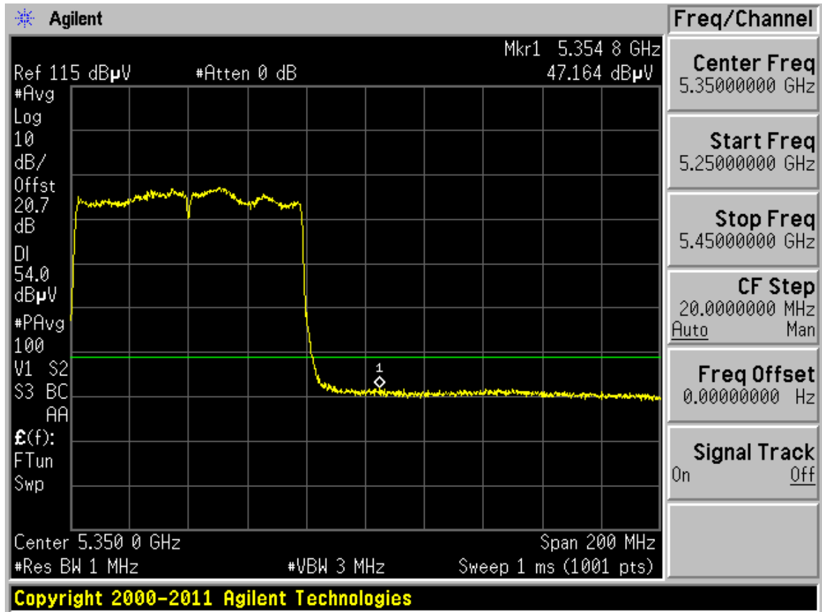
Plot 6-100. Radiated Restricted Upper Band Edge Plot (Peak – UNII Band 2)
