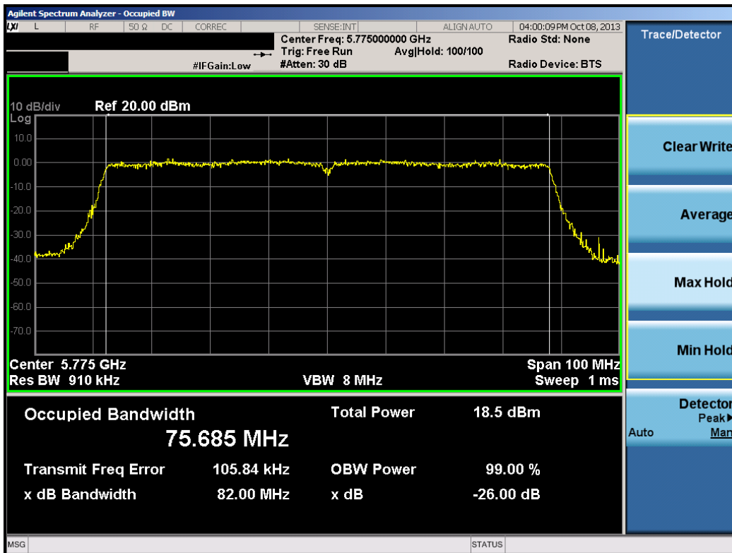
Plot 6-38. 26dB Bandwidth Plot (80MHz BW 802.11ac (UNII Band 4) – Ch. 155)
