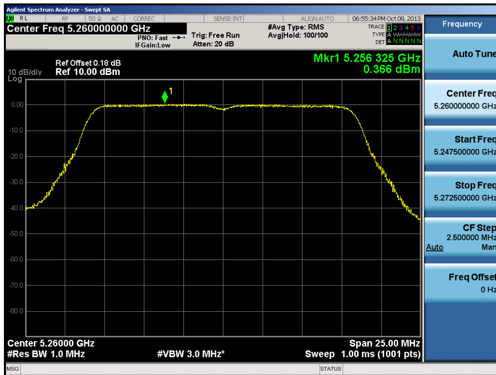
Plot 6-50. Peak Power Spectral Density Plot (802.11a (UNII Band 2) – Ch. 52)
