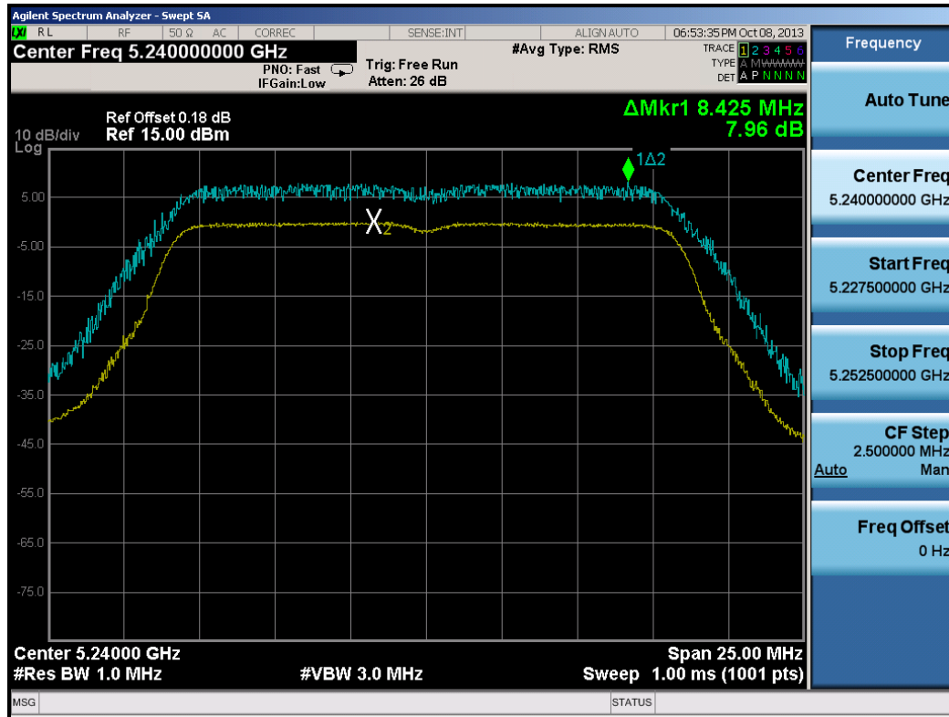
Plot 6-79. Peak Excursion Ratio Plot (802.11a)
