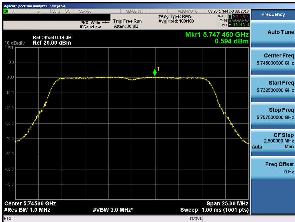
Plot 6-70. Peak Power Spectral Density Plot (20MHz BW 802.11a (UNII Band 4) – Ch. 149)
