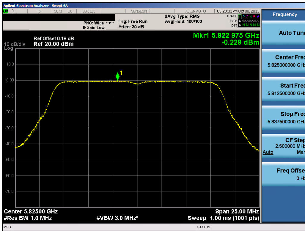
Plot 6-72. Peak Power Spectral Density Plot (20MHz BW 802.11a (UNII Band 4) – Ch. 165)
