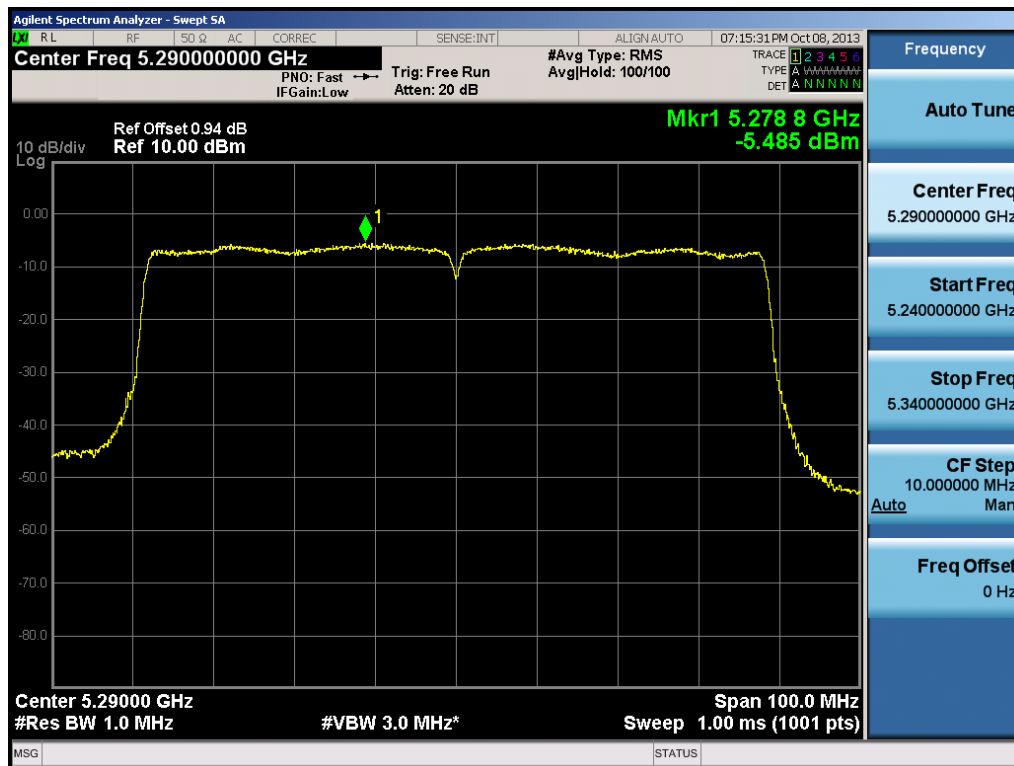
Plot 6-58. Peak Power Spectral Density Plot (80MHz BW 802.11ac (UNII Band 2) – Ch. 58)
