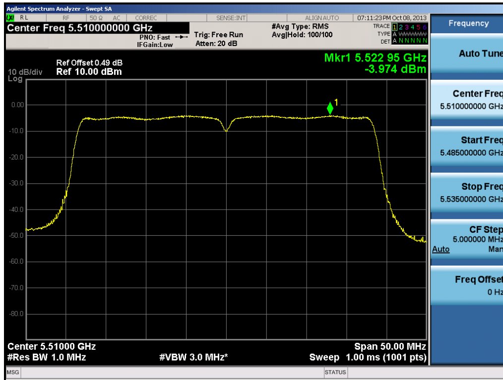
Plot 6-65. Peak Power Spectral Density Plot (40MHz BW 802.11n (UNII Band 3) – Ch. 102)
