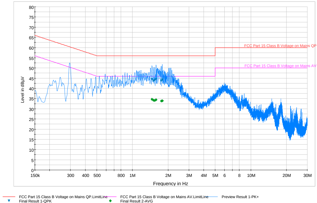
Plot 6-104. Line Conducted Plot with 802.11a UNII Band 1 (N)
