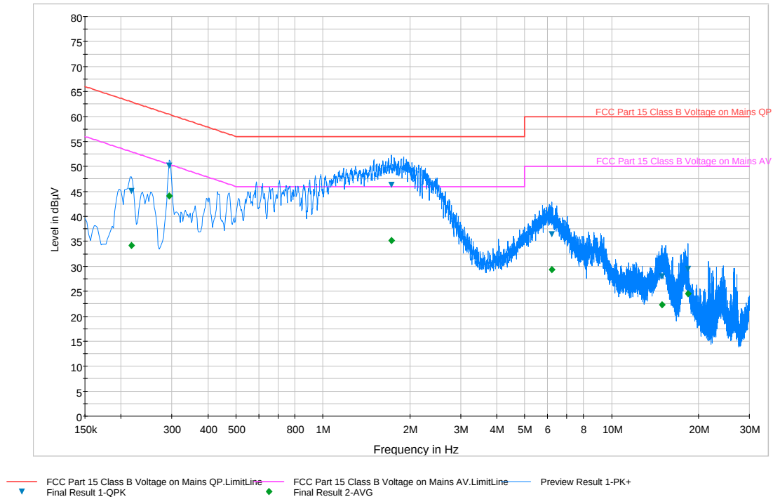
Plot 6-103. Line Conducted Plot with 802.11a UNII Band 1 (L1)
