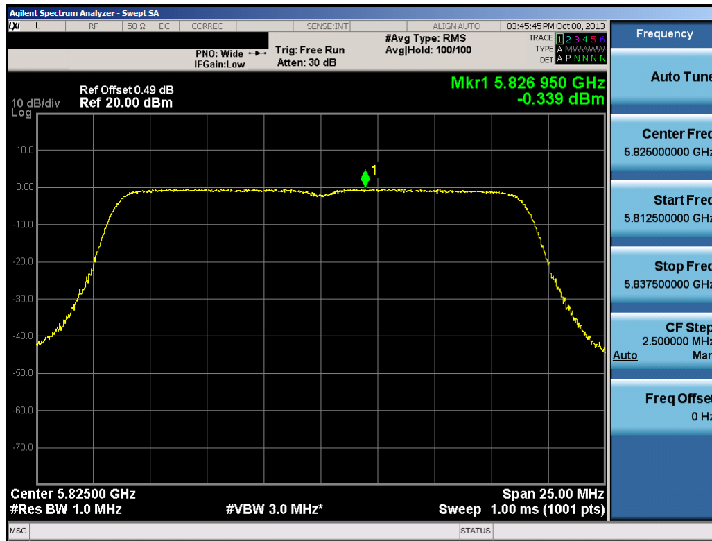
Plot 6-75. Peak Power Spectral Density Plot (20MHz BW 802.11n (UNII Band 4) – Ch. 165)
