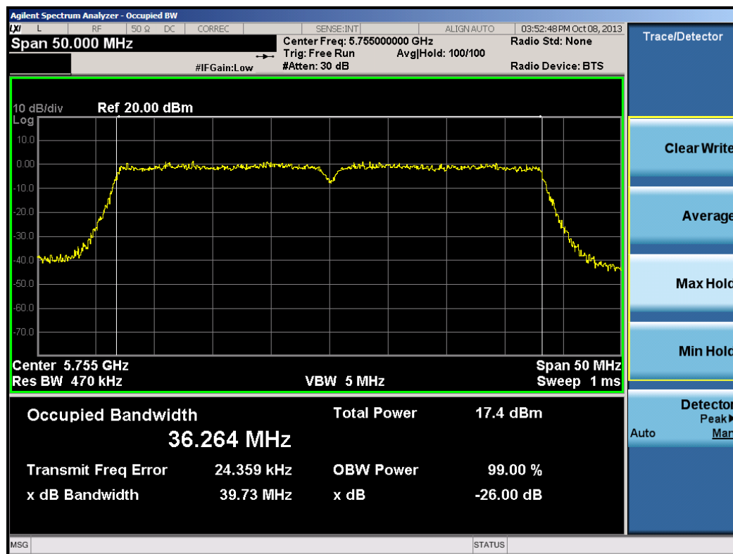
Plot 6-36. 26dB Bandwidth Plot (40MHz BW 802.11n (UNII Band 4) – Ch. 151)
