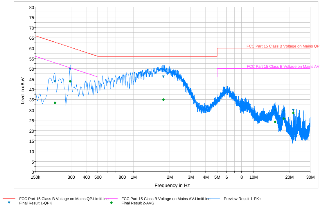
Plot 6-105. Line Conducted Plot with 802.11a UNII Band 2 (L1)
