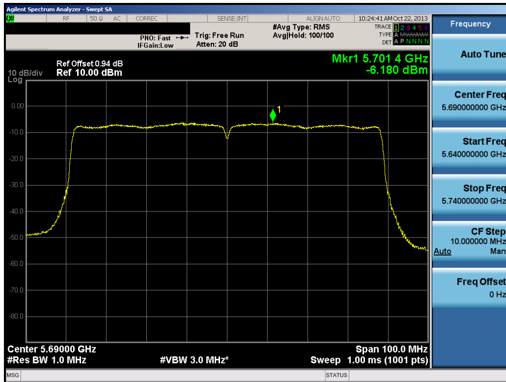
Plot 6-69. Peak Power Spectral Density Plot (80MHz BW 802.11ac (UNII Band 3) – Ch. 138)
