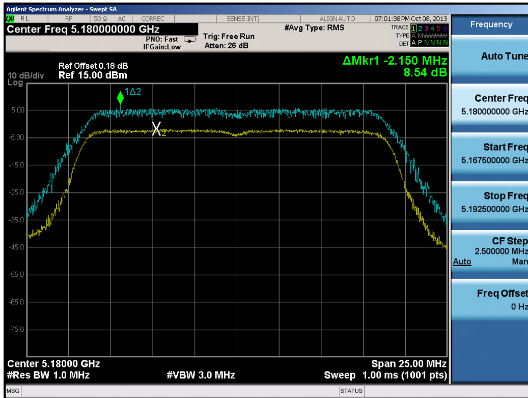
Plot 6-80. Peak Excursion Ratio Plot (20MHz BW 802.11n)
