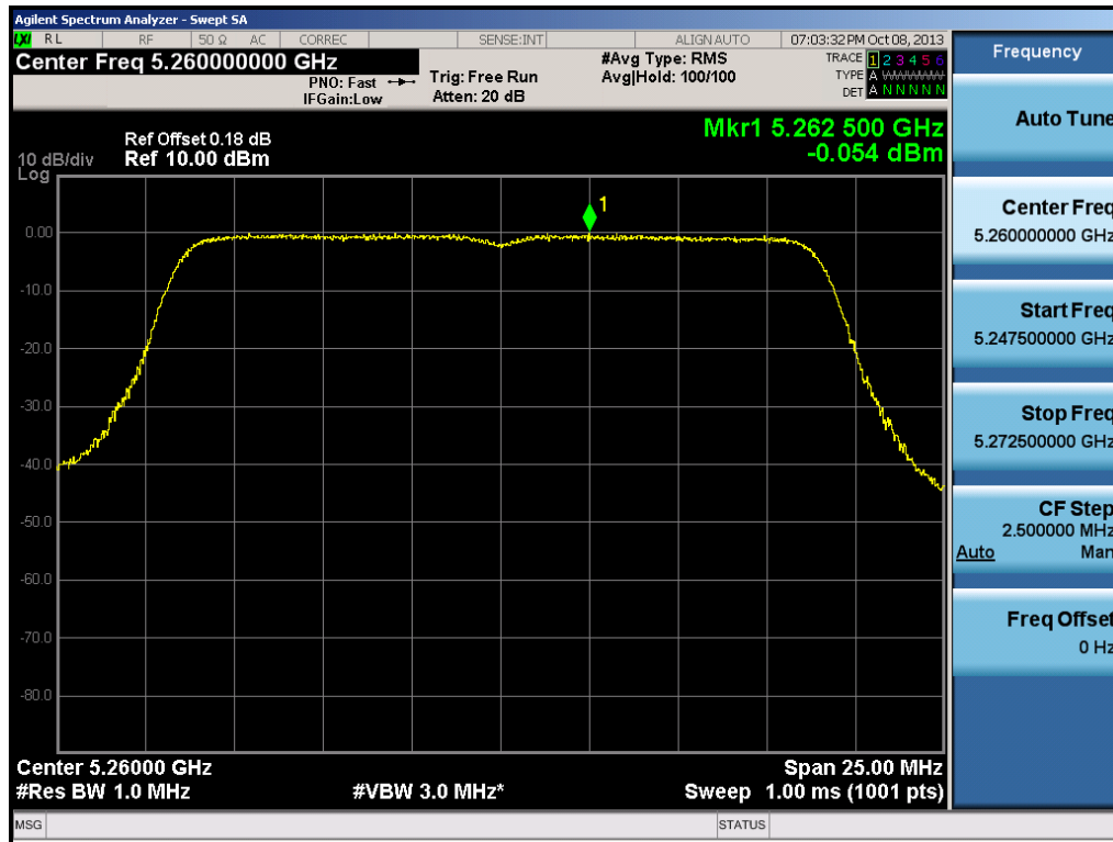
Plot 6-53. Peak Power Spectral Density Plot (20MHz BW 802.11n (UNII Band 2) – Ch. 52)
