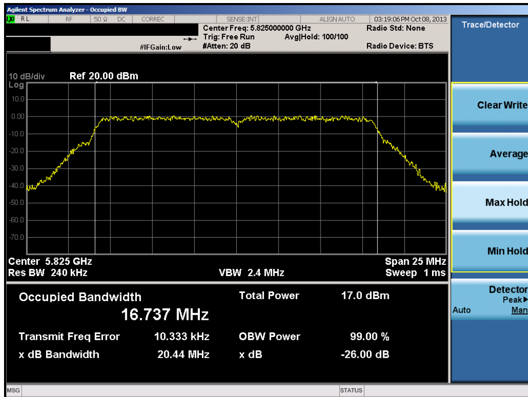
Plot 6-32. 26dB Bandwidth Plot (20MHz BW 802.11a (UNII Band 4) – Ch. 165)
