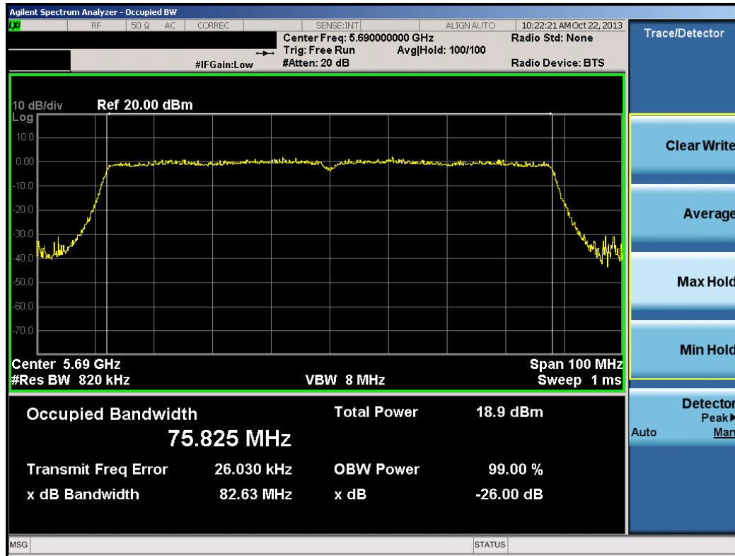
Plot 6-29. 26dB Bandwidth Plot (80MHz BW 802.11ac (UNII Band 3) – Ch. 138)
