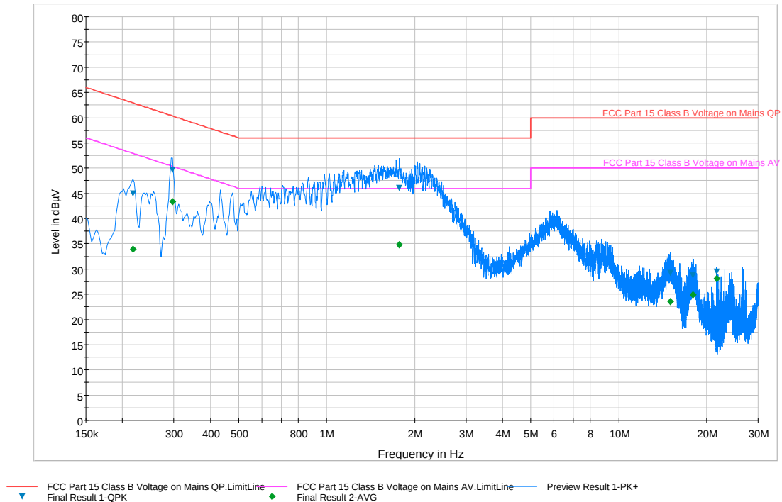
Plot 6-107. Line Conducted Plot with 802.11a UNII Band 3 (L1)
