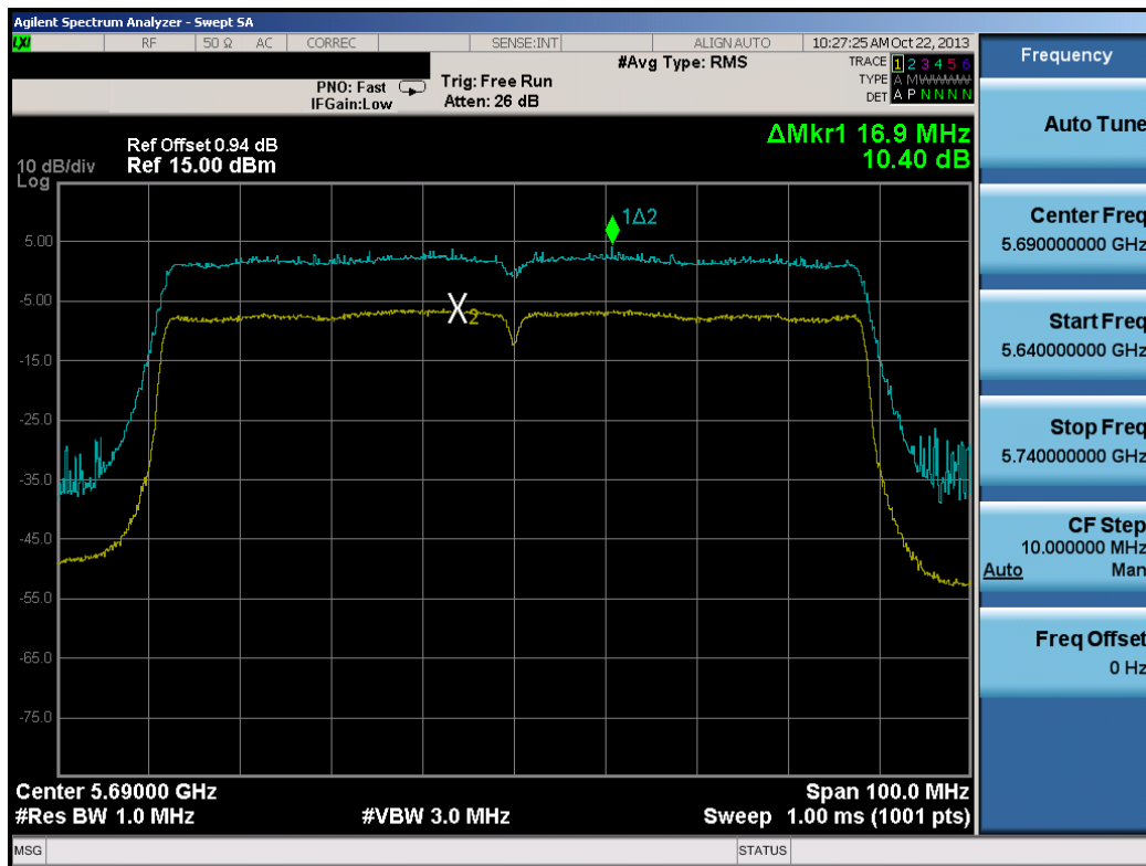
Plot 6-82. Peak Excursion Ratio Plot (80MHz BW 802.11ac)
