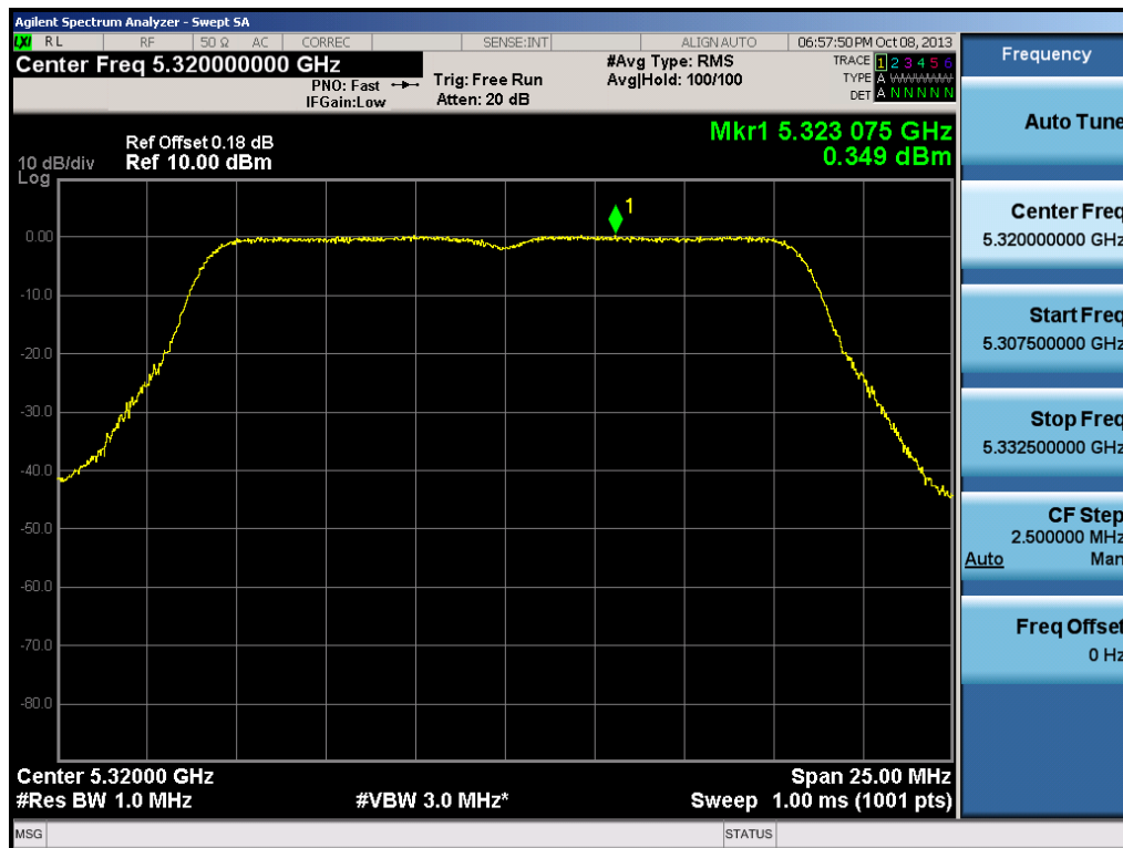
Plot 6-52. Peak Power Spectral Density Plot (802.11a (UNII Band 2) – Ch. 64)
