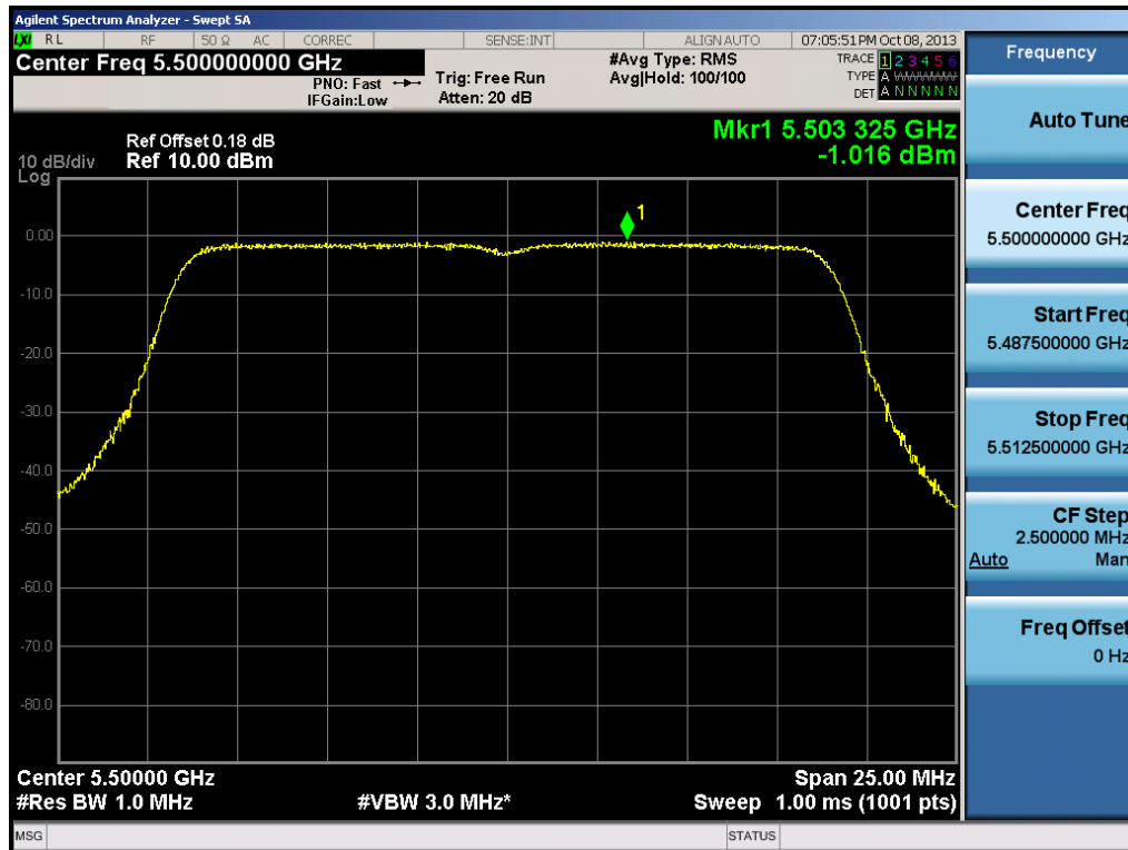
Plot 6-62. Peak Power Spectral Density Plot (20MHz BW 802.11n (UNII Band 3) – Ch. 100)
