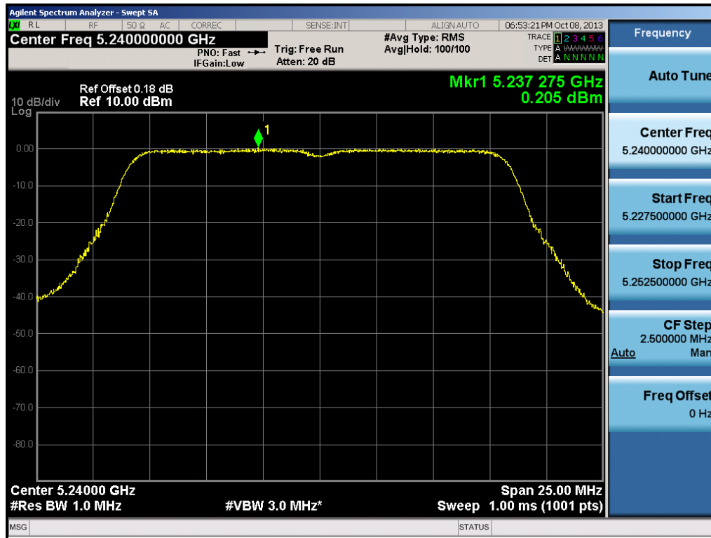
Plot 6-43. Peak Power Spectral Density Plot (802.11a (UNII Band 1) – Ch. 48)
