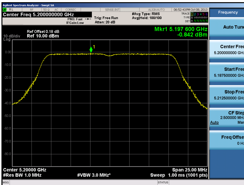
Plot 6-42. Peak Power Spectral Density Plot (802.11a (UNII Band 1) – Ch. 40)
