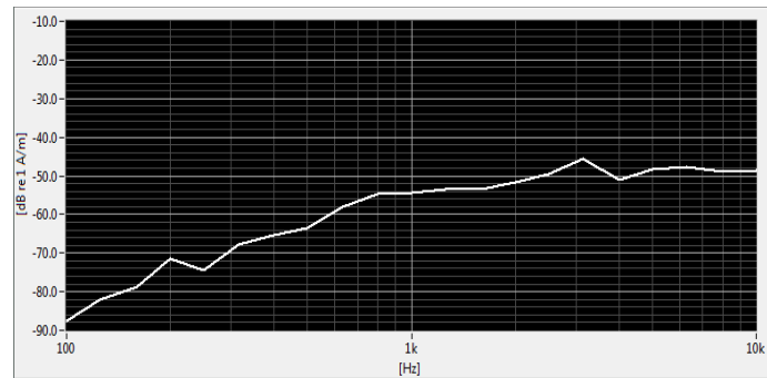
Figure 7-3 Worst-case ABM2 Plot for UMTS
