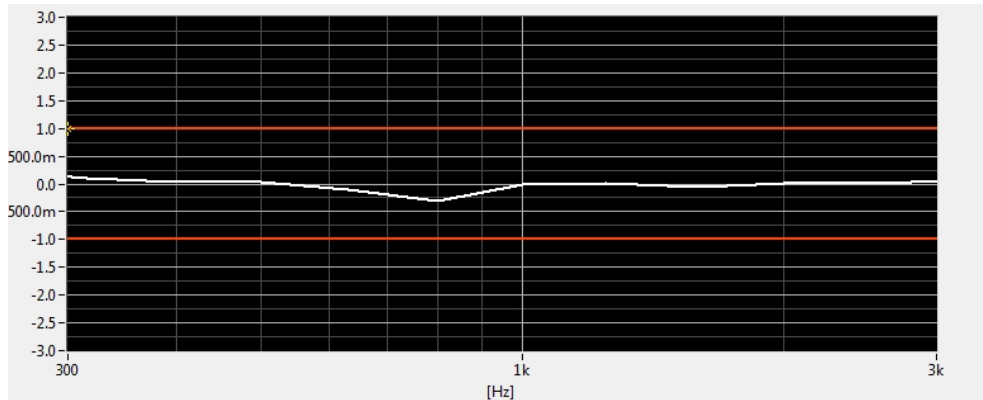
Figure 7-4 Helmholtz Coil Validation for Frequency Response
