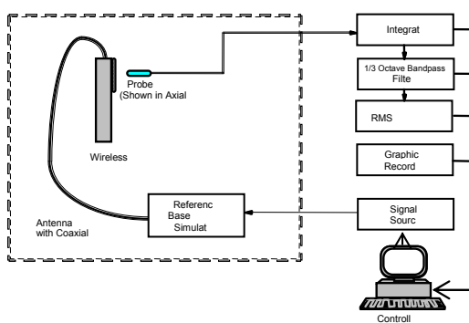
Figure 5-14 Audio Magnetic Field Test Setup
