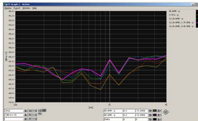
Figure 6-2 UMTS Audio Band Magnetic Noise
