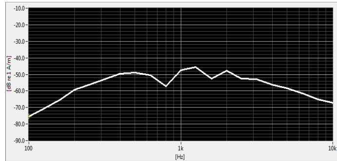
Figure 7-2 Worst-case ABM2 Plot for CDMA
