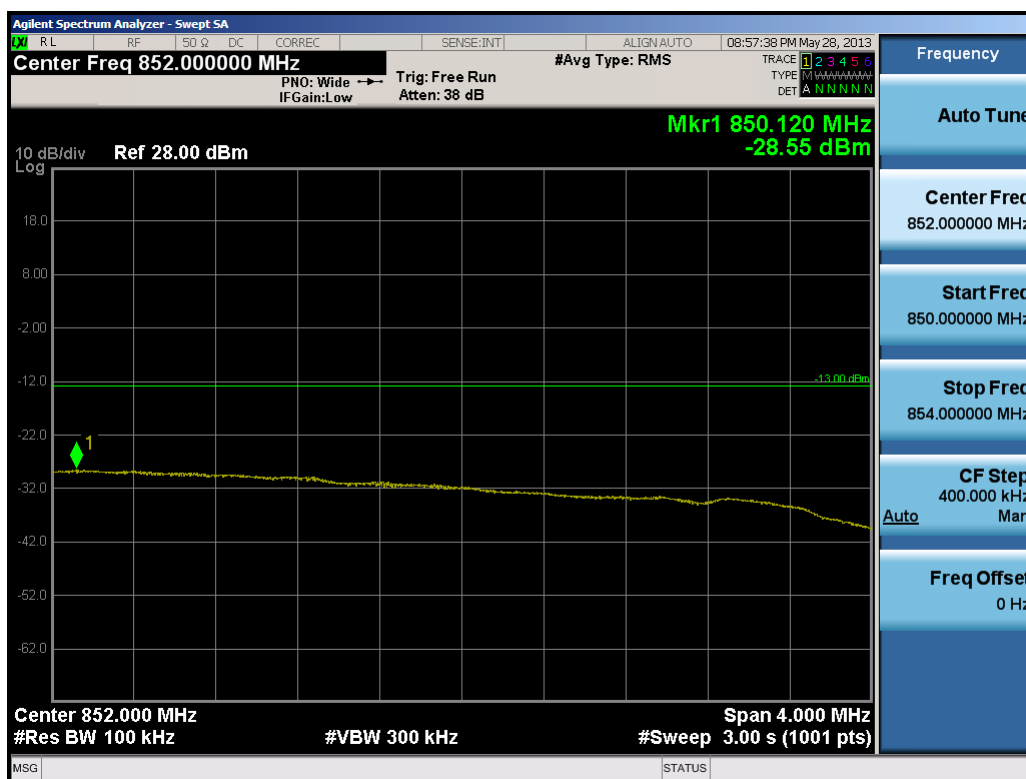
Plot 7-30. Upper Extended Band Edge Plot (10.0MHz QPSK – RB Size 50)
