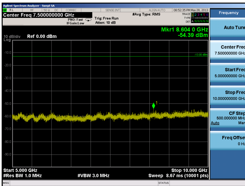
Plot 7-18. Conducted Spurious Plot (5.0MHz QPSK – RB Size 1, RB Offset 0 – Low Channel)
