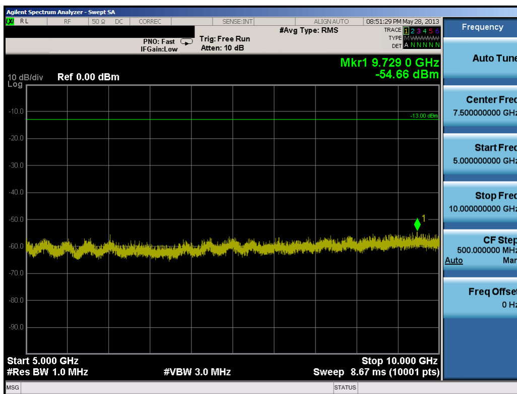
Plot 7-20. Conducted Spurious Plot (5.0MHz QPSK – RB Size 1, RB Offset 0 – Mid Channel)
