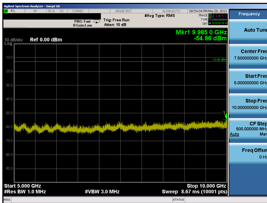
Plot 7-22. Conducted Spurious Plot (5.0MHz QPSK – RB Size 1, RB Offset 0 – High Channel)
