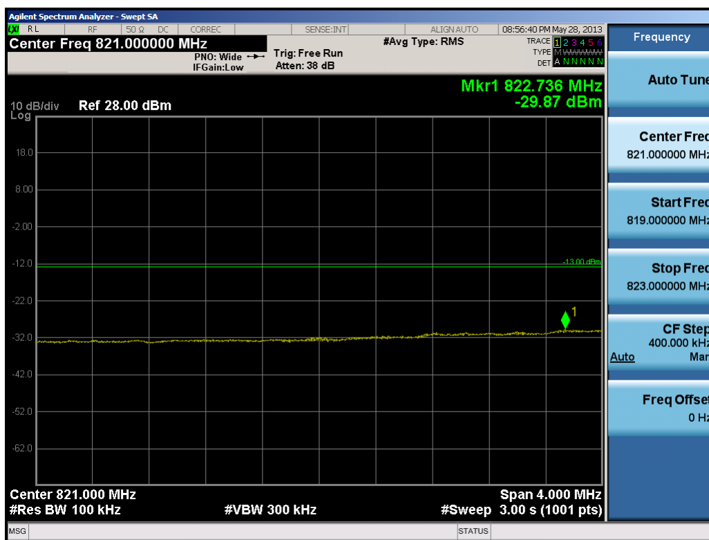
Plot 7-26. Lower Extended Band Edge Plot (10.0MHz QPSK – RB Size 50)
