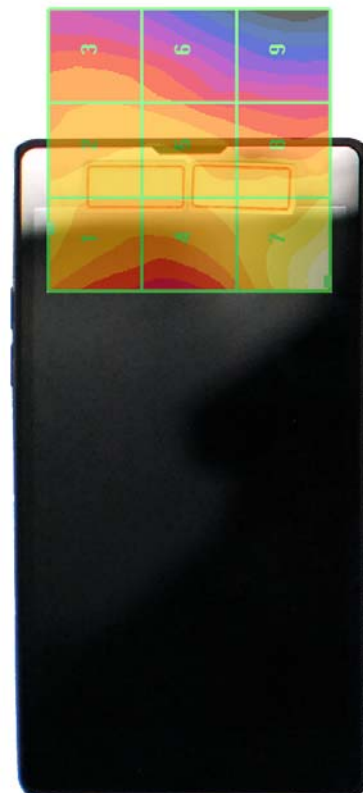
Figure 17-5 H-Field WD Scan overlay
