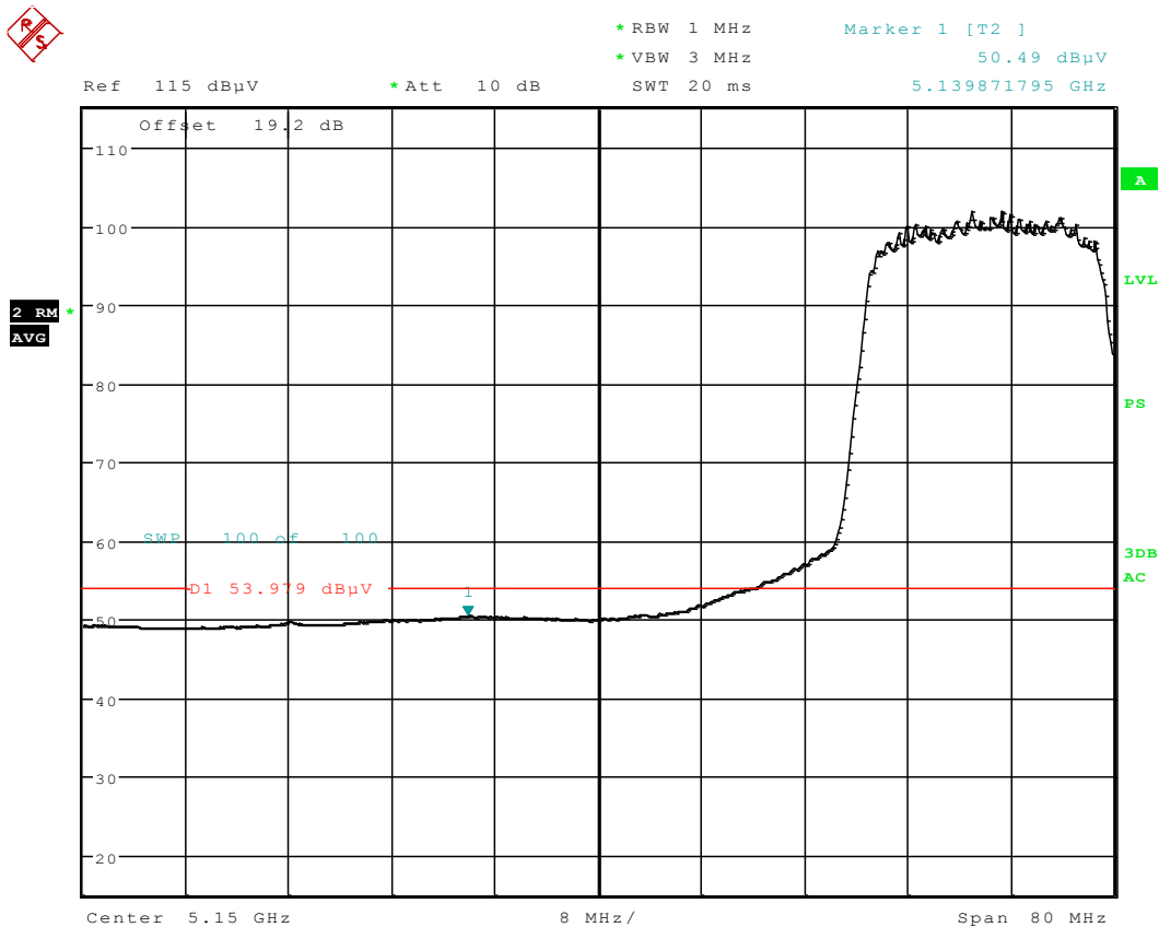
Plot 6-1. Radiated Restricted Lower Band Edge Plot (Average – UNII Band 1)
