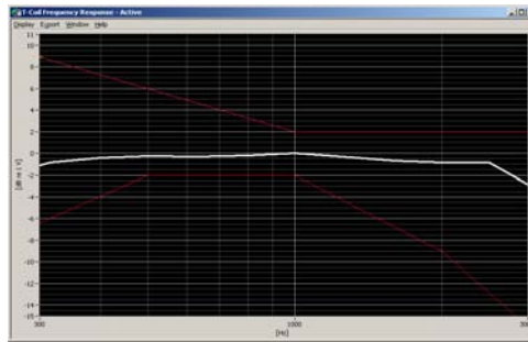
Figure 6-1 Axial Frequency Response
