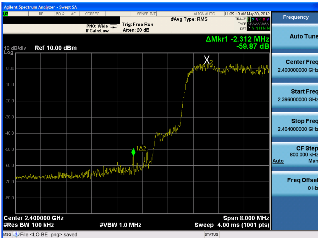
Plot 6-12. Band Edge Plot (Bluetooth with Hopping Enabled, 3Mbps)
