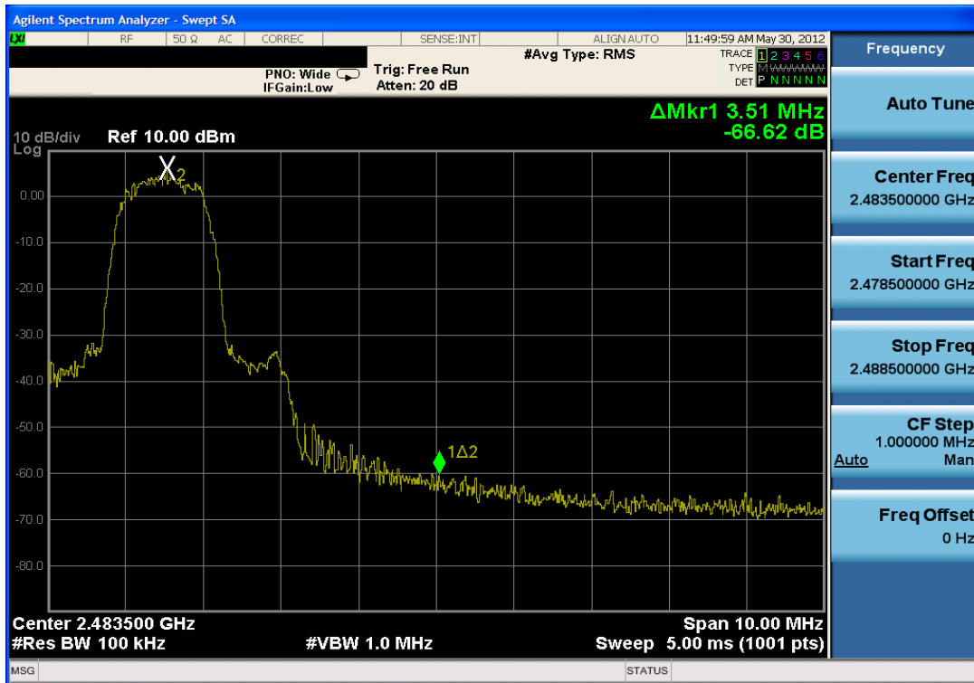
Plot 6-11. Band Edge Plot (Bluetooth with Hopping Disabled, 3Mbps – Ch. 78)
