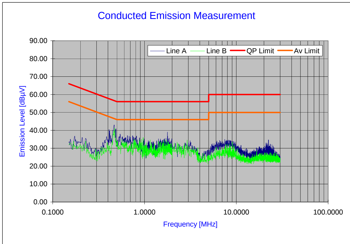
Plot 6-24. Line Conducted Plot with Bluetooth
