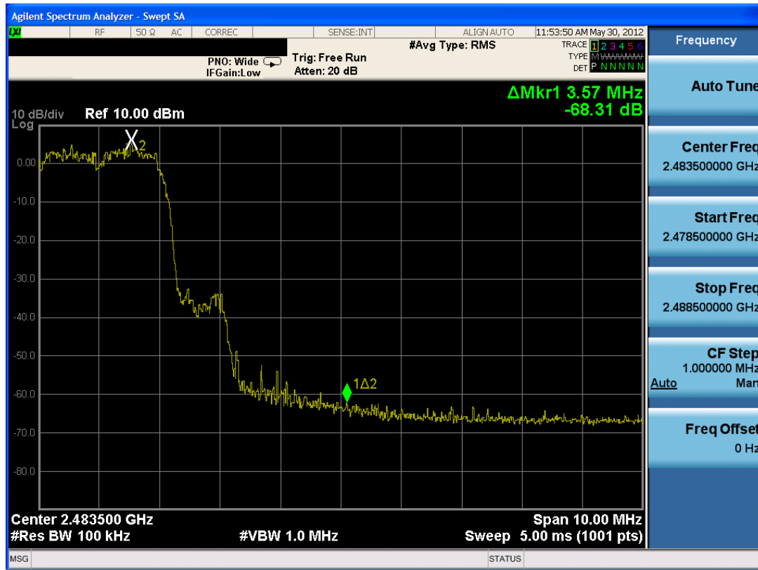
Plot 6-13. Band Edge Plot (Bluetooth with Hopping Enabled, 3Mbps)
