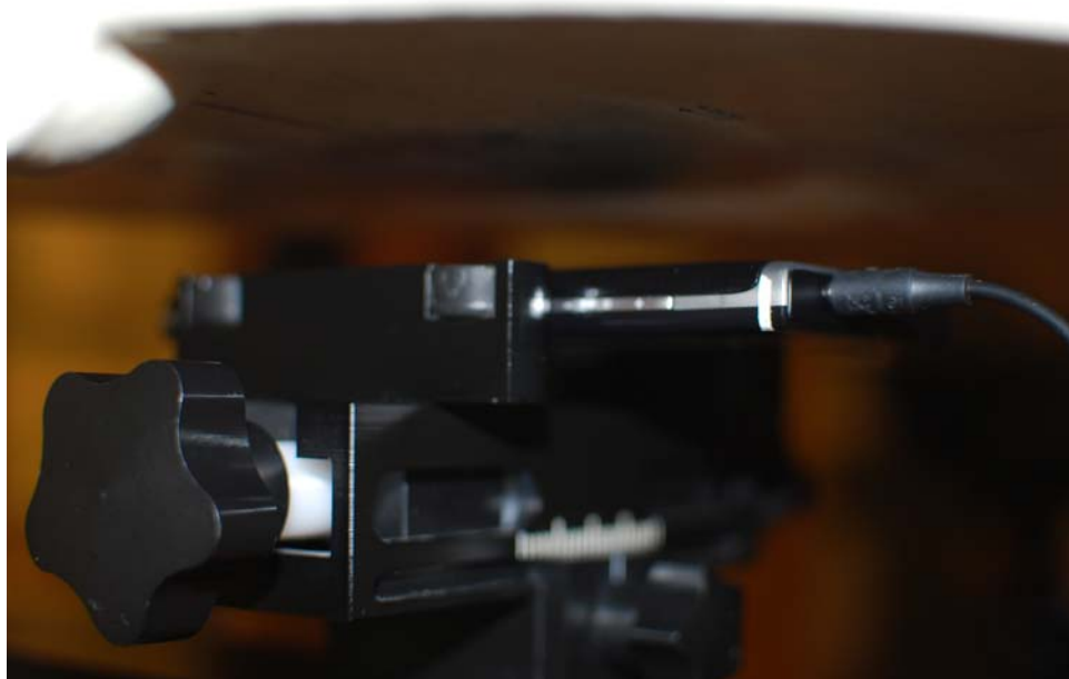
SAR Test Setup Photo 5 – Body-Worn Back at 2.0 cm
