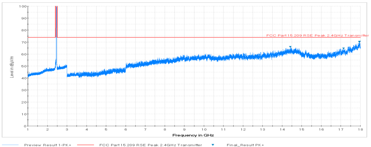
Plot 7-36. Radiated Spurious Plot above 1GHz (802.11b – Ch. 11, Ant. Pol. V)
