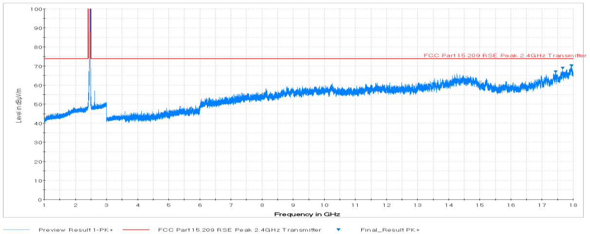
Plot 7-35. Radiated Spurious Plot above 1GHz (802.11b – Ch. 11, Ant. Pol. H)
