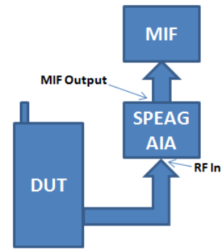
Figure 7-2 MIF Measurement Setup for unlicensed modes
