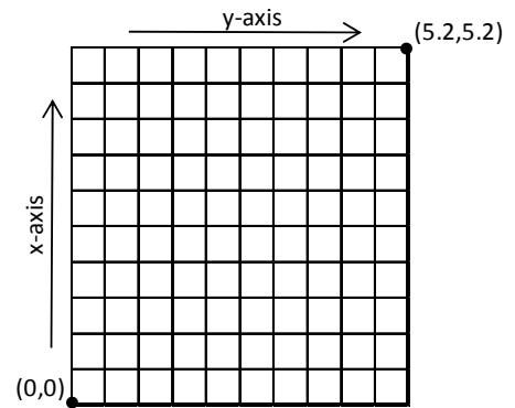
Figure 4-12 Measurement Grid
