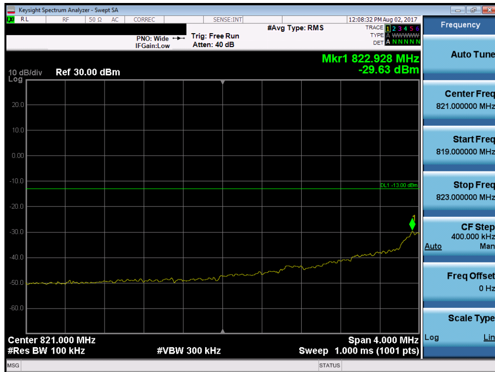
Plot 7-22. 4MHz Span Plot (Cellular CDMA Mode – Ch. 1013)
