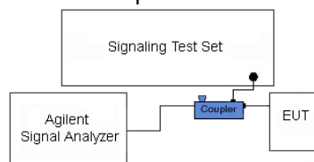
Figure 7-3. Test Instrument & Measurement Setup
